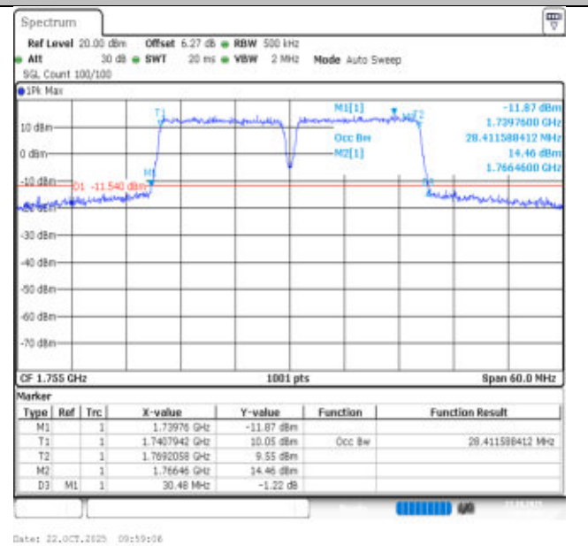
66-66-15MHz-15MHz-16QAM-16QAM-132347-132497-75RB#0-75RB#0-PASS
