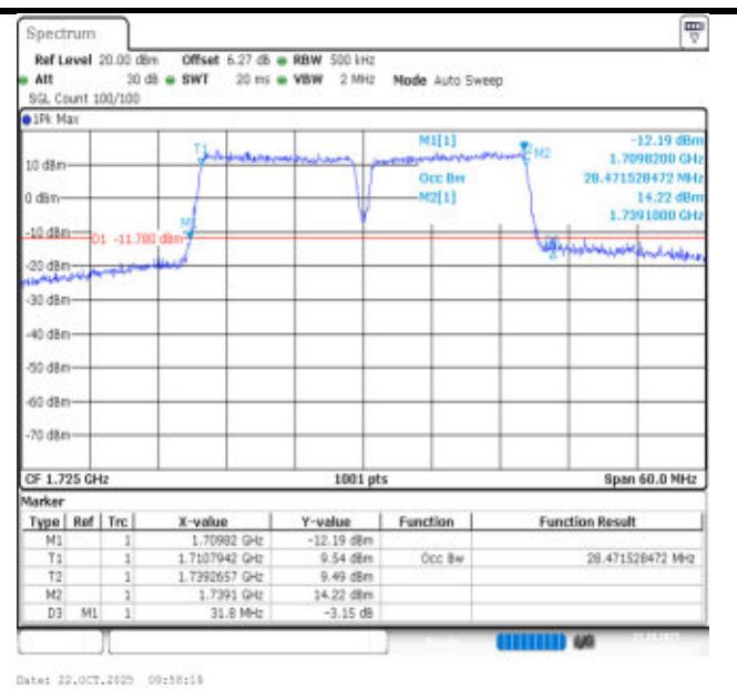
66-66-15MHz-15MHz-16QAM-16QAM-132047-132197-75RB#0-75RB#0-PASS
