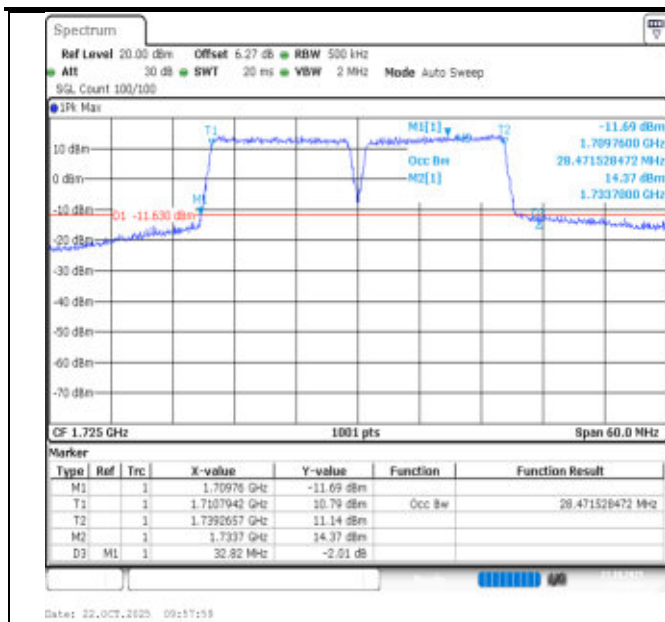
66-66-15MHz-15MHz-QPSK-QPSK-132047-132197-75RB#0-75RB#0-PASS
