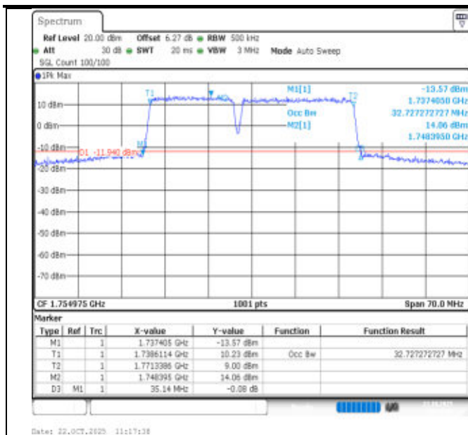
66-66-15MHz-20MHz-QPSK-QPSK-132325-132496-75RB#0-100RB#0-PASS
