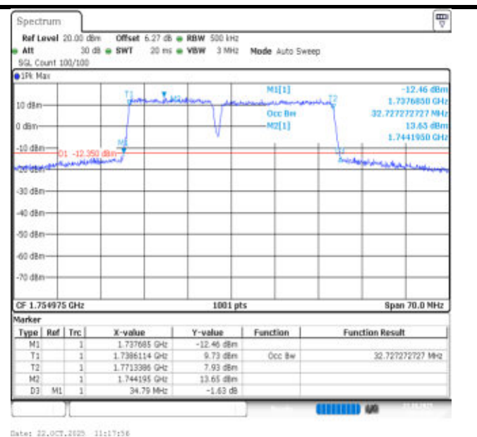
66-66-15MHz-20MHz-16QAM-16QAM-132325-132496-75RB#0-100RB#0-PASS
