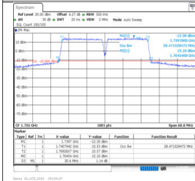
66-66-15MHz-15MHz-QPSK-QPSK-132347-132497-75RB#0-75RB#0-PASS
