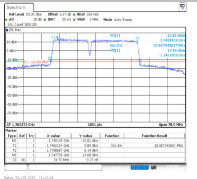
66-66-15MHz-20MHz-16QAM-16QAM-132401-132572-75RB#0-100RB#0-PASS
