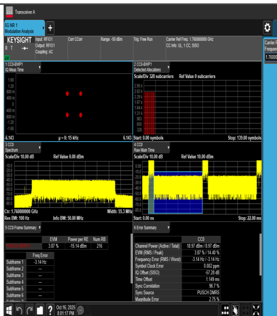
NTVN-n66-PC3-15-40-H-CP-QPSK-Outer_Full-PASS
