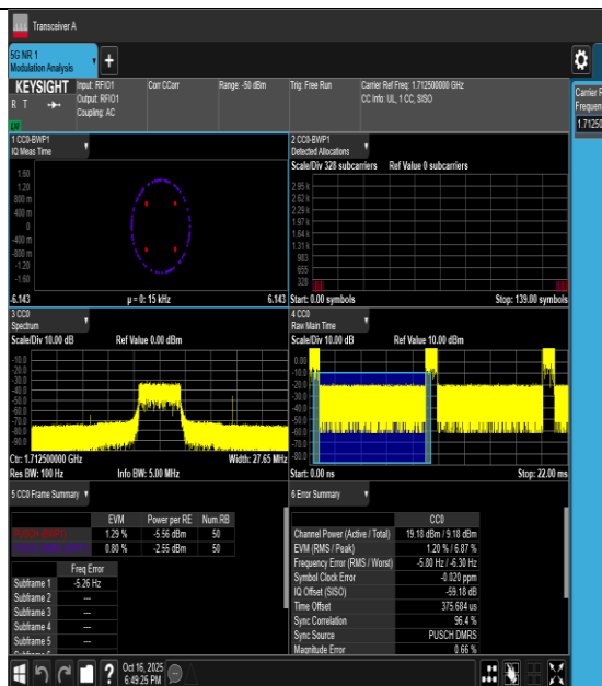
50NV-n66-PC3-15-5-L-DFT-QPSK-Outer_Full-PASS
