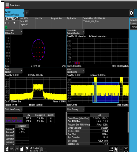
30NV-n66-PC3-15-5-L-DFT-16QAM-Outer_Full-PASS
