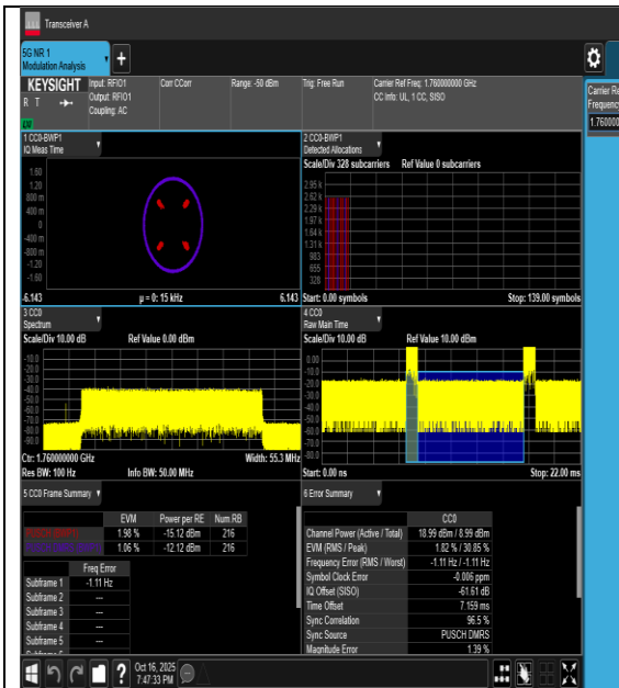
NTVH-n66-PC3-15-40-H-DFT-QPSK-Outer_Full-PASS
