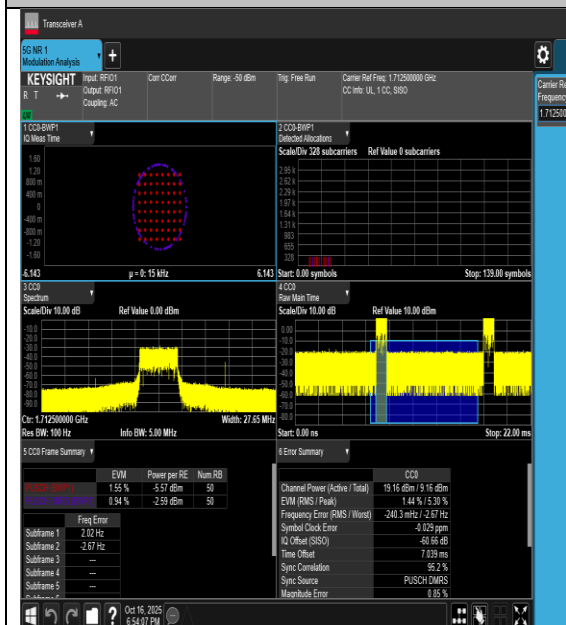
20NV-n66-PC3-15-5-L-DFT-64QAM-Outer_Full-PASS
