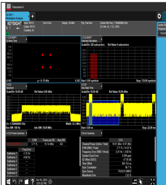
NTVL-n66-PC3-15-40-H-CP-QPSK-Outer_Full-PASS
