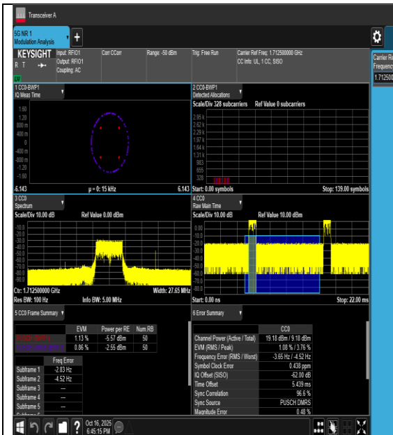
30NV-n66-PC3-15-5-L-DFT-BPSK-Outet_Full-PASS
