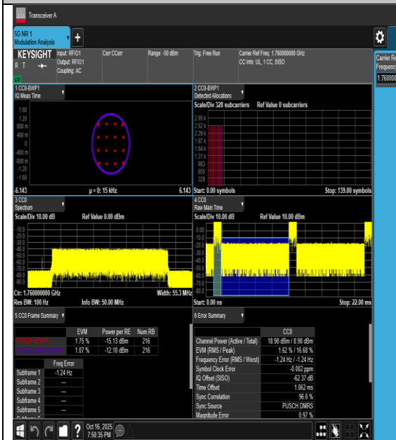
NTVN-n66-PC3-15-40-H-DFT-16QAM-Outer_Full-PASS
