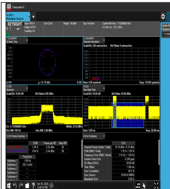
40NV-n66-PC3-15-5-L-DFT-QPSK-Outer_Full-PASS
