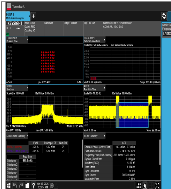
NTVN-n66-PC3-15-5-L-CP-64QAM-Outter_Full-PASS
