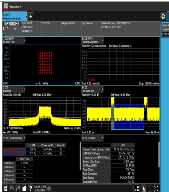
NTVH-n66-PC3-15-5-L-CP-64QAM-Outter_Full-PASS
