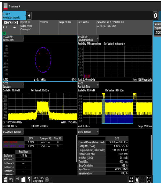
40NV-n66-PC3-15-5-L-DFT-BPSK-Outet_Full-PASS
