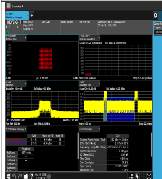
NTVL-n66-PC3-15-5-L-CP-256QAM-Outter_Full-PASS
