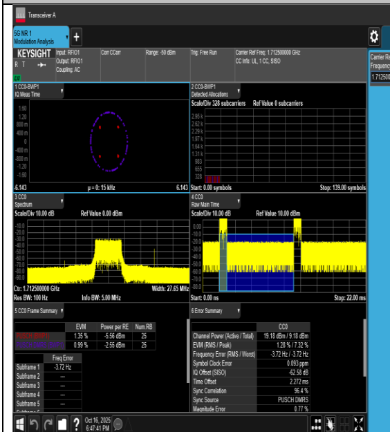
30NV-n66-PC3-15-5-L-DFT-QPSK-Outet_Full-PASS
