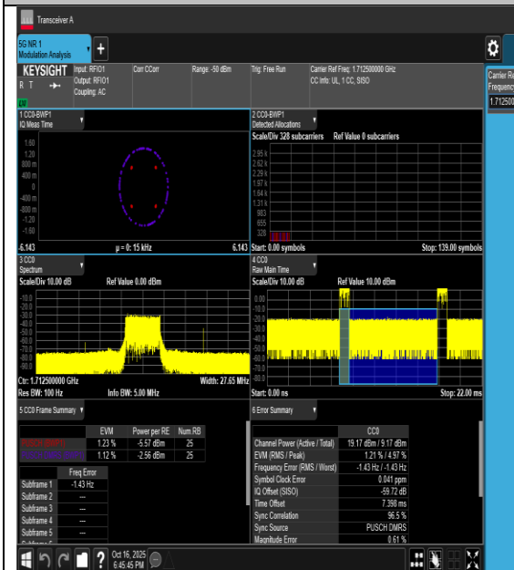
50NV-n66-PC3-15-5-L-DFT-BPSK-Outet_Full-PASS
