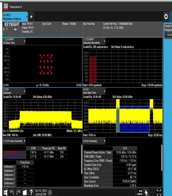
NTVL-n66-PC3-15-40-H-CP-16QAM-Outer_Full-PASS
