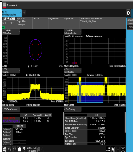
30NV-n66-PC3-15-5-L-DFT-QPSK-Outet_Full-PASS
