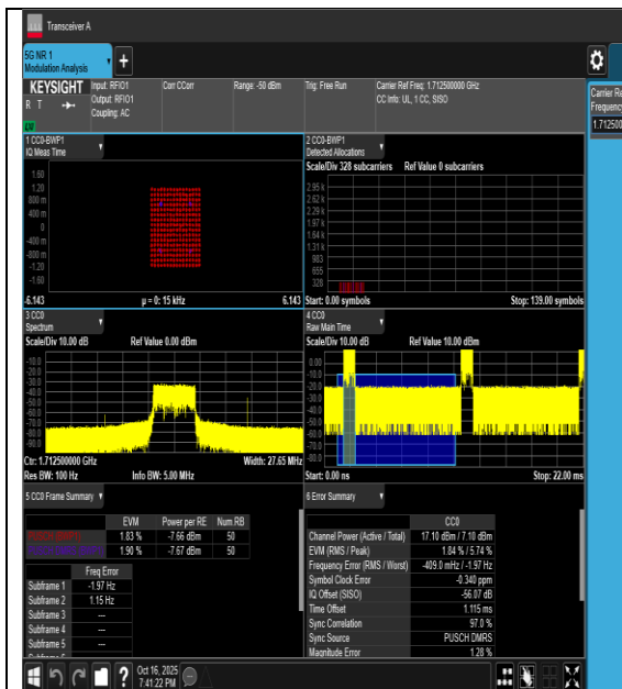
20NV-n66-PC3-15-5-L-CP-256QAM-Outer_Full-PASS
