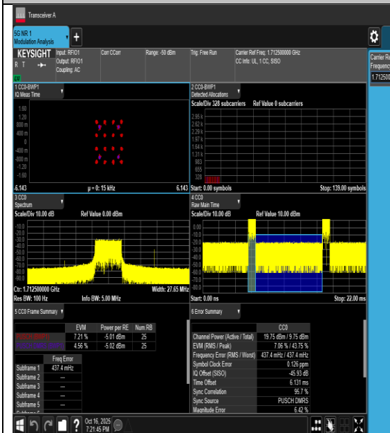
20NV-n66-PC3-15-5-L-CP-16QAM-Outer_Full-PASS
