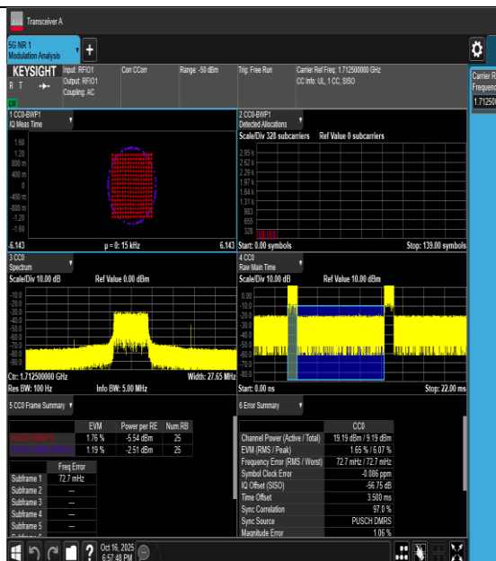
20NV-n66-PC3-15-5-L-DFT-256QAM-Outer_Full-PASS
