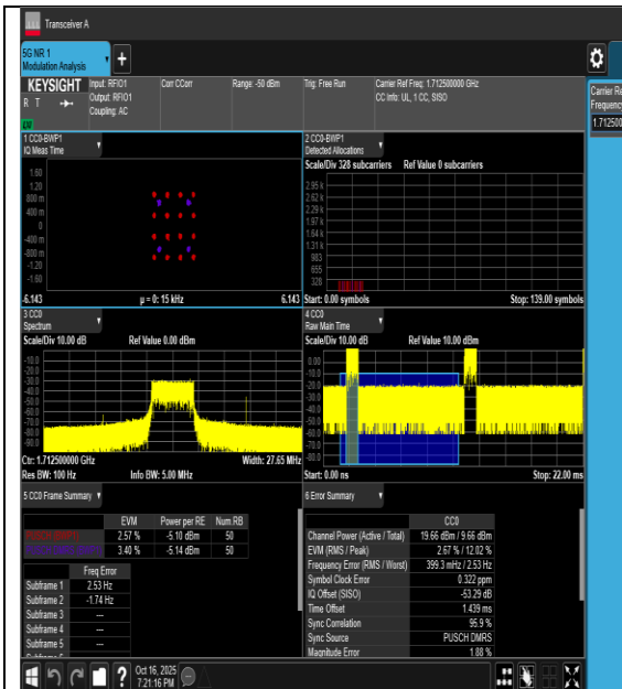
0NV-n66-PC3-15-5-L-CP-16QAM-Outer_Full-PASS
