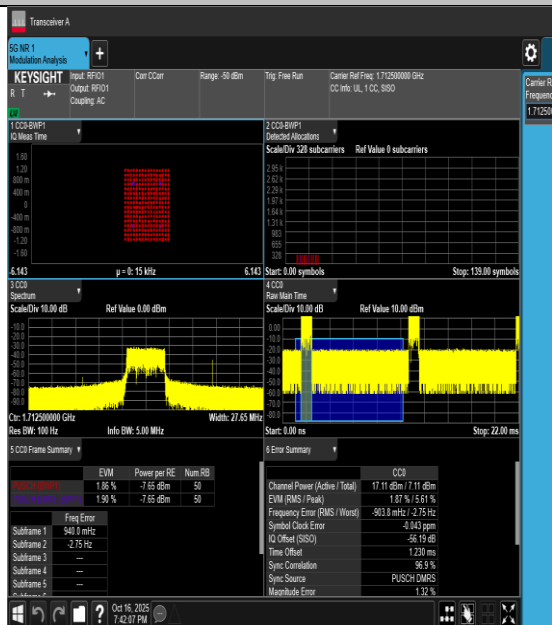
50NV-n66-PC3-15-5-L-CP-256QAM-Outer_Full-PASS
