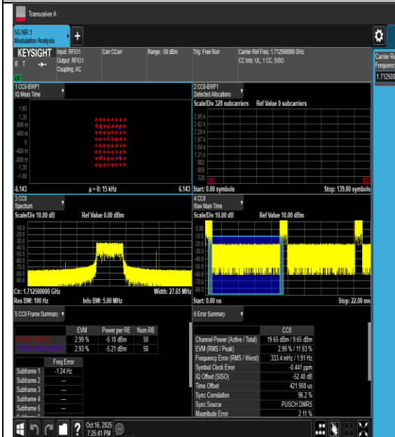
50NV-n66-PC3-15-5-L-CP-64QAM-Outer_Full-PASS
