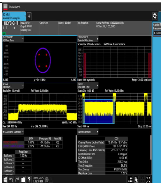
40NV-n66-PC3-15-40-H-DFT-BPSK-Outter_Full-PASS
