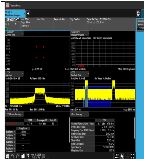
10NV-n66-PC3-15-5-L-CP-QPSK-Outet_Full-PASS
