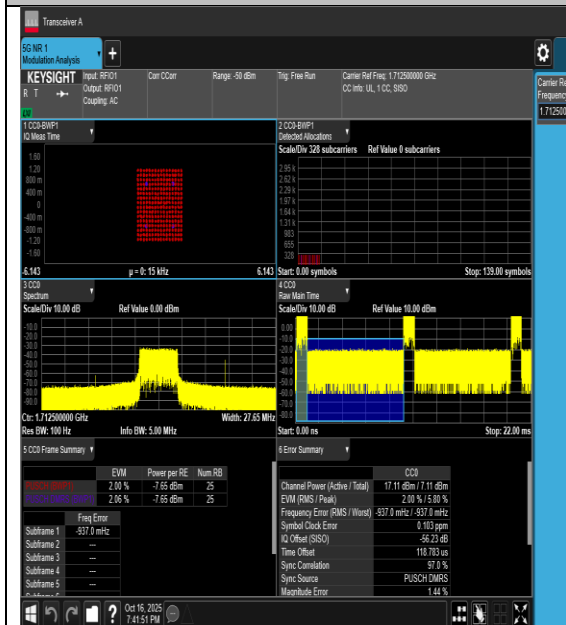
40NV-n66-PC3-15-5-L-CP-256QAM-Outer_Full-PASS
