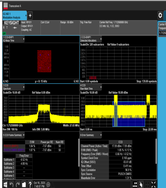
60NV-n66-PC3-15-5-L-CP-64QAM-Outer_Full-PASS
