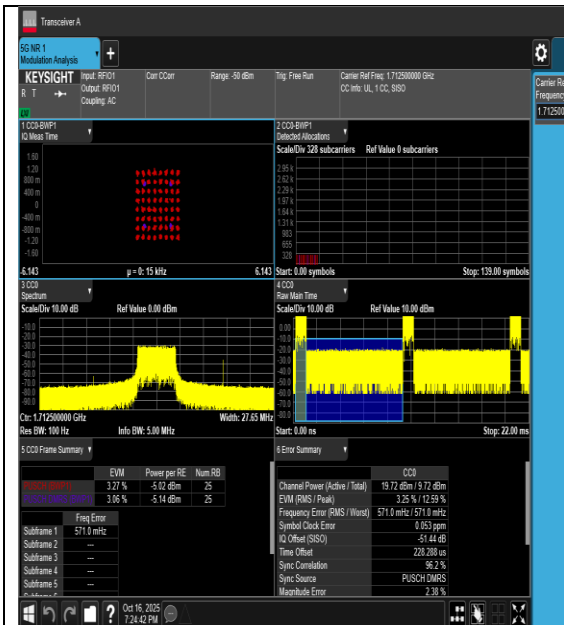
10NV-n66-PC3-15-5-L-CP-64QAM-Outer_Full-PASS
