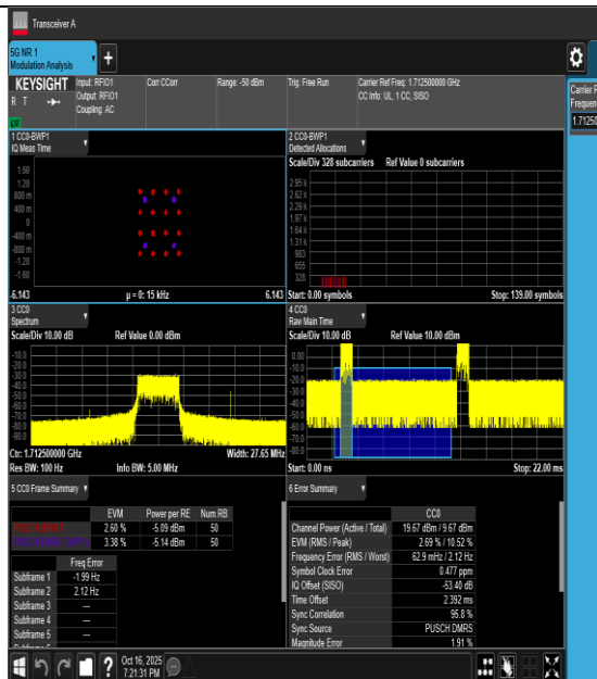
10NV-n66-PC3-15-5-L-CP-16QAM-Outer_Full-PASS
