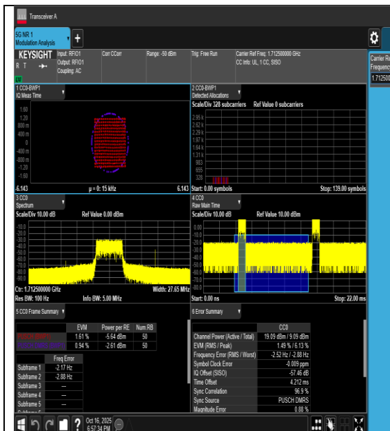
30NV-n66-PC3-15-5-L-DFT-256QAM-Outer_Full-PASS
