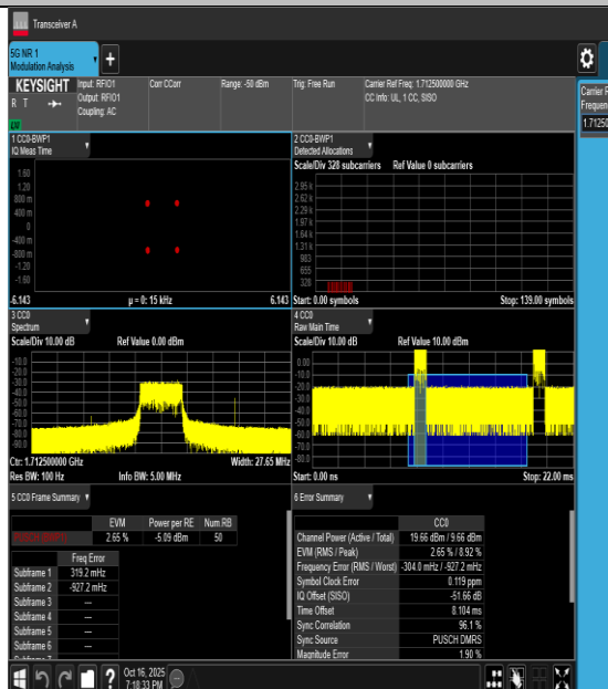
20NV-n66-PC3-15-5-L-CP-QPSK-Outet_Full-PASS
