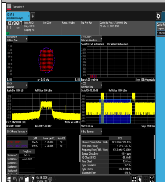
10NV-n66-PC3-15-5-L-DFT-256QAM-Outer_Full-PASS
