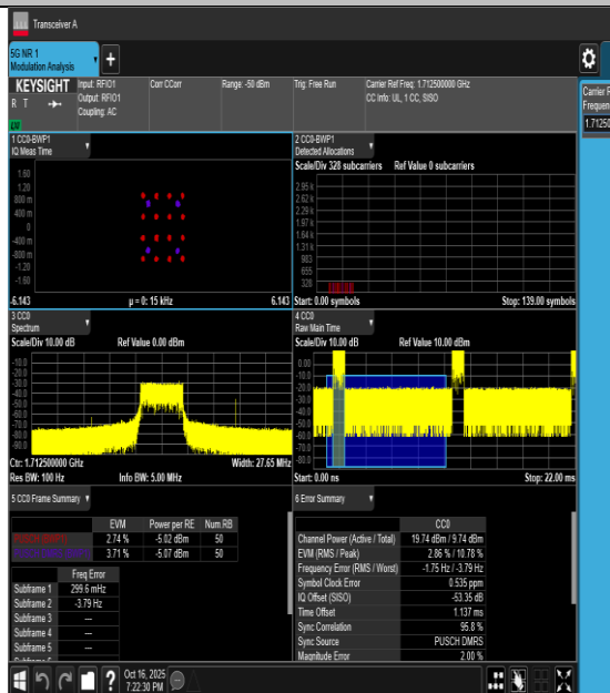
30NV-n66-PC3-15-5-L-CP-16QAM-Outer_Full-PASS
