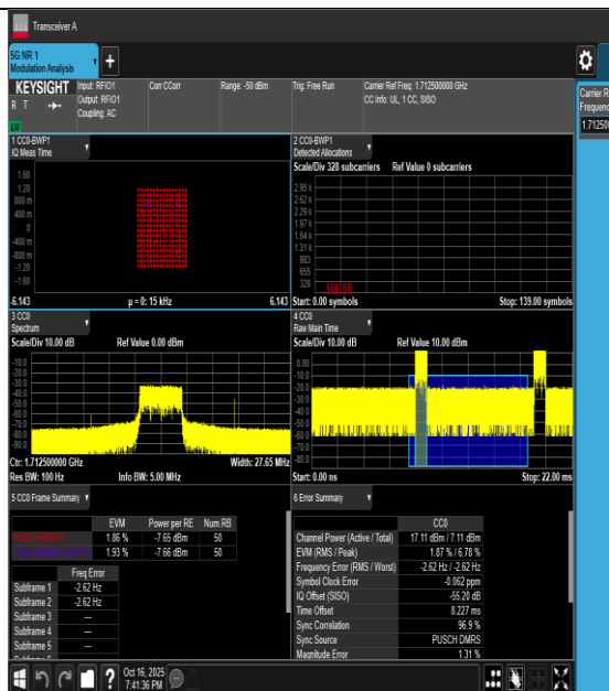
30NV-n66-PC3-15-5-L-CP-256QAM-Outer_Full-PASS
