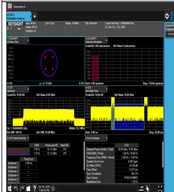
50NV-n66-PC3-15-40-H-DFT-BPSK-Outter_Full-PASS
