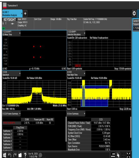
0NV-n66-PC3-15-5-L-CP-QPSK-Outet_Full-PASS
