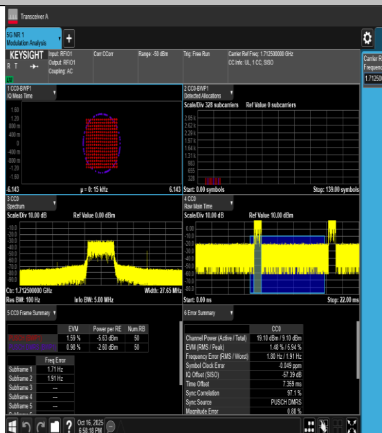
0NV-n66-PC3-15-5-L-DFT-256QAM-Outer_Full-PASS
