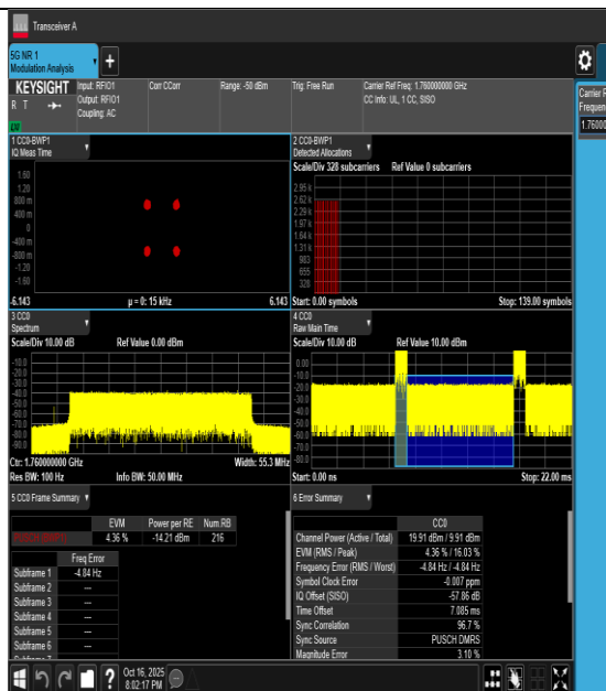
10NV-n66-PC3-15-40-H-CP-QPSK-Outet_Full-PASS
