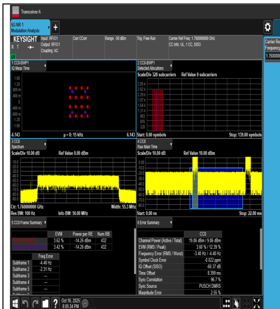
10NV-n66-PC3-15-40-H-CP-16QAM-Outer_Full-PASS
