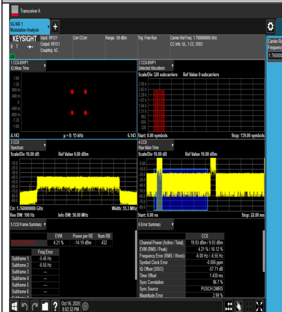
0NV-n66-PC3-15-40-H-CP-QPSK-Outet_Full-PASS
