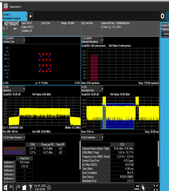
20NV-n66-PC3-15-40-H-CP-16QAM-Outer_Full-PASS
