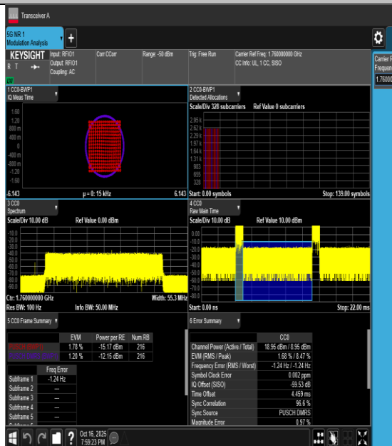
0NV-n66-PC3-15-40-H-DFT-256QAM-Outer_Full-PASS
