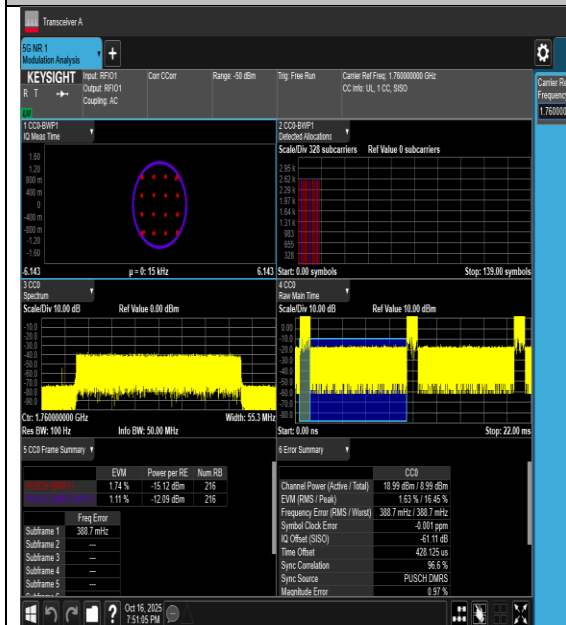
30NV-n66-PC3-15-40-H-DFT-16QAM-Outer_Full-PASS
