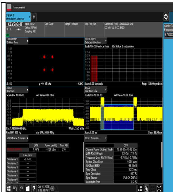
20NV-n66-PC3-15-40-H-CP-QPSK-Outet_Full-PASS
