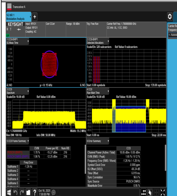
10NV-n66-PC3-15-40-H-DFT-256QAM-Outer_Full-PASS
