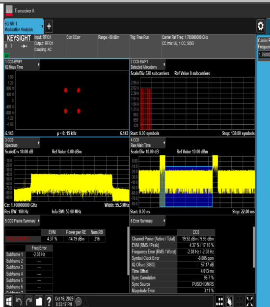
10NV-n66-PC3-15-40-H-CP-QPSK-Outet_Full-PASS
