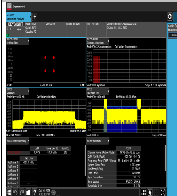
20NV-n66-PC3-15-40-H-CP-QPSK-Outet_Full-PASS
