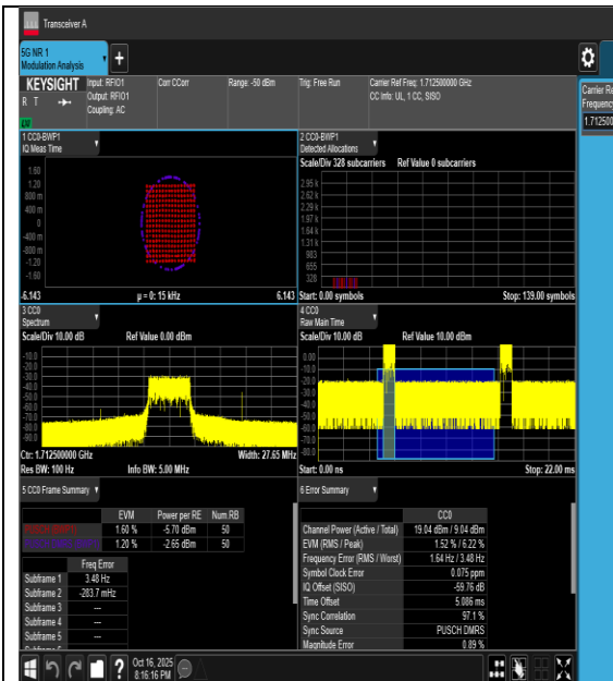
NTNV-n66-PC3-15-5-L-DFT-256QAM-Outer_Full-PASS
