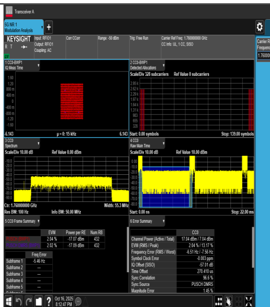
20NV-n66-PC3-15-40-H-CP-256QAM-Outer_Full- PASS
