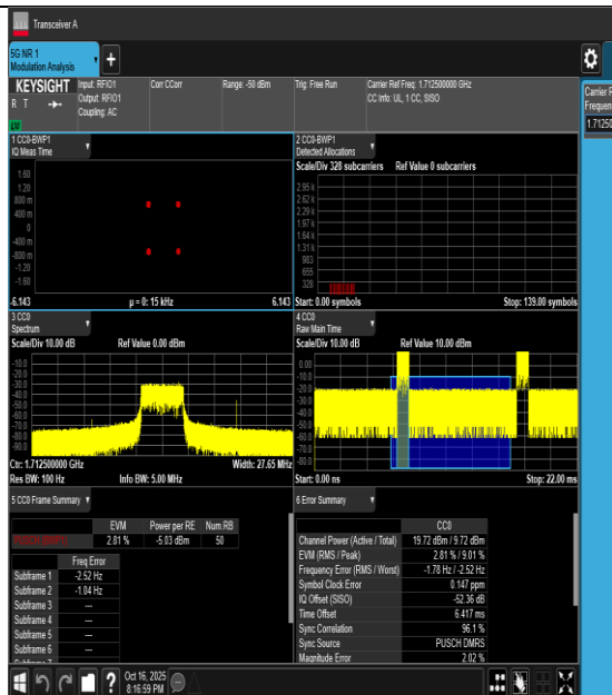
NTNV-n66-PC3-15-5-L-CP-QPSK-Outer_Full-PASS
