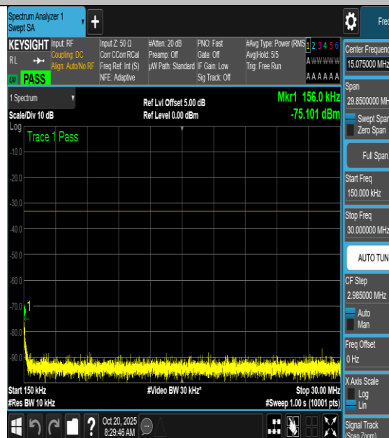
NTNV-n66-PC3-15-5-L-DFT-16QAM- Edge_1RB_Left-0.15-30-PASS
