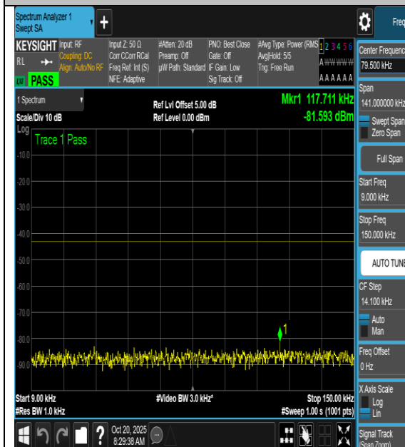
NTNV-n66-PC3-15-5-L-DFT-16QAM- Edge_1RB_Left-0.009-0.15-PASS
