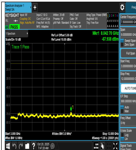
NTNV-n66-PC3-15-5-L-DFT-BPSK-Outter_Full- 3000-12000-PASS
