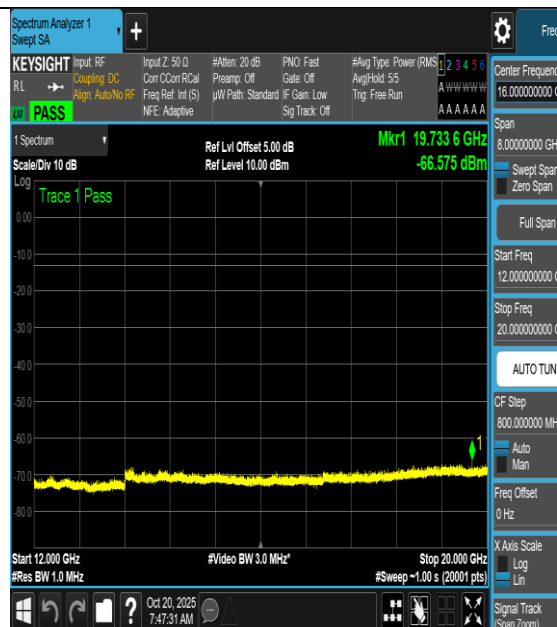
NTNV-n66-PC3-15-5-L-DFT-BPSK-Outter_Full- 12000-20000-PASS
