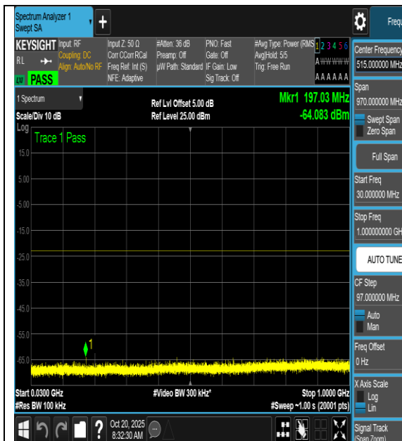
NTNV-n66-PC3-15-5-L-DFT-16QAM- Inner_1RB_Left-30-1000-PASS
