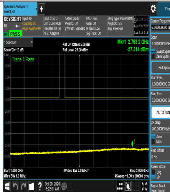
NTNV-n66-PC3-15-5-L-DFT-QPSK- Edge_1RB_Left-0.15-30-PASS
