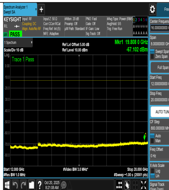
NTNV-n66-PC3-15-5-L-DFT-QPSK-Outter_Full- 12000-20000-PASS
