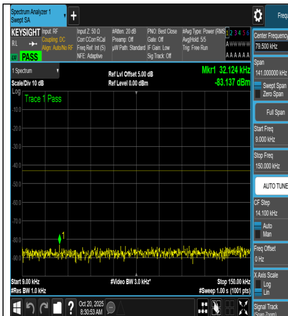
NTNV-n66-PC3-15-5-L-DFT-16QAM- Edge_1RB_Right-0.009-0.15-PASS
