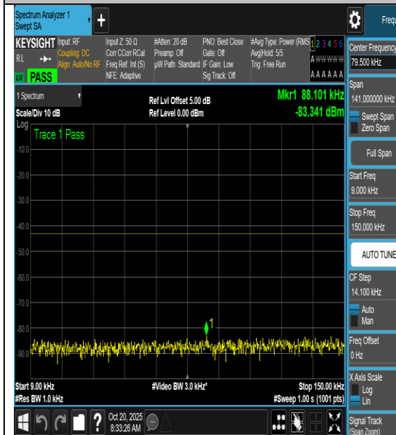
NTNV-n66-PC3-15-5-L-DFT-16QAM- Inner_1RB_Left-3000-12000-PASS
