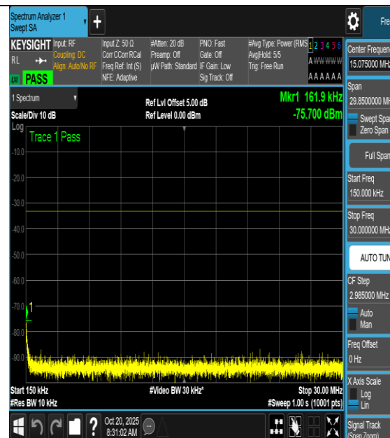
NTNV-n66-PC3-15-5-L-DFT-16QAM- Edge_1RB_Right-0.15-30-PASS
