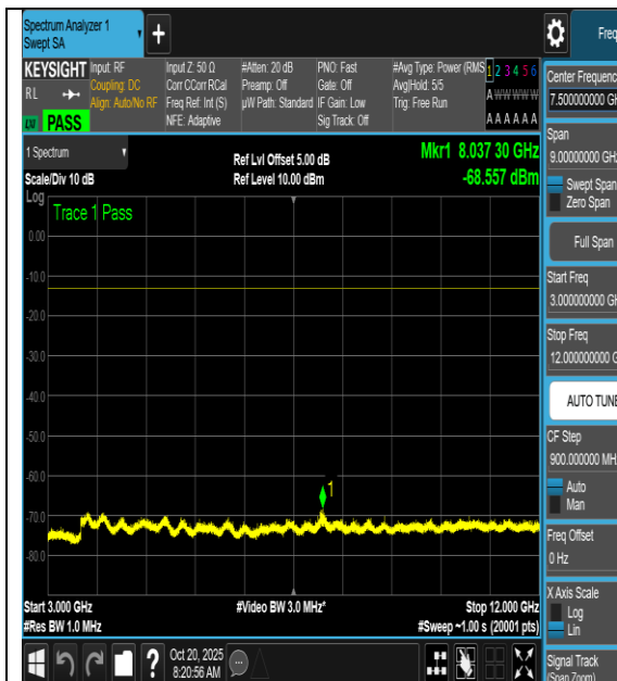
NTNV-n66-PC3-15-5-L-DFT-QPSK-Outter_Full- 3000-12000-PASS
