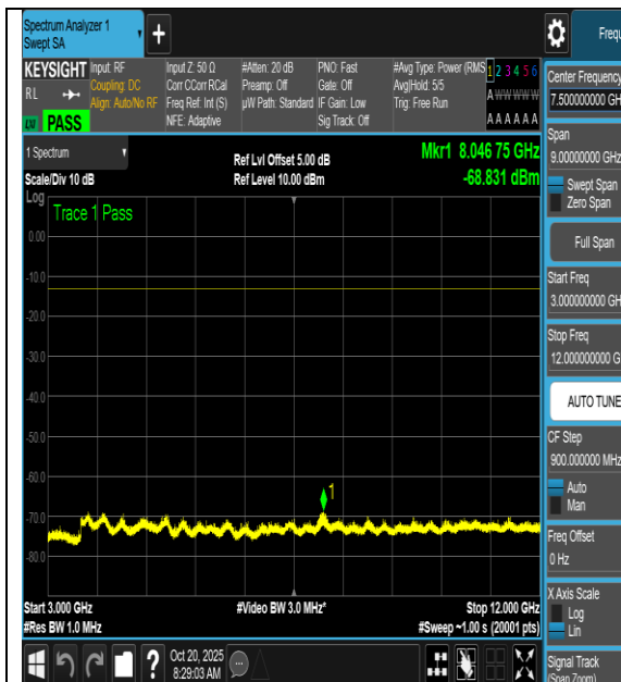
NTNV-n66-PC3-15-5-L-DFT-16QAM-Outer_Full- 3000-12000-PASS
