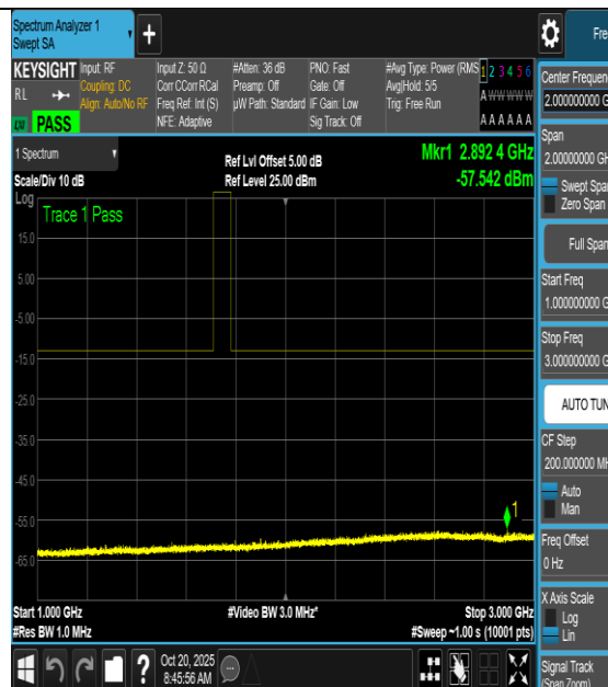
NTNV-n66-PC3-15-5-L-DFT-256QAM- Inner_1RB_Left-1000-3000-PASS
