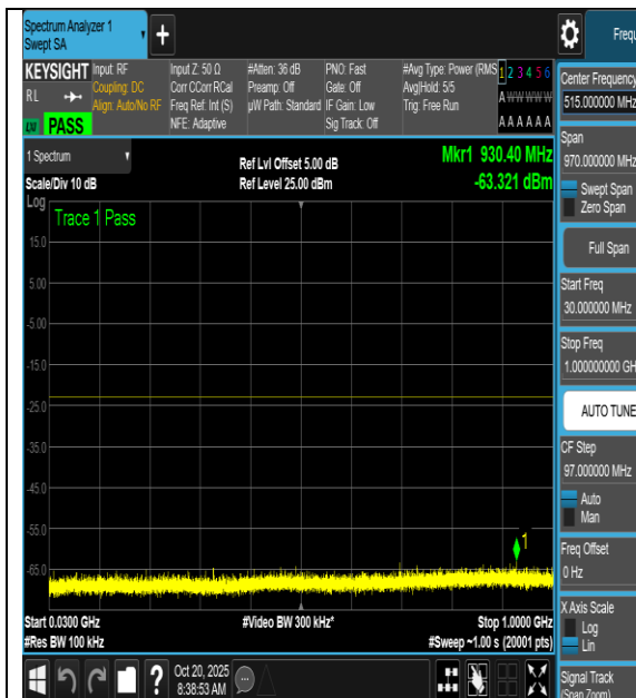
NTNV-n66-PC3-15-5-L-DFT-64QAM- Inner_1RB_Left-30-1000-PASS
