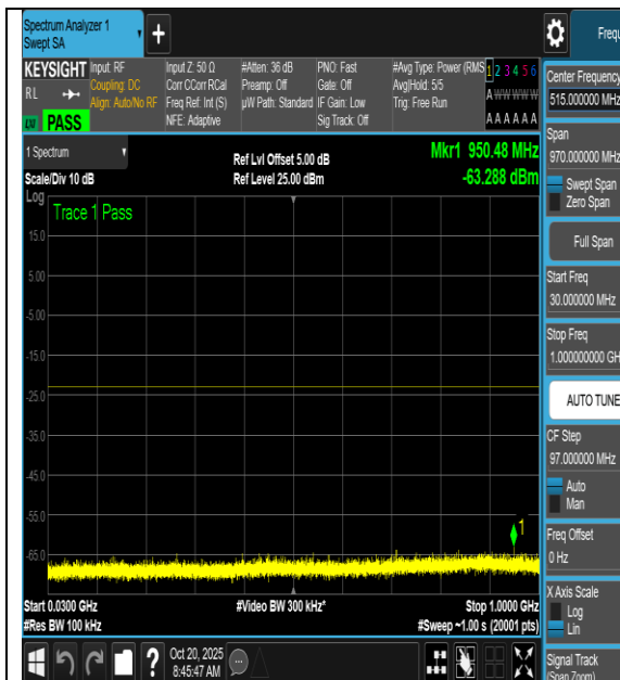
NTNV-n66-PC3-15-5-L-DFT-256QAM- Inner_1RB_Left-30-1000-PASS
