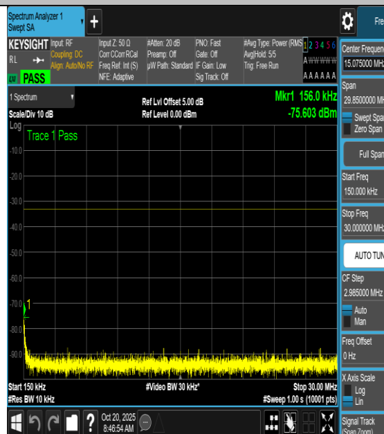
NTNV-n66-PC3-15-5-L-DFT-256QAM- Inner_1RB_Left-12000-20000-PASS
