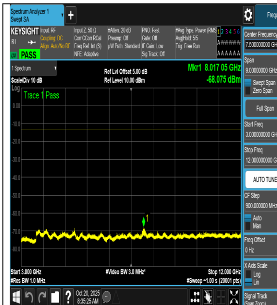
NTNV-n66-PC3-15-5-L-DFT-64QAM-Outer_Full- 3000-12000-PASS
