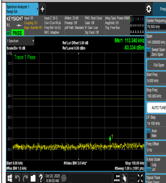
NTNV-n66-PC3-15-5-L-DFT-64QAM- Edge_1RB_Left-0.009-0.15-PASS
