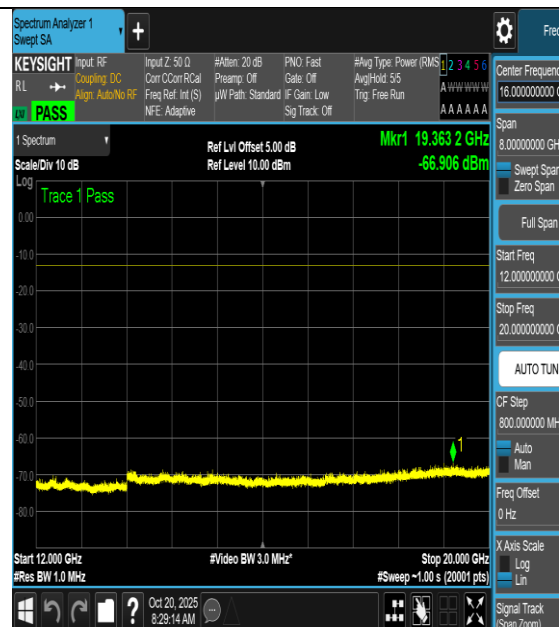
NTNV-n66-PC3-15-5-L-DFT-16QAM-Outer_Full- 12000-20000-PASS
