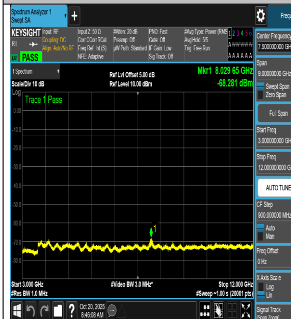
NTNV-n66-PC3-15-5-L-DFT-256QAM- Inner_1RB_Left-3000-12000-PASS
