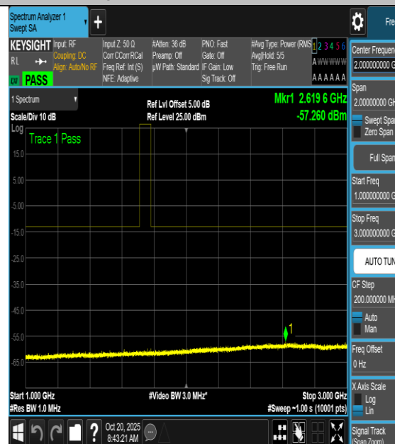
NTNV-n66-PC3-15-5-L-DFT-256QAM- Edge_1RB_Left-0.15-30-PASS
