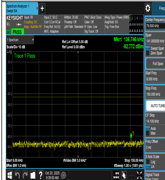
NTNV-n66-PC3-15-5-L-DFT-64QAM- Inner_1RB_Left-3000-12000-PASS
