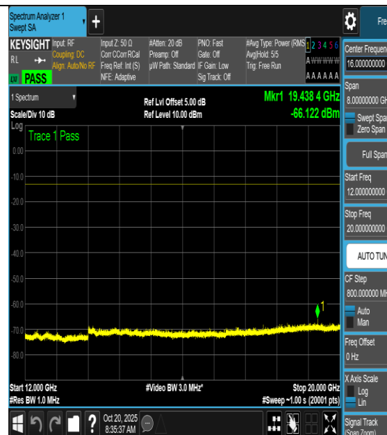
NTNV-n66-PC3-15-5-L-DFT-64QAM-Outer_Full- 12000-20000-PASS
