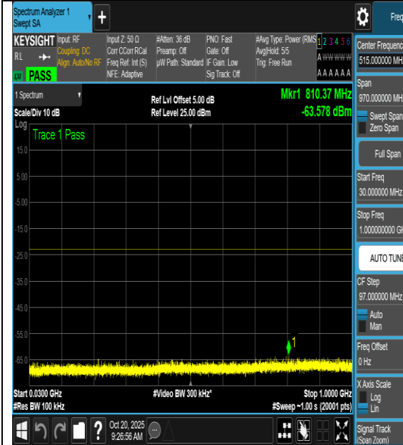
NTNV-n66-PC3-15-5-L-CP-16QAM-Edge_1RB_Left-0.009-0.15-PASS
