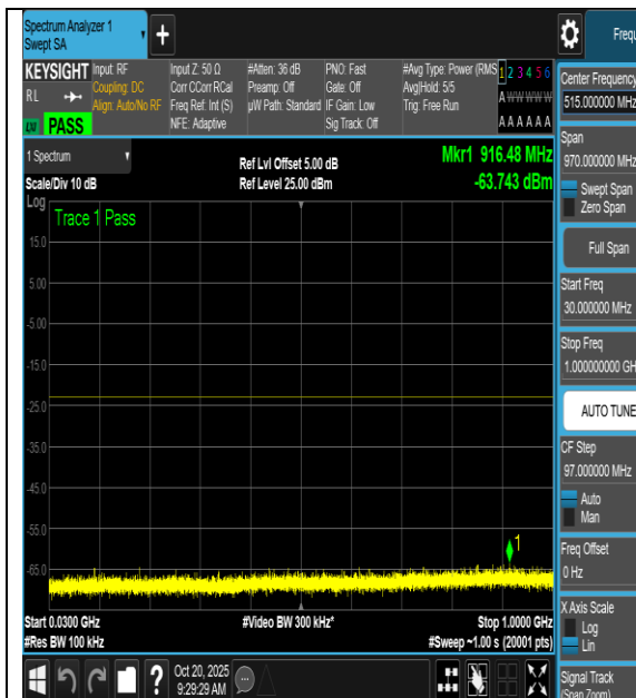
NTNV-n66-PC3-15-5-L-CP-16QAM- Inner_1RB_Left-30-1000-PASS
