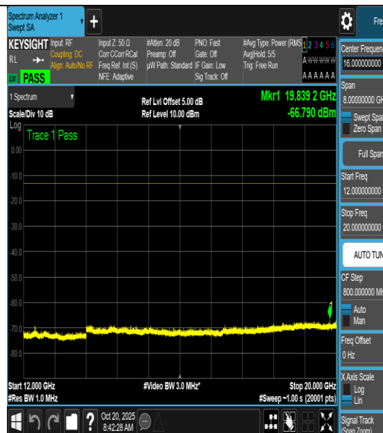
NTNV-n66-PC3-15-5-L-DFT-256QAM-Outer_Full- 12000-20000-PASS
