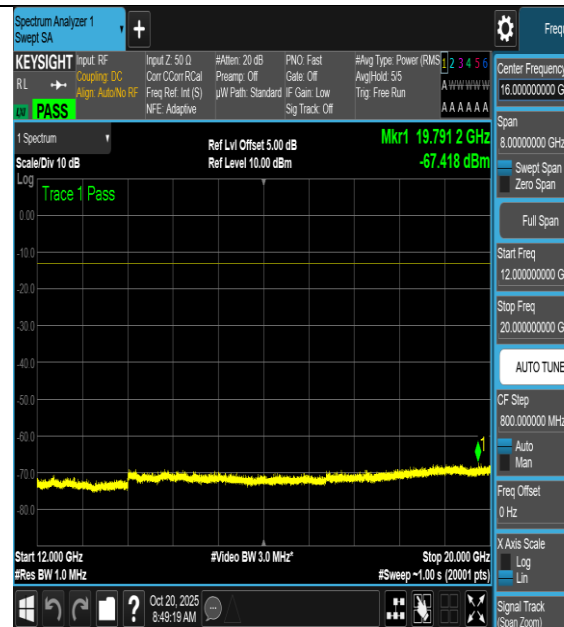
NTNV-n66-PC3-15-5-L-CP-QPSK-Outet_Full-12000-20000-PASS
