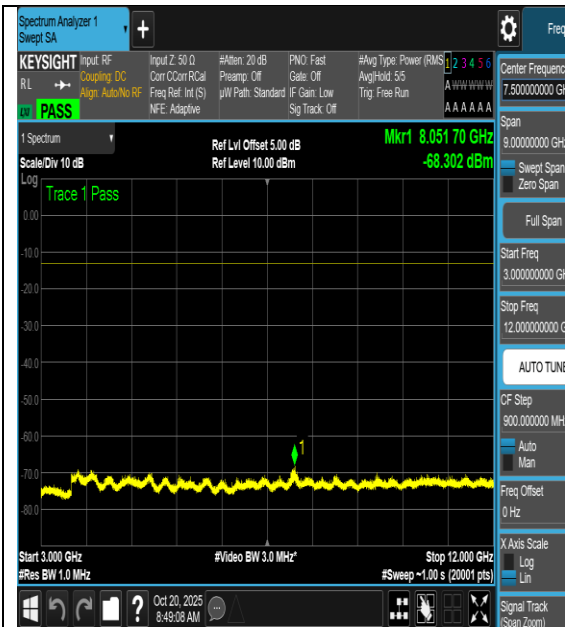
NTNV-n66-PC3-15-5-L-CP-QPSK-Outet_Full-3000-12000-PASS
