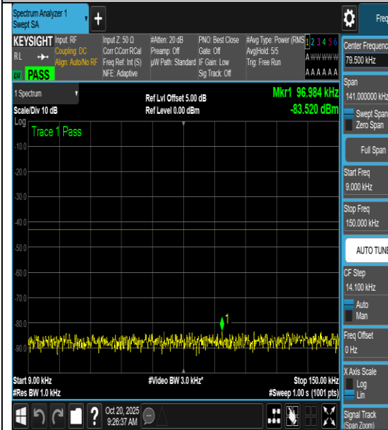
NTNV-n66-PC3-15-5-L-CP-16QAM-Edge_1RB_Left-0.009-0.15-PASS
