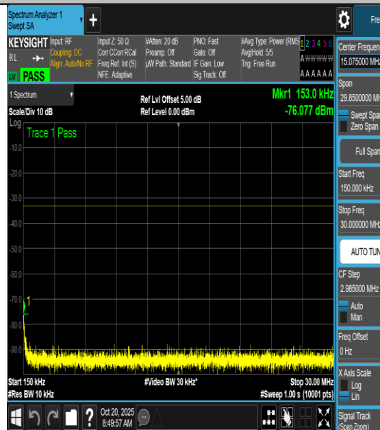
NTNV-n66-PC3-15-5-L-CP-QPSK- Edge_1RB_Left-0.15-30-PASS
