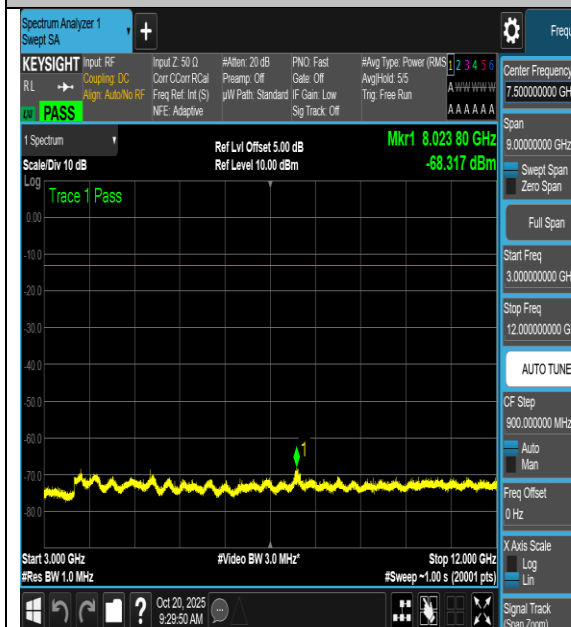
NTNV-n66-PC3-15-5-L-CP-16QAM- Inner_1RB_Left-3000-12000-PASS
