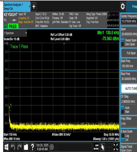
NTNV-n66-PC3-15-5-L-CP-16QAM-Edge_1RB_Left-0.15-30-PASS
