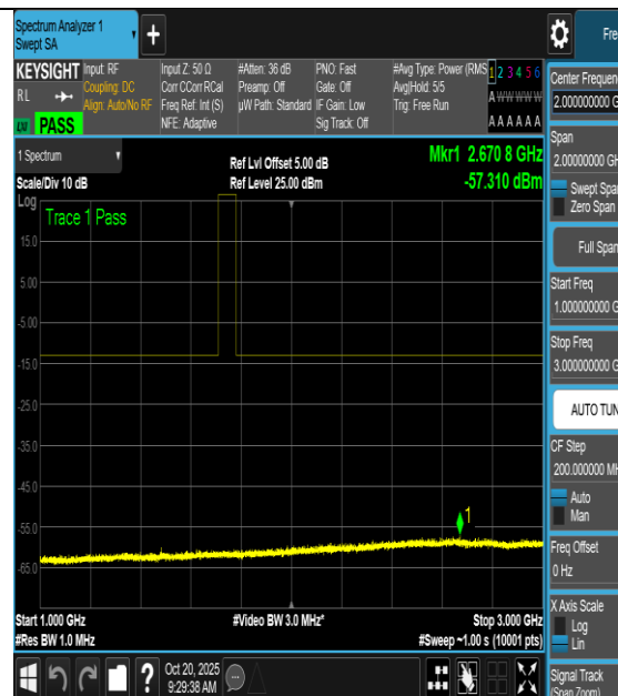
NTNV-n66-PC3-15-5-L-CP-16QAM- Inner_1RB_Left-1000-3000-PASS
