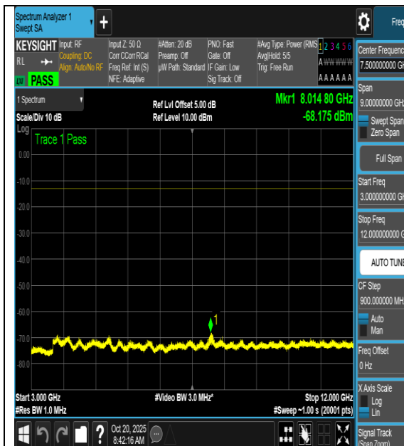
NTNV-n66-PC3-15-5-L-DFT-256QAM-Outer_Full- 3000-12000-PASS
