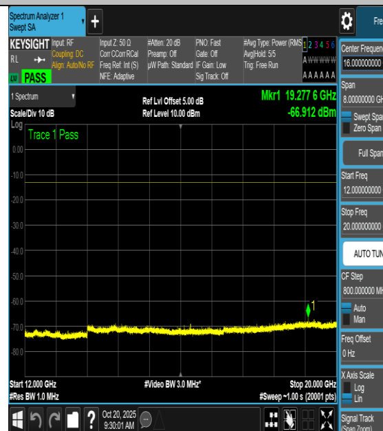
NTNV-n66-PC3-15-5-L-CP-16QAM- Inner_1RB_Left-12000-20000-PASS
