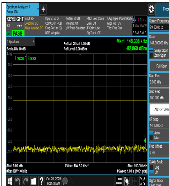
NTNV-n66-PC3-15-5-L-CP-64QAM- Edge_1RB_Right-0.009-0.15-PASS
