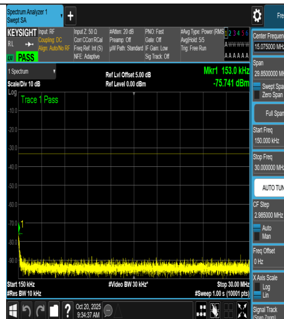
NTNV-n66-PC3-15-5-L-CP-64QAM- Edge_1RB_Right-0.15-30-PASS
