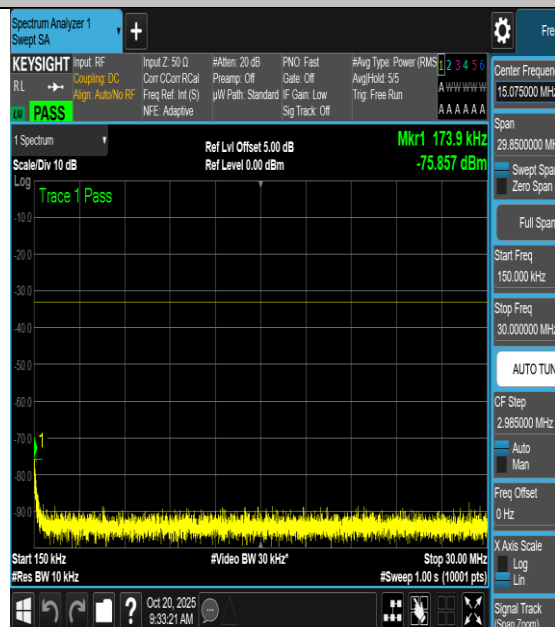
NTNV-n66-PC3-15-5-L-CP-64QAM- Edge_1RB_Left-0.15-30-PASS
