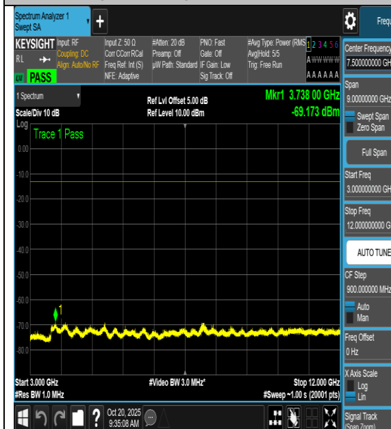
NTNV-n66-PC3-15-5-L-CP-64QAM- Edge_1RB_Right-30-1000-PASS
