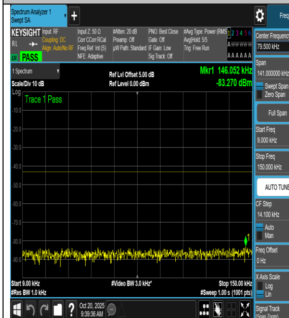
NTNV-n66-PC3-15-5-L-CP-256QAM- Edge_1RB_Left-0.009-0.15-PASS
