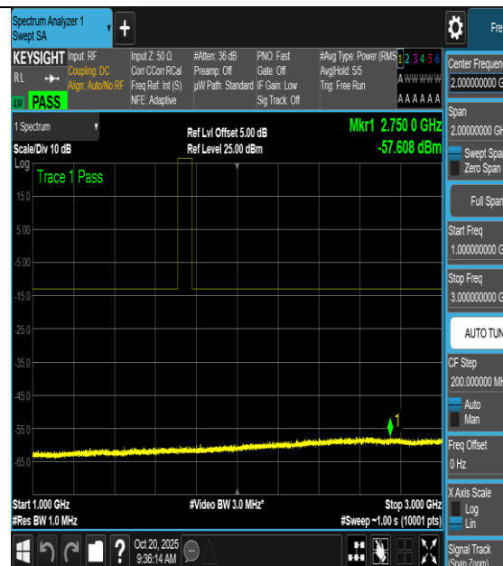
NTNV-n66-PC3-15-5-L-CP-64QAM- Inner_1RB_Left-1000-3000-PASS
