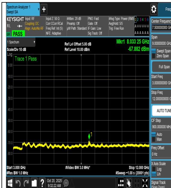
NTNV-n66-PC3-15-5-L-CP-64QAM-Outer_Full- 3000-12000-PASS
