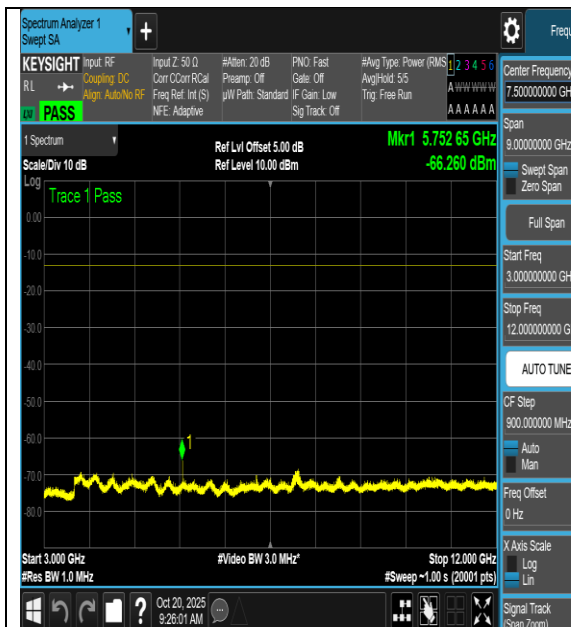
NTNV-n66-PC3-15-5-L-CP-16QAM-Outer_Full- 3000-12000-PASS
