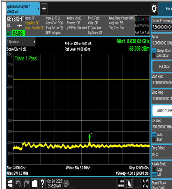
NTNV-n66-PC3-15-5-L-CP-64QAM- Inner_1RB_Left-3000-12000-PASS
