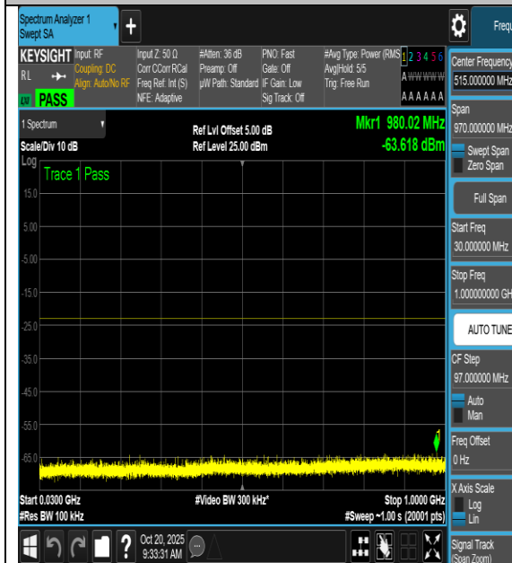
NTNV-n66-PC3-15-5-L-CP-64QAM- Edge_1RB_Left-0.009-0.15-PASS
