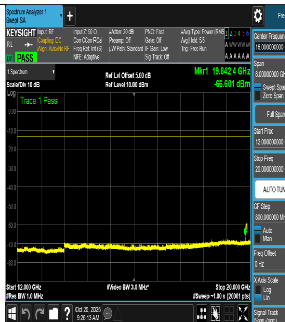
NTNV-n66-PC3-15-5-L-CP-16QAM-Outer_Full- 12000-20000-PASS
