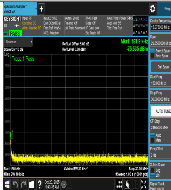
NTNV-n66-PC3-15-5-L-CP-256QAM- Inner_1RB_Left-12000-20000-PASS
