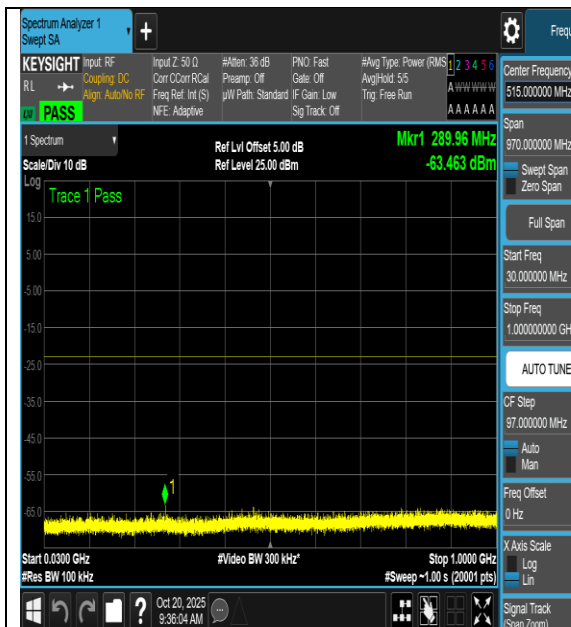
NTNV-n66-PC3-15-5-L-CP-64QAM- Inner_1RB_Left-30-1000-PASS
