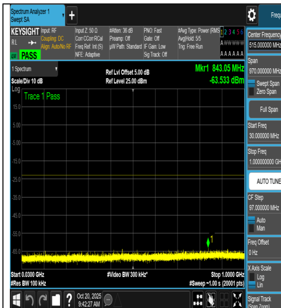
NTNV-n66-PC3-15-5-L-CP-256QAM- Inner_1RB_Left-30-1000-PASS
