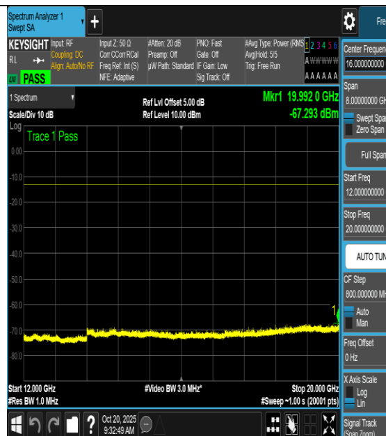
NTNV-n66-PC3-15-5-L-CP-64QAM-Outer_Full- 12000-20000-PASS
