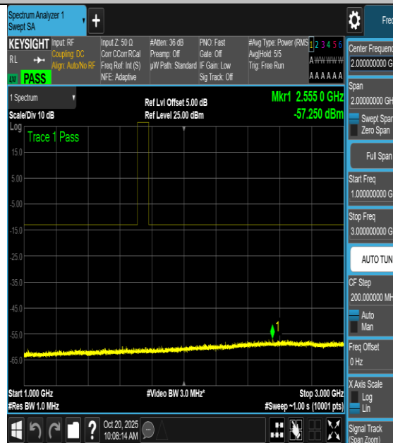
NTNV-n66-PC3-15-40-H-DFT-QPSK- Edge_1RB_Left-0.15-30-PASS
