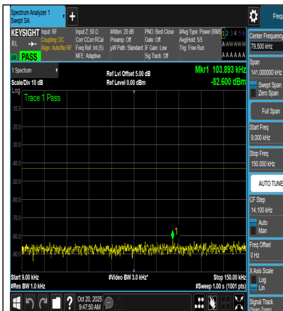
NTNV-n66-PC3-15-40-H-DFT-BPSK- Edge_1RB_Right-0.009-0.15-PASS
