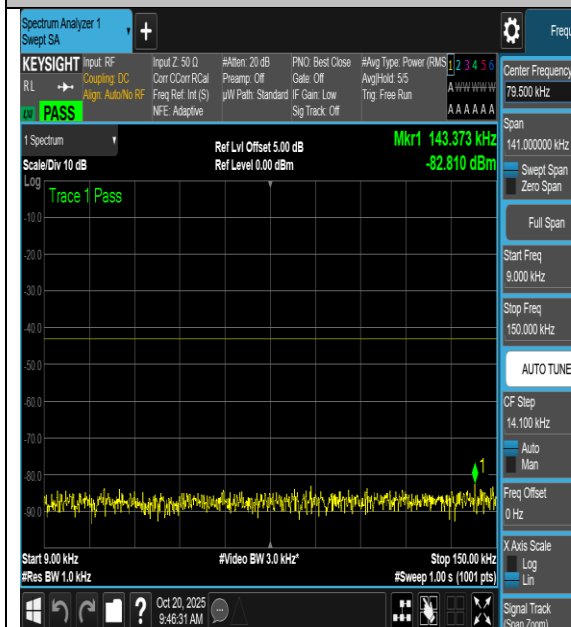
NTNV-n66-PC3-15-40-H-DFT-BPSK- Edge_1RB_Left-0.009-0.15-PASS
