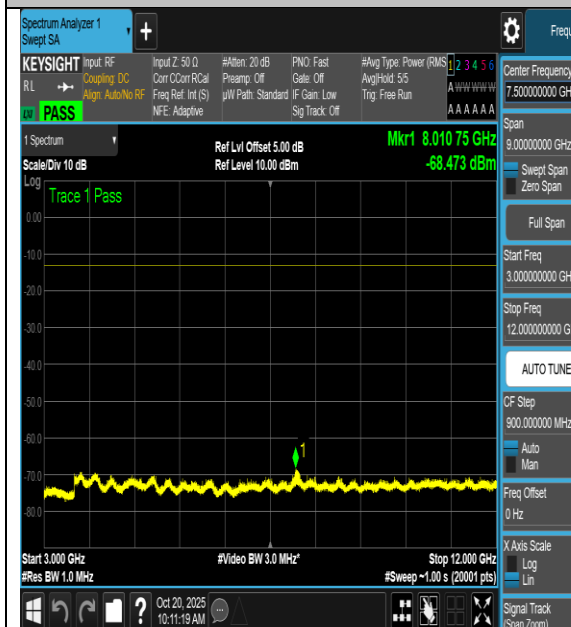
NTNV-n66-PC3-15-40-H-DFT-QPSK- Inner_1RB_Left-3000-12000-PASS
