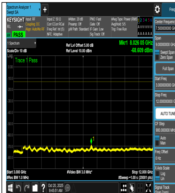
NTNV-n66-PC3-15-40-H-DFT-BPSK-Outer_Full- 3000-12000-PASS
