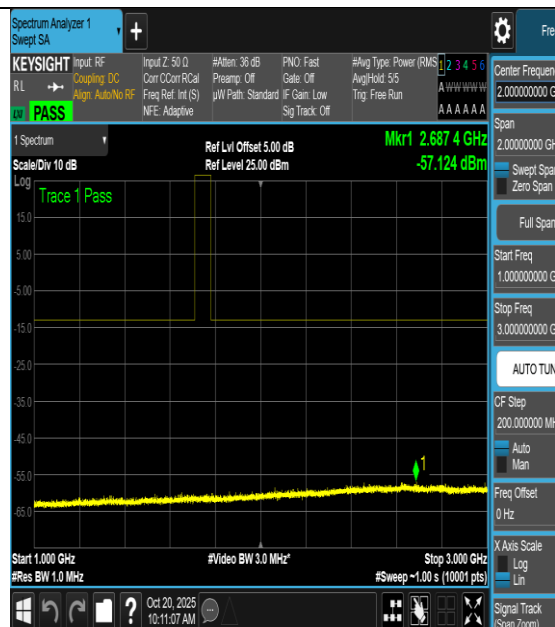
NTNV-n66-PC3-15-40-H-DFT-QPSK- Inner_1RB_Left-1000-3000-PASS
