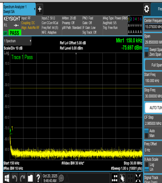
NTNV-n66-PC3-15-40-H-DFT-BPSK- Edge_1RB_Left-0.15-30-PASS
