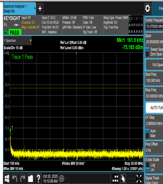
NTNV-n66-PC3-15-40-H-DFT-QPSK- Inner_1RB_Left-12000-20000-PASS
