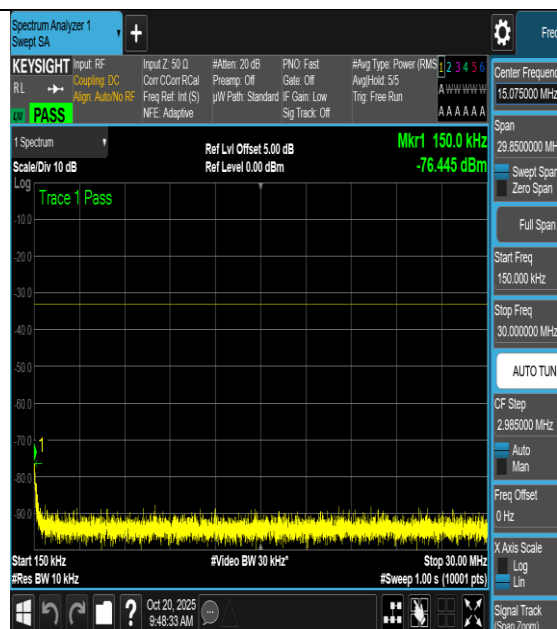
NTNV-n66-PC3-15-40-H-DFT-BPSK- Edge_1RB_Right-0.15-30-PASS
