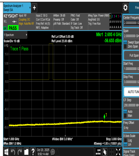
NTNV-n66-PC3-15-40-H-DFT-BPSK- Inner_1RB_Left-1000-3000-PASS
