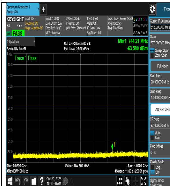
NTNV-n66-PC3-15-40-H-DFT-QPSK- Inner_1RB_Left-30-1000-PASS
