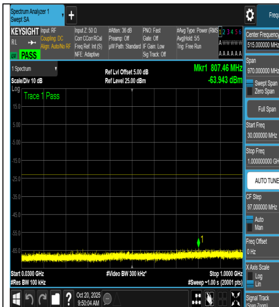
NTNV-n66-PC3-15-40-H-DFT-BPSK- Inner_1RB_Left-30-1000-PASS
