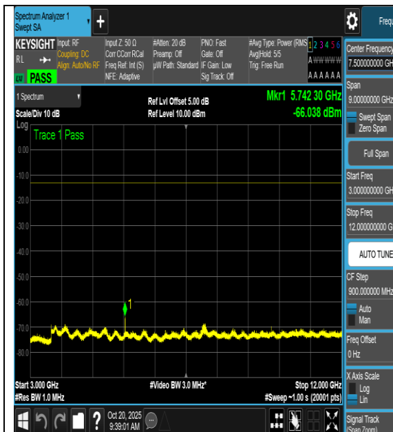
NTNV-n66-PC3-15-5-L-CP-256QAM-Outer_Full- 3000-12000-PASS
