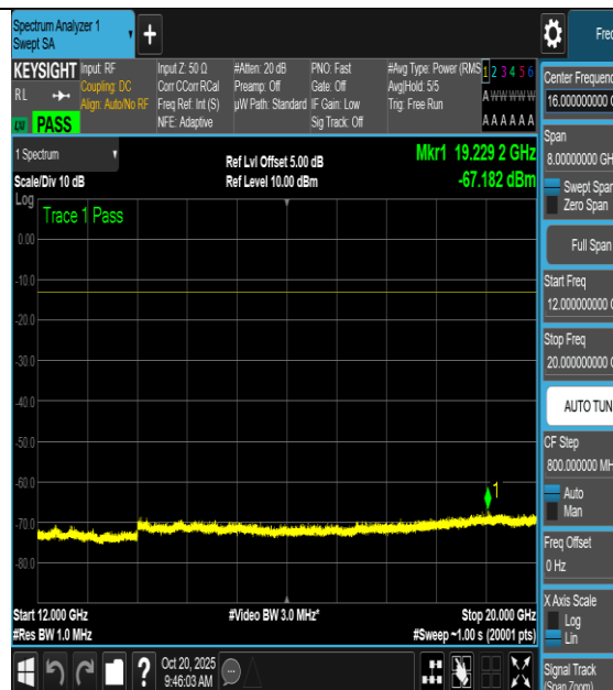
NTNV-n66-PC3-15-40-H-DFT-BPSK-Outer_Full- 12000-20000-PASS
