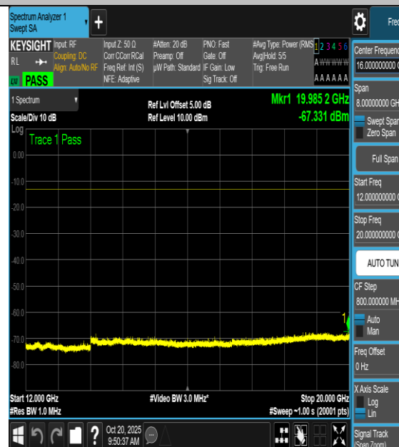
NTNV-n66-PC3-15-40-H-DFT-BPSK- Inner_1RB_Left-12000-20000-PASS
