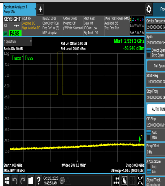
NTNV-n66-PC3-15-40-H-DFT-BPSK- Edge_1RB_Right-1000-3000-PASS
