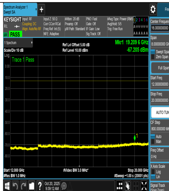
NTNV-n66-PC3-15-5-L-CP-256QAM-Outer_Full- 12000-20000-PASS
