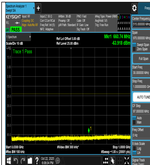
NTNV-n66-PC3-15-40-H-DFT-16QAM- Inner_1RB_Left-30-1000-PASS
