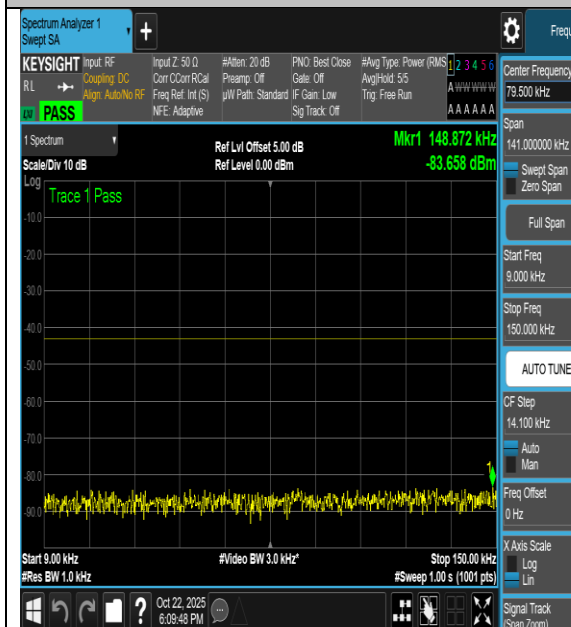
NTNV-n66-PC3-15-40-H-DFT-64QAM- Edge_1RB_Left-0.009-0.15-PASS
