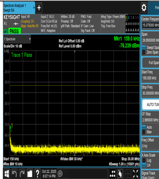
NTNV-n66-PC3-15-40-H-DFT-16QAM- Inner_1RB_Left-12000-20000-PASS
