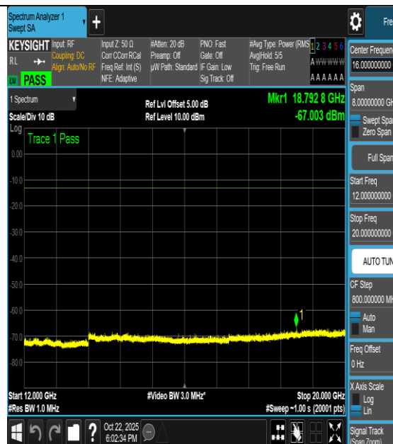
NTNV-n66-PC3-15-40-H-DFT-16QAM-Outer_Full- 12000-20000-PASS
