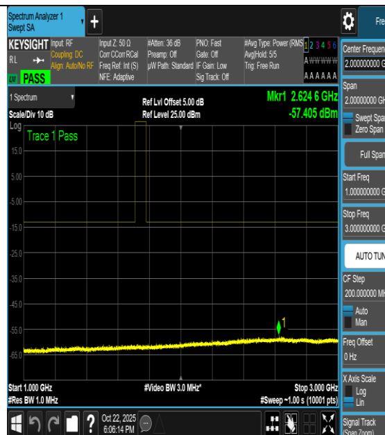
NTNV-n66-PC3-15-40-H-DFT-16QAM- Inner_1RB_Left-1000-3000-PASS
