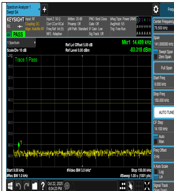
NTNV-n66-PC3-15-40-H-DFT-16QAM- Edge_1RB_Right-0.009-0.15-PASS
