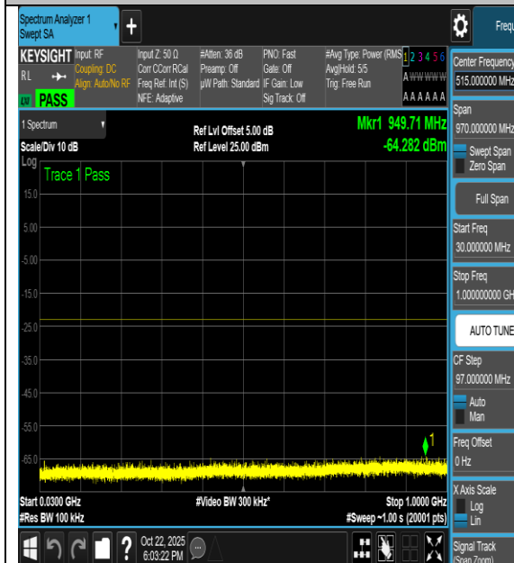
NTNV-n66-PC3-15-40-H-DFT-16QAM- Edge_1RB_Left-0.009-0.15-PASS
