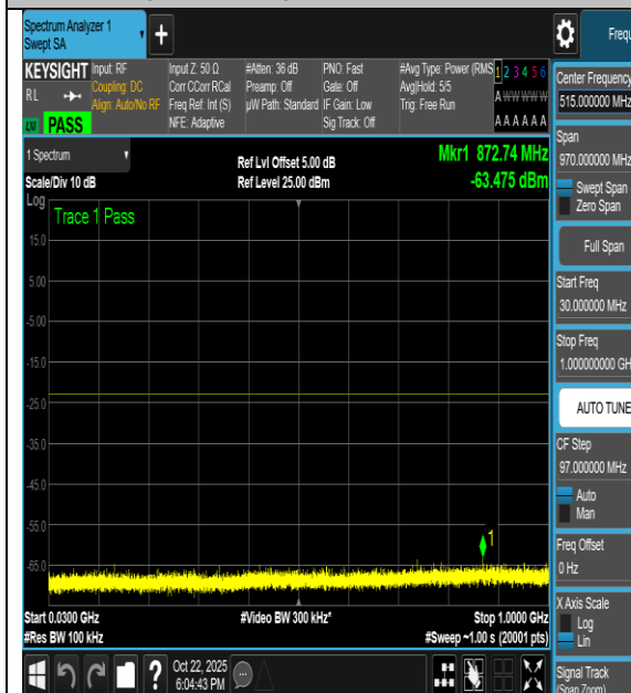
NTNV-n66-PC3-15-40-H-DFT-16QAM- Edge_1RB_Right-30-1000-PASS
