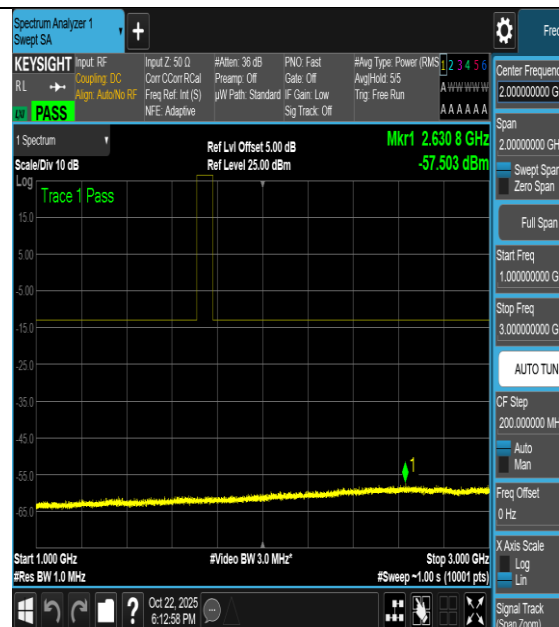
NTNV-n66-PC3-15-40-H-DFT-64QAM- Inner_1RB_Left-1000-3000-PASS
