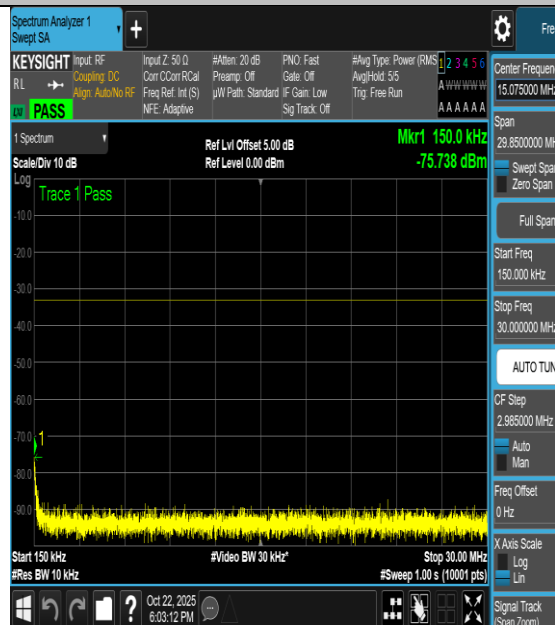
NTNV-n66-PC3-15-40-H-DFT-16QAM- Edge_1RB_Left-0.15-30-PASS
