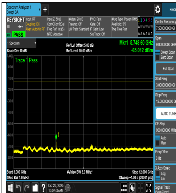
NTNV-n66-PC3-15-40-H-DFT-QPSK-Outer_Full- 3000-12000-PASS
