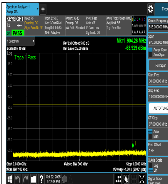
NTNV-n66-PC3-15-40-H-DFT-64QAM- Inner_1RB_Left-30-1000-PASS
