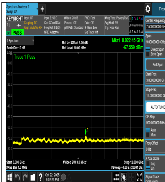
NTNV-n66-PC3-15-40-H-DFT-16QAM-Outer_Full- 3000-12000-PASS
