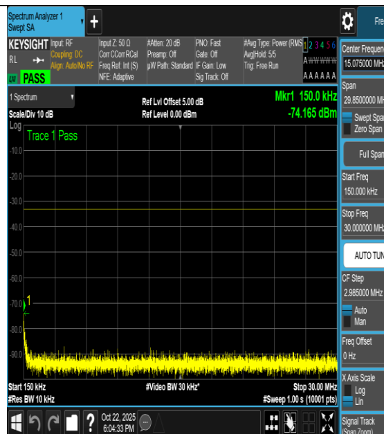
NTNV-n66-PC3-15-40-H-DFT-16QAM- Edge_1RB_Right-0.15-30-PASS
