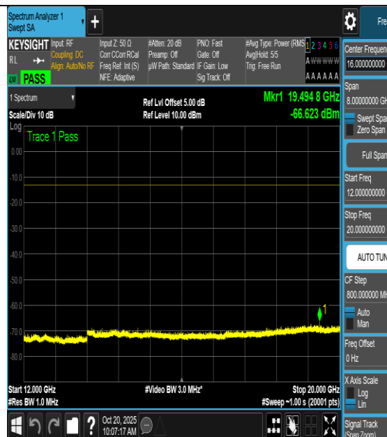
NTNV-n66-PC3-15-40-H-DFT-QPSK-Outer_Full- 12000-20000-PASS
