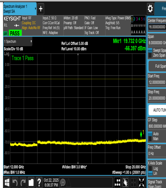
NTNV-n66-PC3-15-40-H-DFT-16QAM- Inner_1RB_Left-12000-20000-PASS
