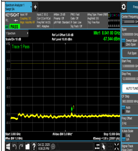
NTNV-n66-PC3-15-40-H-DFT-16QAM- Inner_1RB_Left-3000-12000-PASS
