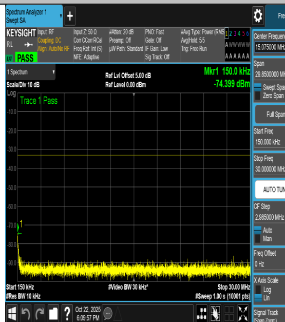
NTNV-n66-PC3-15-40-H-DFT-64QAM- Edge_1RB_Left-0.15-30-PASS
