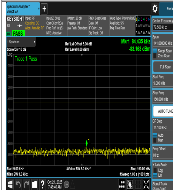
NTNV-n66-PC3-15-40-H-CP-QPSK- Edge_1RB_Left-0.009-0.15-PASS
