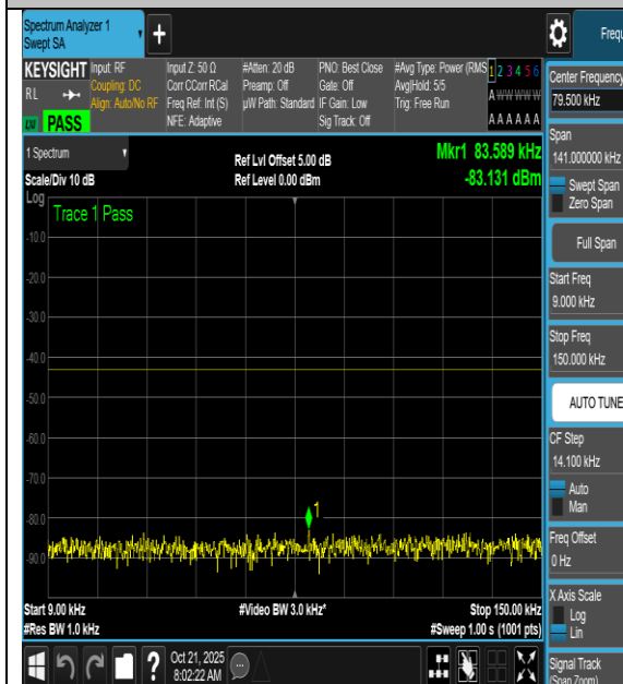
NTNV-n66-PC3-15-40-H-CP-QPSK- Inner_1RB_Left-3000-12000-PASS
