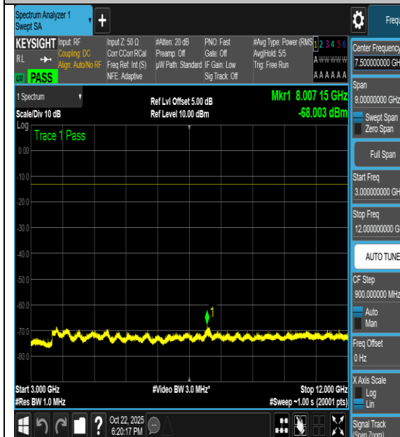
NTNV-n66-PC3-15-40-H-DFT-256QAM- Inner_1RB_Left-3000-12000-PASS
