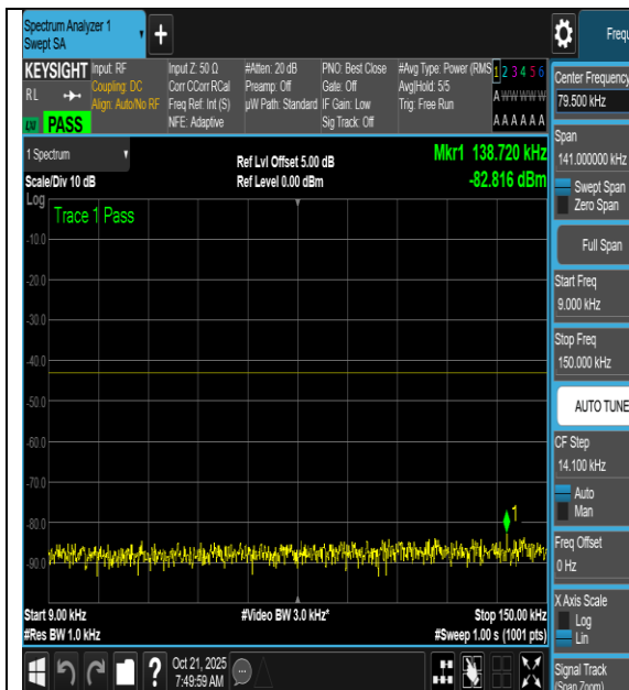
NTNV-n66-PC3-15-40-H-CP-QPSK- Edge_1RB_Right-0.009-0.15-PASS
