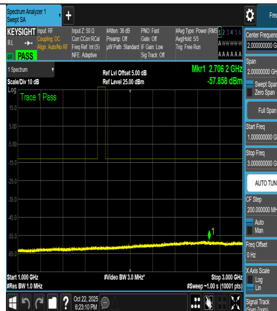
NTNV-n66-PC3-15-40-H-CP-QPSK- Inner_1RB_Left-1000-3000-PASS
