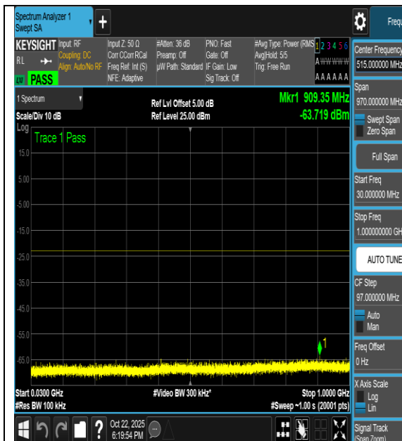
NTNV-n66-PC3-15-40-H-DFT-256QAM- Inner_1RB_Left-30-1000-PASS
