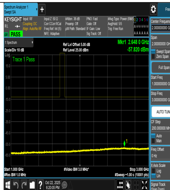
NTNV-n66-PC3-15-40-H-DFT-256QAM- Inner_1RB_Left-1000-3000-PASS
