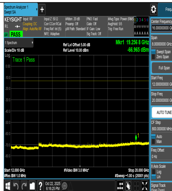
NTNV-n66-PC3-15-40-H-DFT-256QAM- Outer_Full-12000-20000-PASS
