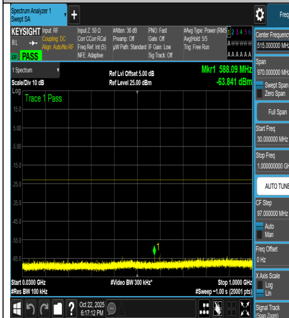
NTNV-n66-PC3-15-40-H-DFT-256QAM- Edge_1RB_Left-0.009-0.15-PASS
