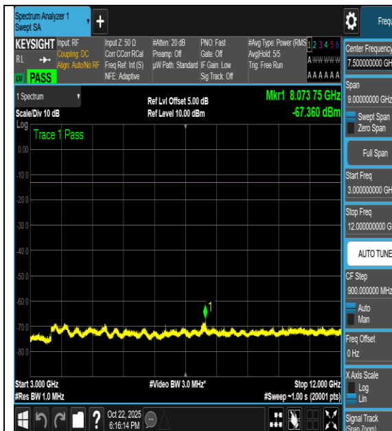
NTNV-n66-PC3-15-40-H-DFT-256QAM- Outer_Full-3000-12000-PASS
