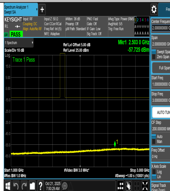
NTNV-n66-PC3-15-40-H-CP-QPSK- Edge_1RB_Right-1000-3000-PASS
