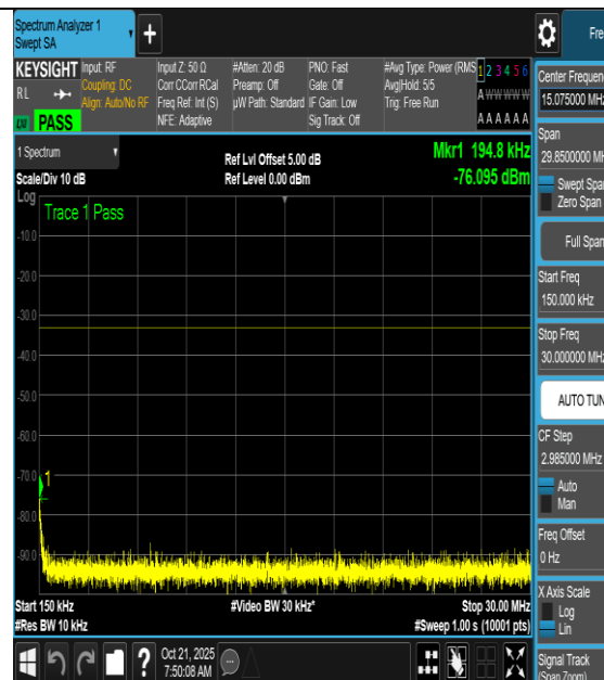
NTNV-n66-PC3-15-40-H-CP-QPSK- Edge_1RB_Right-0.15-30-PASS
