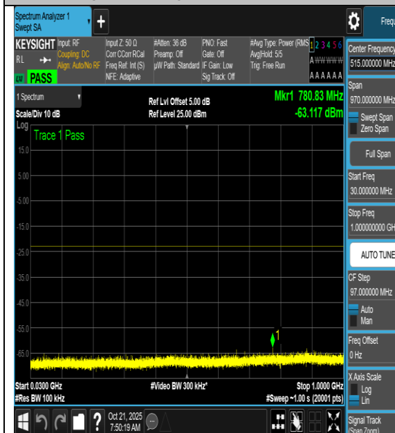
NTNV-n66-PC3-15-40-H-CP-QPSK- Edge_1RB_Right-30-1000-PASS
