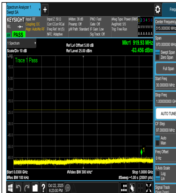
NTNV-n66-PC3-15-40-H-CP-QPSK- Inner_1RB_Left-30-1000-PASS
