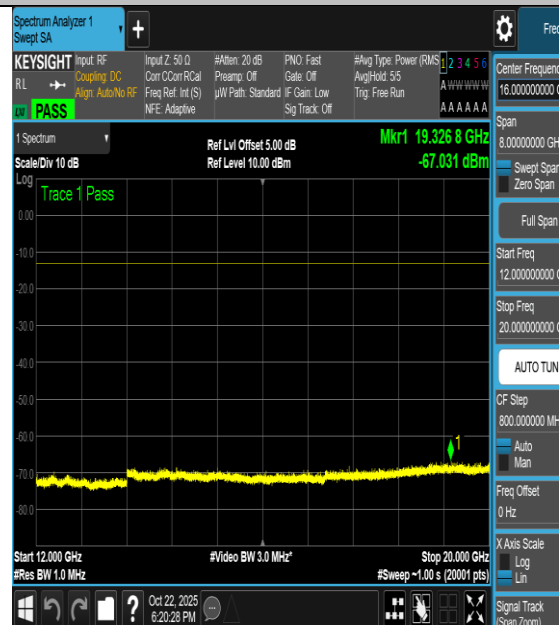
NTNV-n66-PC3-15-40-H-DFT-256QAM- Inner_1RB_Left-12000-20000-PASS
