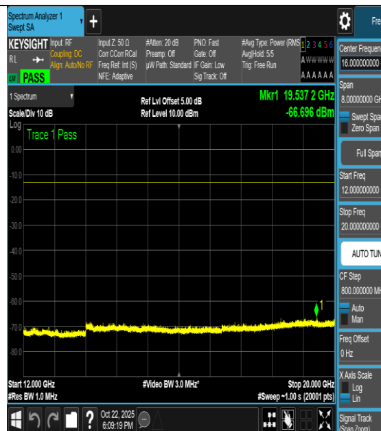
NTNV-n66-PC3-15-40-H-DFT-64QAM-Outer_Full- 12000-20000-PASS
