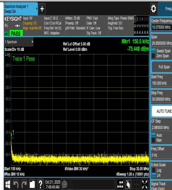
NTNV-n66-PC3-15-40-H-CP-QPSK- Edge_1RB_Left-0.15-30-PASS
