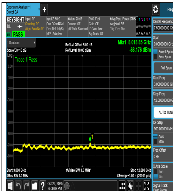
NTNV-n66-PC3-15-40-H-DFT-64QAM-Outer_Full- 3000-12000-PASS
