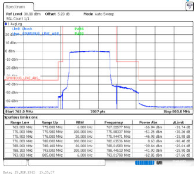
Band13-10MHz-16QAM-23230-50RB#0-PASS
