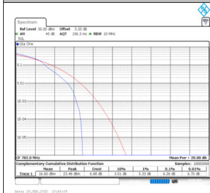
Band13-10MHz-16QAM-23230-1RB#0-PASS
