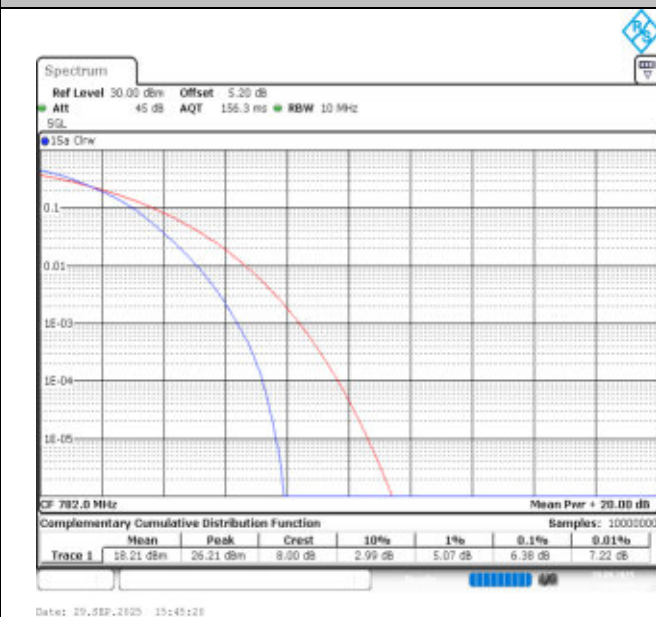
Band13-10MHz-16QAM-23230-50RB#0-PASS
