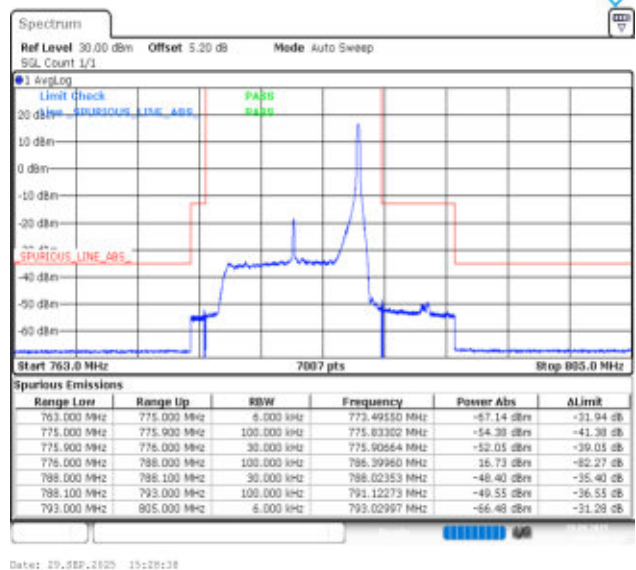
Band13-10MHz-QPSK-23230-1RB#49-PASS
