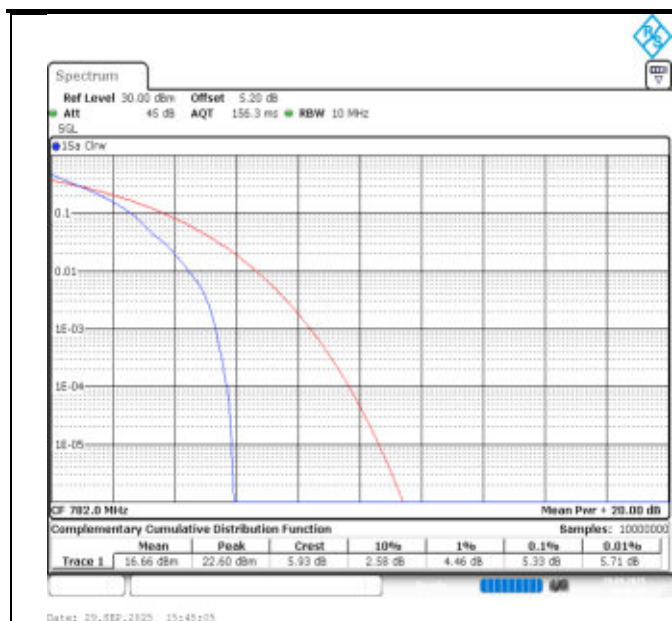
Band13-10MHz-QPSK-23230-1RB#0-PASS
