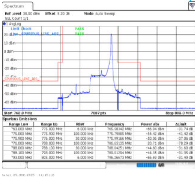
Band13-5MHz-16QAM-23255-1RB#24-PASS
