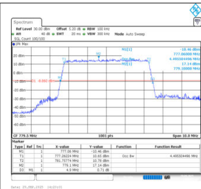
Band13-5MHz-16QAM-23205-25RB#0-PASS
