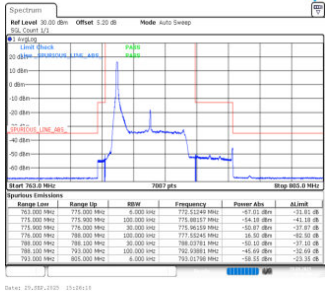
Band13-10MHz-16QAM-23230-1RB#0-PASS
