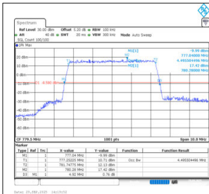
Band13-5MHz-QPSK-23205-25RB#0-PASS
