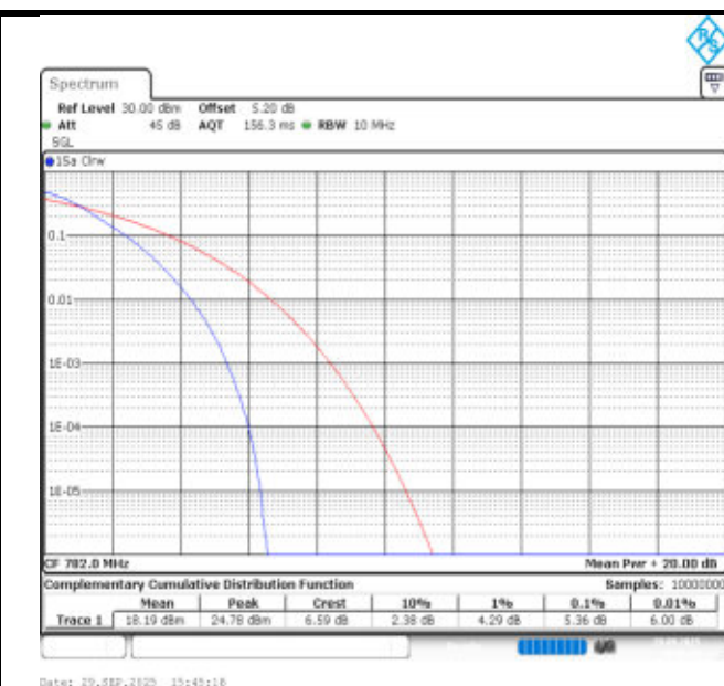
Band13-10MHz-QPSK-23230-50RB#0-PASS
