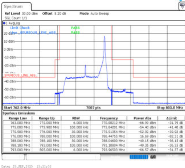
Band13-10MHz-16QAM-23230-1RB#49-PASS
