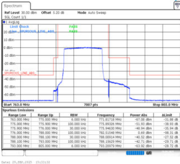
Band13-10MHz-QPSK-23230-50RB#0-PASS
