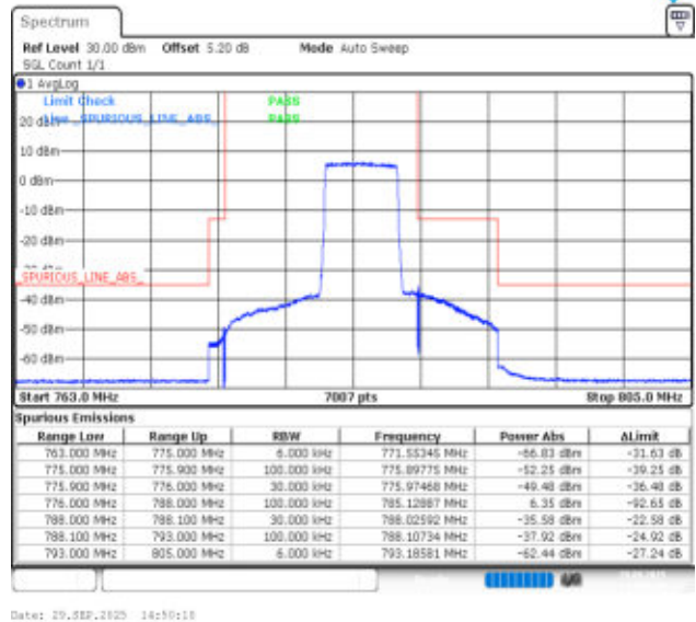
Band13-5MHz-16QAM-23255-25RB#0-PASS
