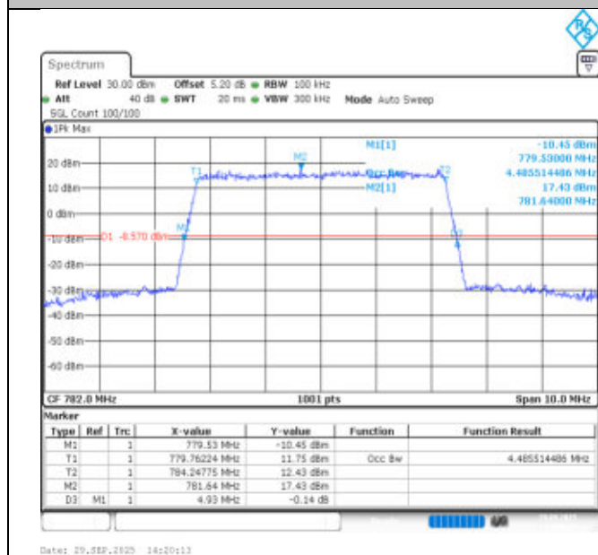
Band13-5MHz-QPSK-23230-25RB#0-PASS
