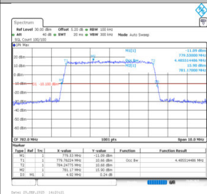
Band13-5MHz-16QAM-23230-25RB#0-PASS
