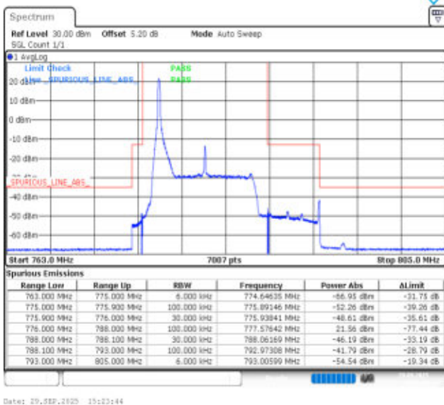
Band13-10MHz-QPSK-23230-1RB#0-PASS
