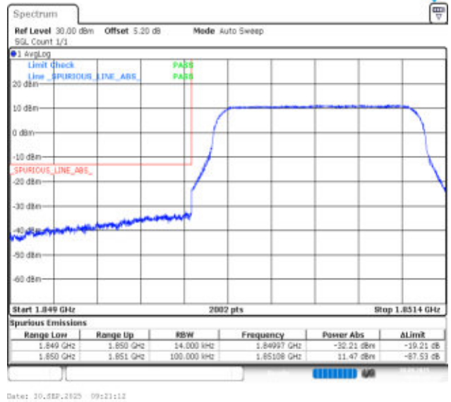
Band25-1.4MHz-16QAM-26047-6RB#0-PASS
