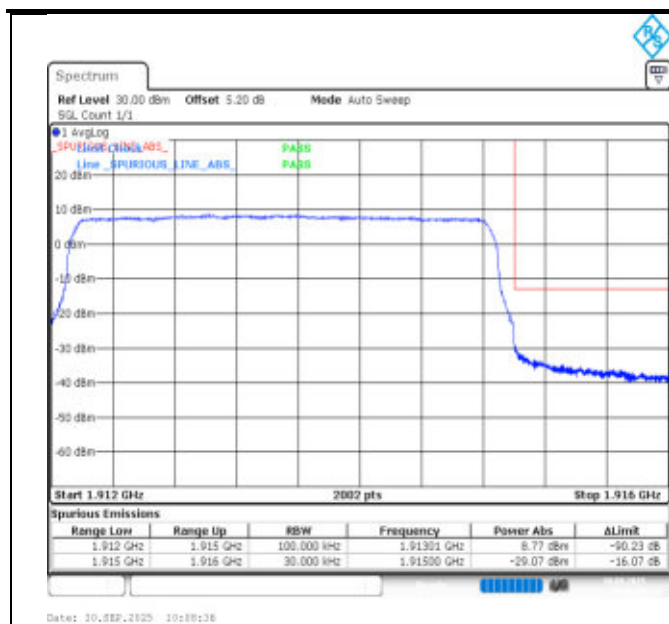
Band25-3MHz-QPSK-26675-15RB#0-PASS
