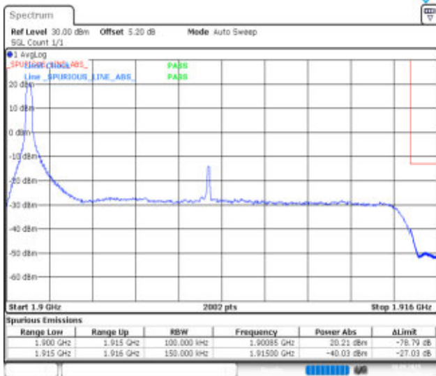
Band25-15MHz-QPSK-26615-1RB#0-PASS
