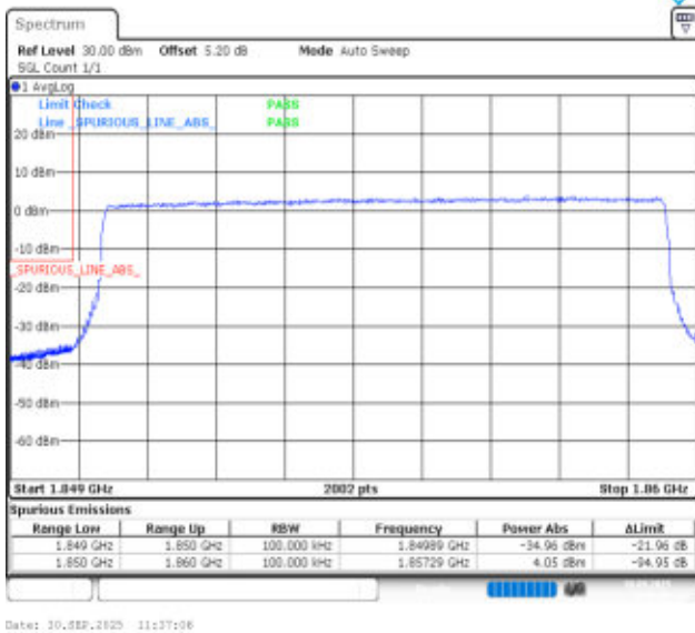
Band25-10MHz-QPSK-26090-50RB#0-PASS
