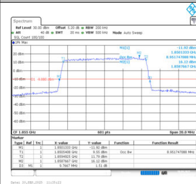
Band25-10MHz-16QAM-26090-50RB#0-PASS
