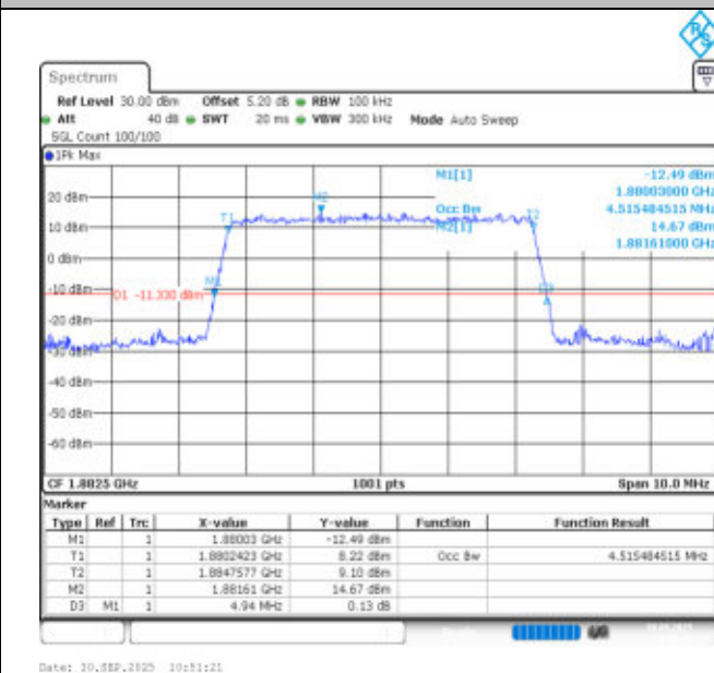
Band25-5MHz-16QAM-26365-25RB#0-PASS
