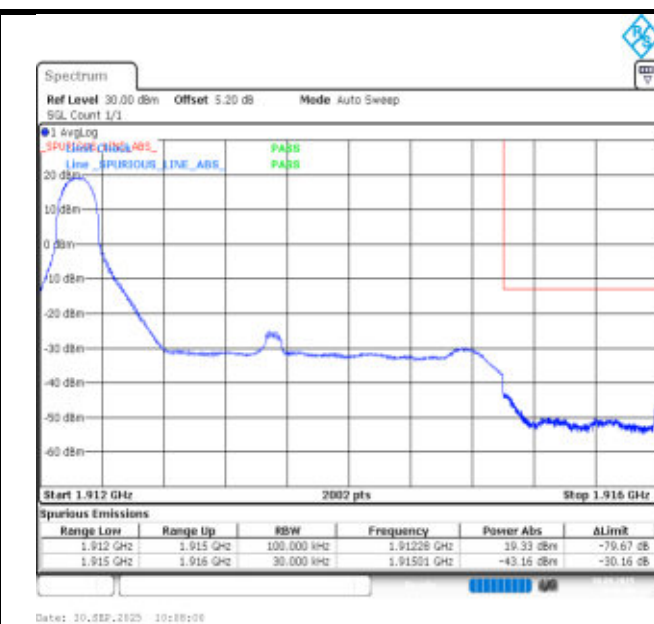
Band25-3MHz-16QAM-26675-1RB#0-PASS
