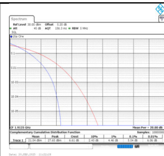
Band25-5MHz-QPSK-26665-25RB#0-PASS
