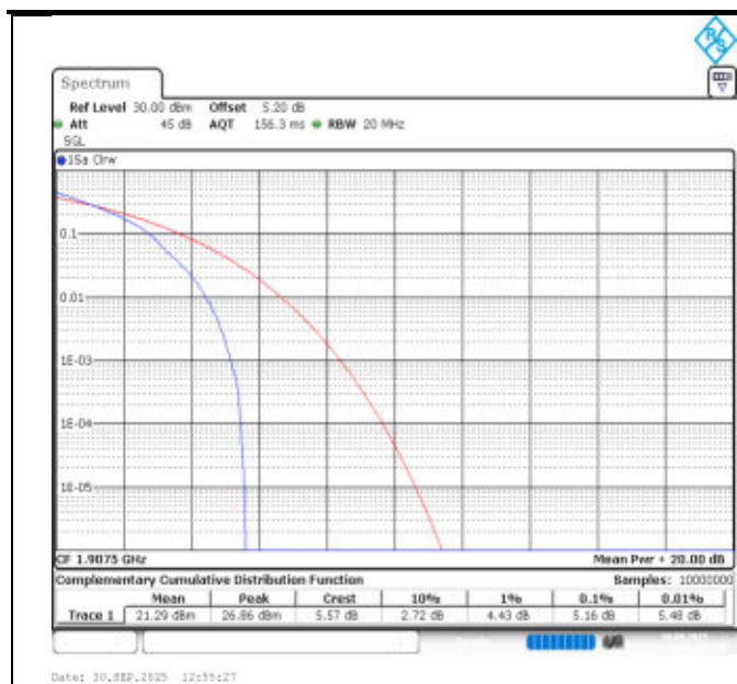
Band25-15MHz-QPSK-26615-1RB#0-PASS
