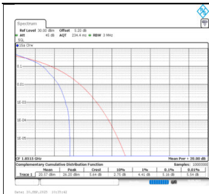
Band25-3MHz-QPSK-26055-1RB#0-PASS
