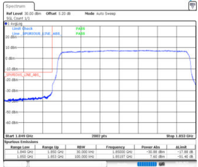
Band25-3MHz-16QAM-26055-15RB#0-PASS
