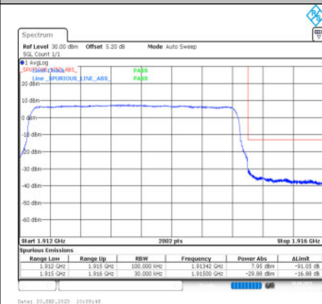
Band25-3MHz-16QAM-26675-15RB#0-PASS
