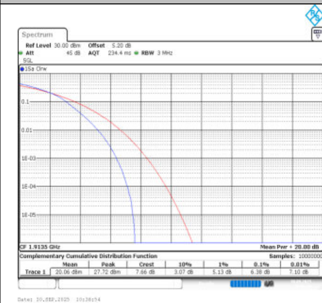
Band25-3MHz-16QAM-26675-15RB#0-PASS
