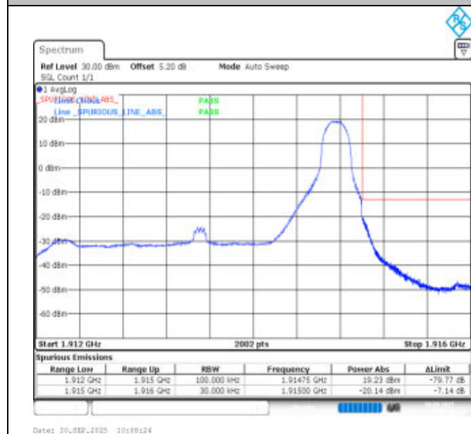
Band25-3MHz-16QAM-26675-1RB#14-PASS
