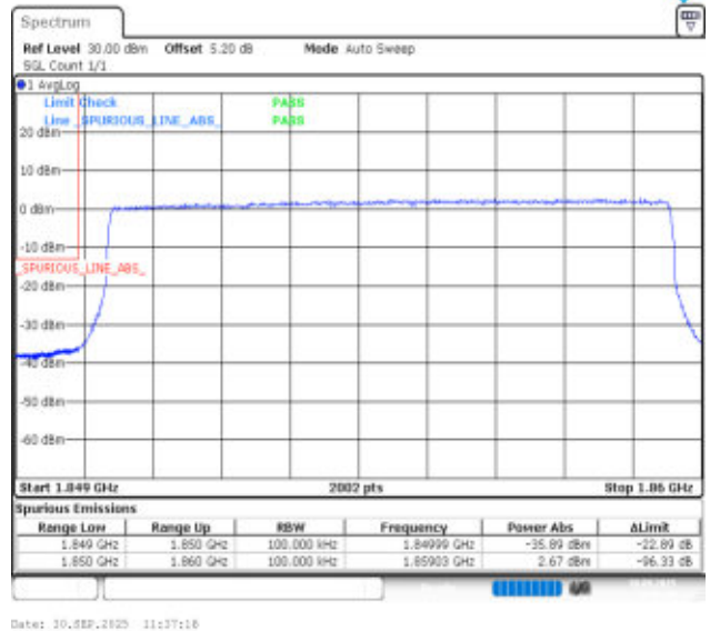
Band25-10MHz-16QAM-26090-50RB#0-PASS
