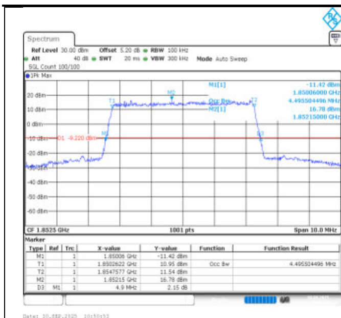
Band25-5MHz-QPSK-26065-25RB#0-PASS
