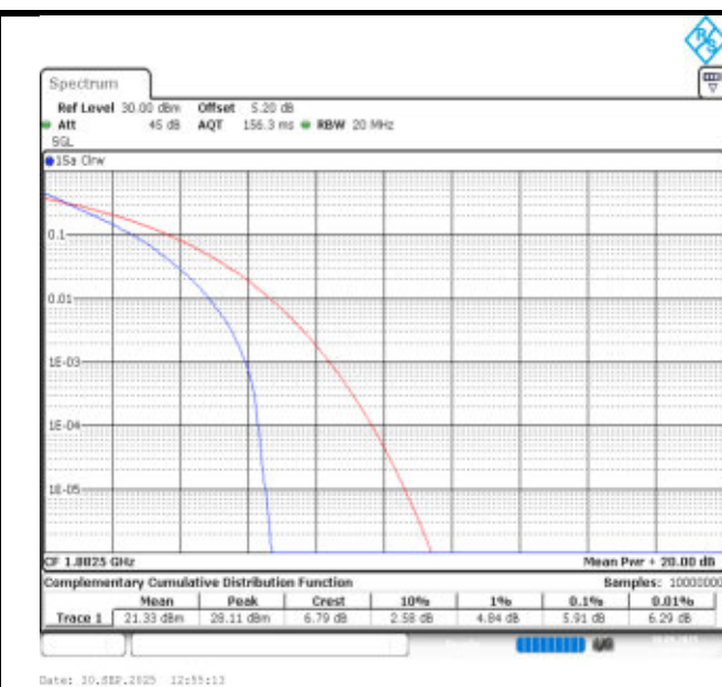
Band25-15MHz-QPSK-26365-75RB#0-PASS
