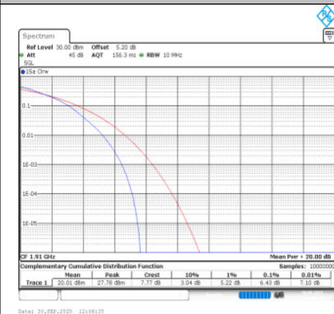
Band25-10MHz-16QAM-26640-50RB#0-PASS
