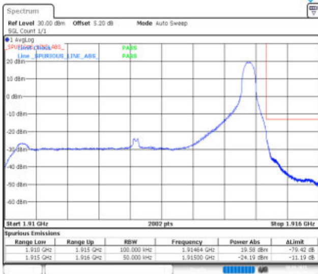
Band25-5MHz-16QAM-26665-1RB#24-PASS
