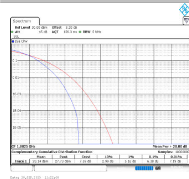
Band25-5MHz-16QAM-26365-25RB#0-PASS
