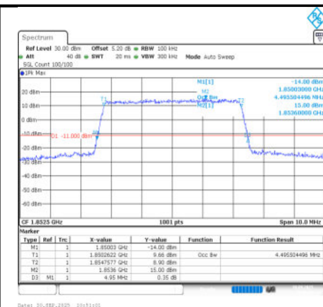
Band25-5MHz-16QAM-26065-25RB#0-PASS
