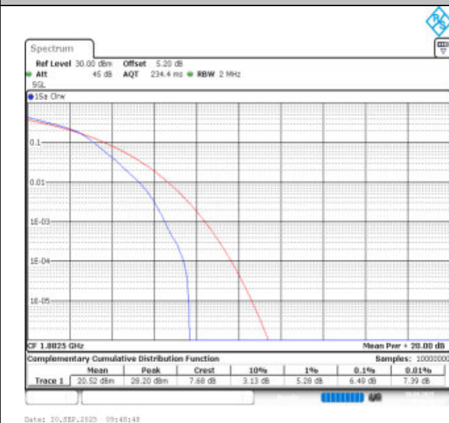
Band25-1.4MHz-16QAM-26365-6RB#0-PASS
