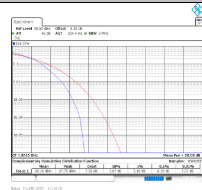
Band25-3MHz-16QAM-26055-15RB#0-PASS
