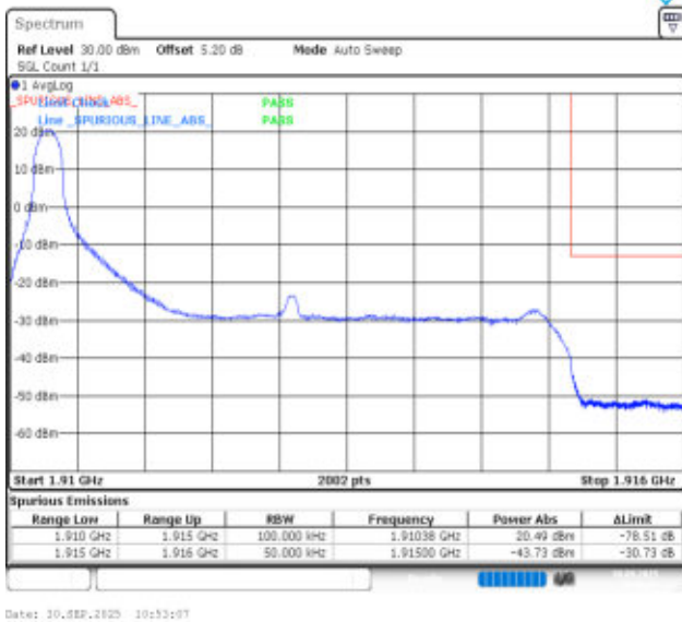
Band25-5MHz-QPSK-26665-1RB#0-PASS
