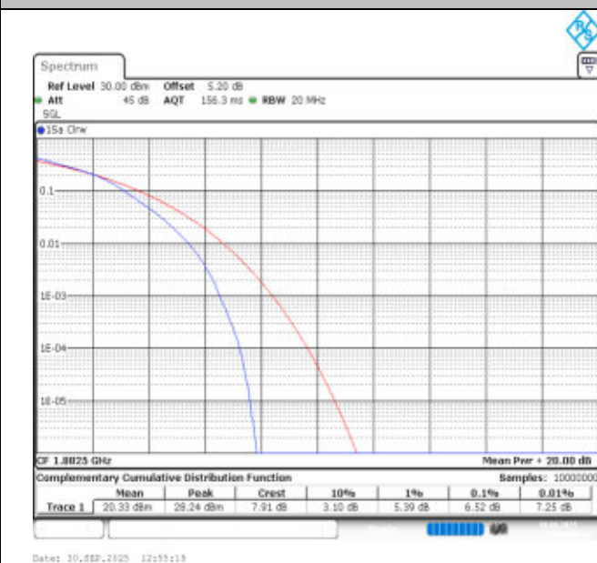
Band25-15MHz-16QAM-26365-75RB#0-PASS
