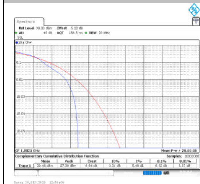
Band25-15MHz-16QAM-26365-1RB#0-PASS
