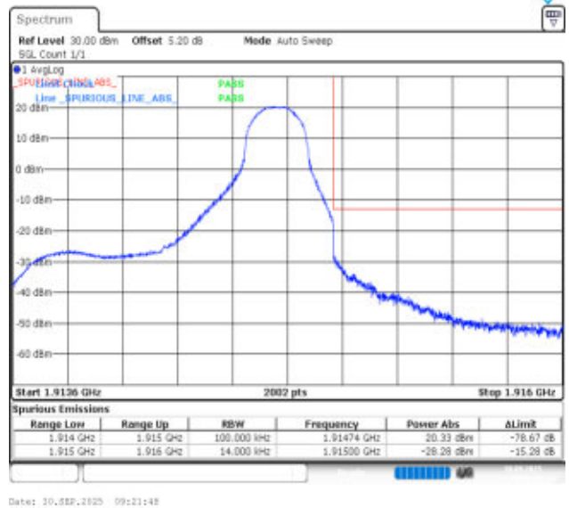
Band25-1.4MHz-QPSK-26683-1RB#5-PASS
