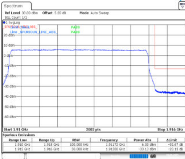
Band25-5MHz-QPSK-26665-25RB#0-PASS
