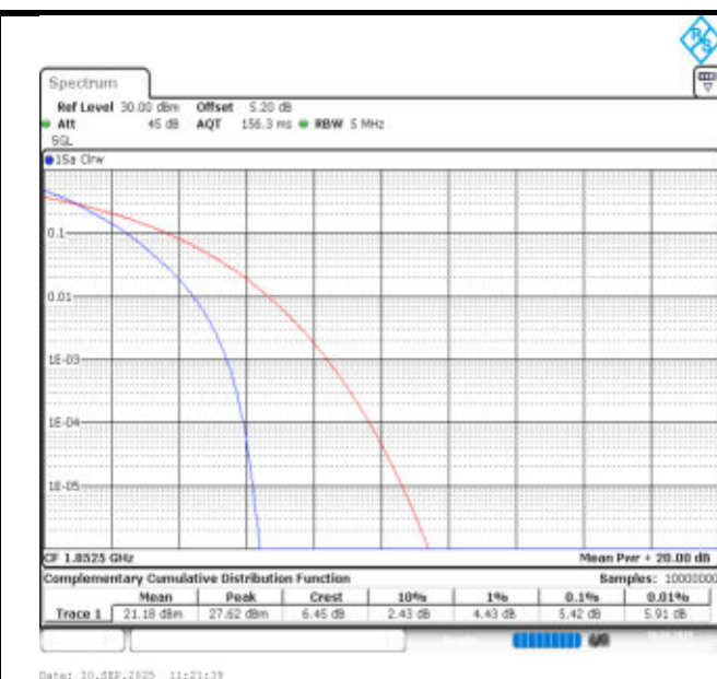
Band25-5MHz-QPSK-26065-25RB#0-PASS
