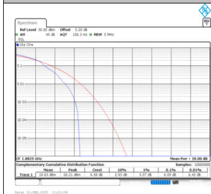
Band25-5MHz-16QAM-26365-1RB#0-PASS
