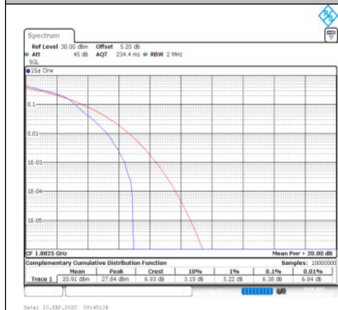
Band25-1.4MHz-16QAM-26365-1RB#0-PASS
