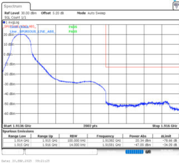
Band25-1.4MHz-QPSK-26683-1RB#0-PASS
