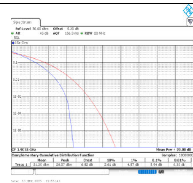
Band25-15MHz-QPSK-26615-75RB#0-PASS
