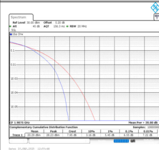
Band25-15MHz-16QAM-26615-75RB#0-PASS
