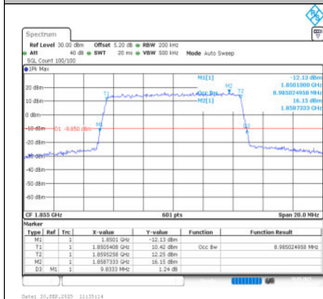
Band25-10MHz-QPSK-26090-50RB#0-PASS
