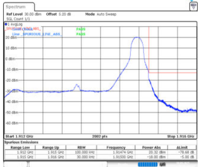
Band25-3MHz-QPSK-26675-1RB#14-PASS
