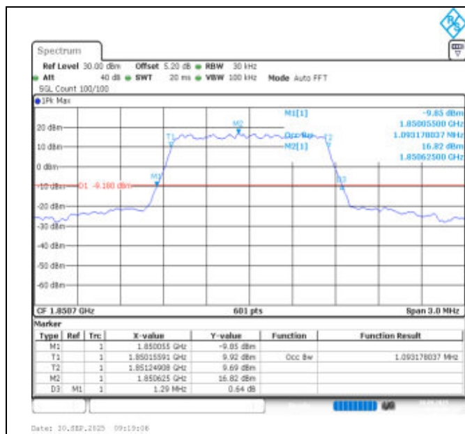
Band25-1.4MHz-QPSK-26047-6RB#0-PASS
