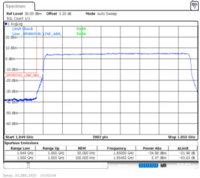
Band25-5MHz-16QAM-26065-25RB#0-PASS
