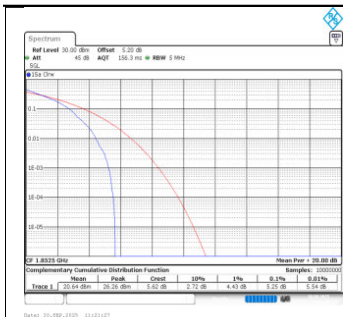
Band25-5MHz-QPSK-26065-1RB#0-PASS
