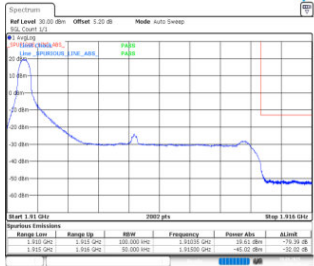
Band25-5MHz-16QAM-26665-1RB#0-PASS
