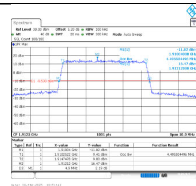
Band25-5MHz-16QAM-26665-25RB#0-PASS
