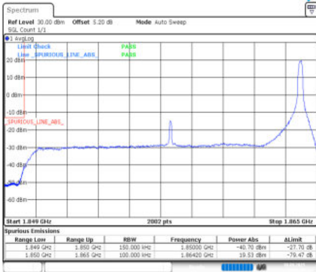
Band25-15MHz-16QAM-26115-1RB#74-PASS
