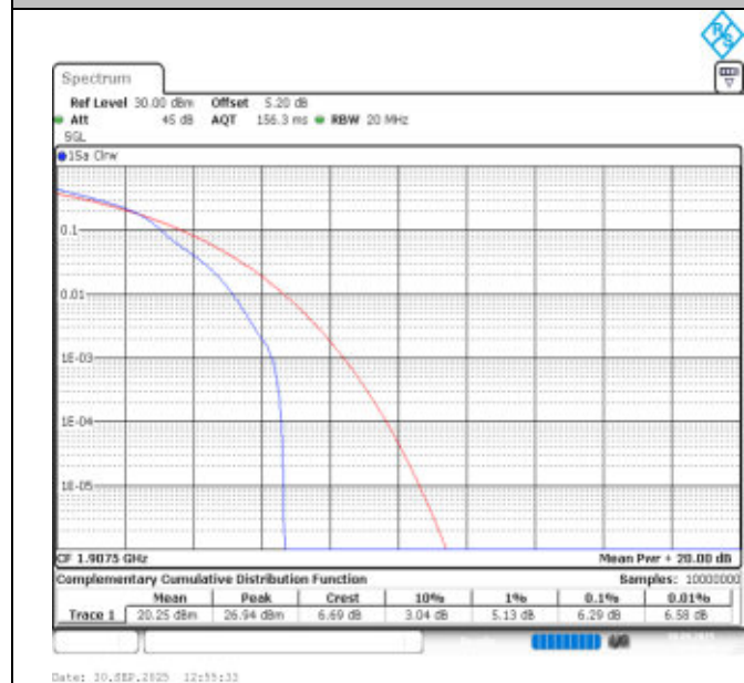
Band25-15MHz-16QAM-26615-1RB#0-PASS
