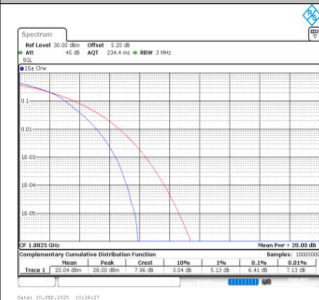
Band25-3MHz-16QAM-26365-15RB#0-PASS
