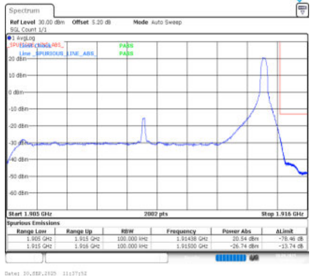
Band25-10MHz-QPSK-26640-1RB#49-PASS
