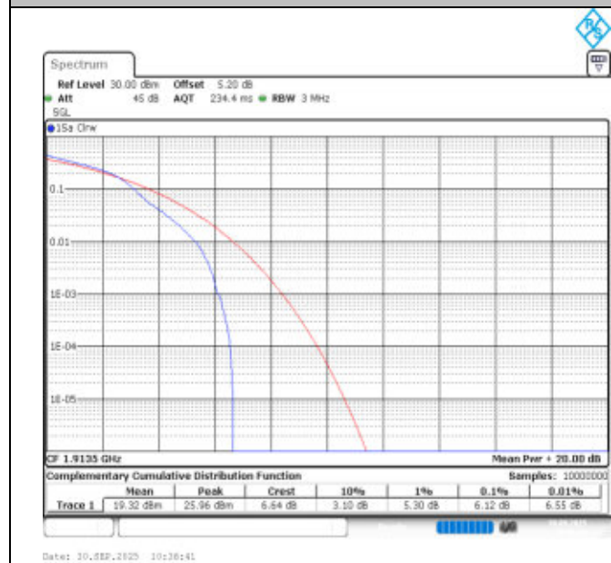
Band25-3MHz-16QAM-26675-1RB#0-PASS
