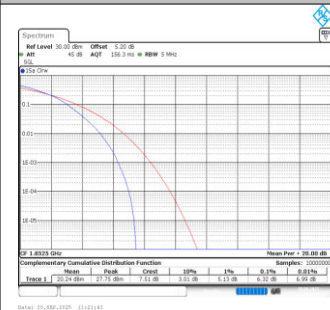
Band25-5MHz-16QAM-26065-25RB#0-PASS
