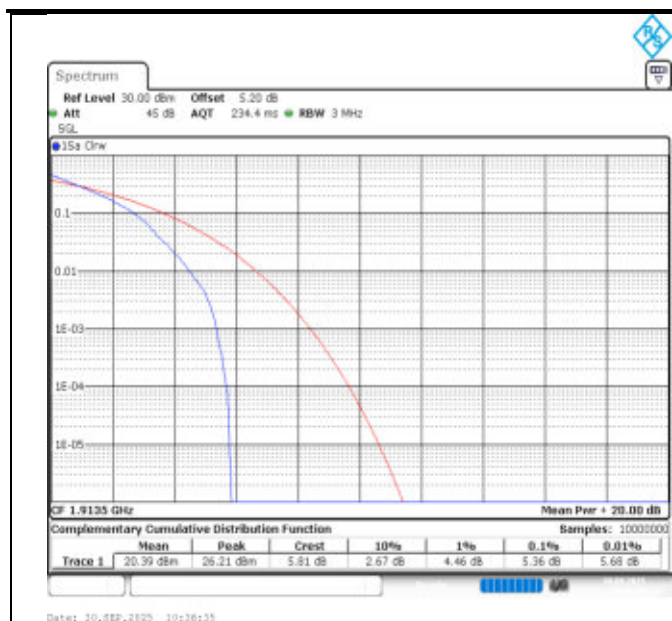
Band25-3MHz-QPSK-26675-1RB#0-PASS
