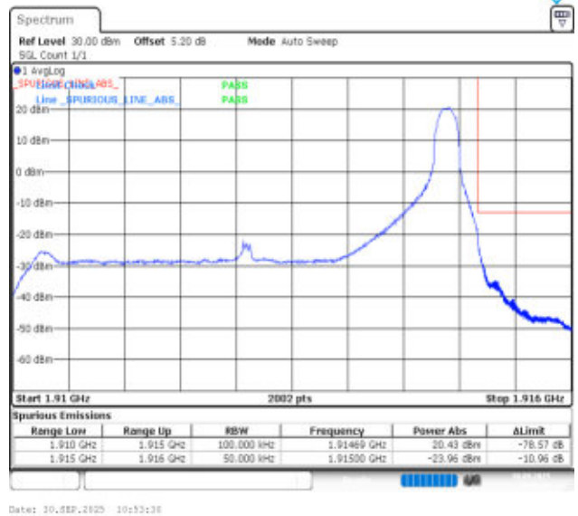
Band25-5MHz-QPSK-26665-1RB#24-PASS
