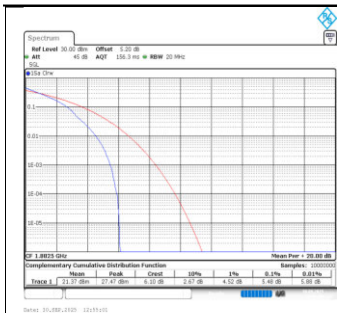
Band25-15MHz-QPSK-26365-1RB#0-PASS
