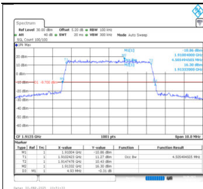
Band25-5MHz-QPSK-26665-25RB#0-PASS
