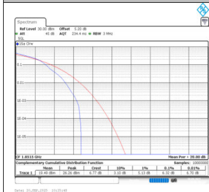
Band25-3MHz-16QAM-26055-1RB#0-PASS
