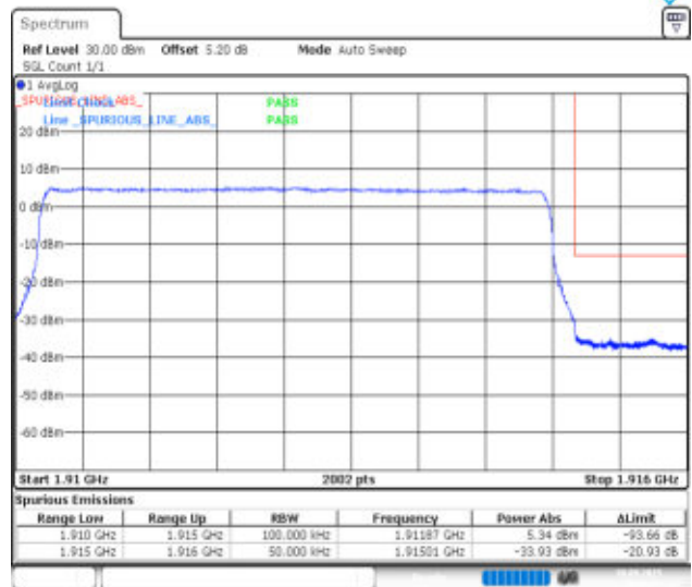
Band25-5MHz-16QAM-26665-25RB#0-PASS
