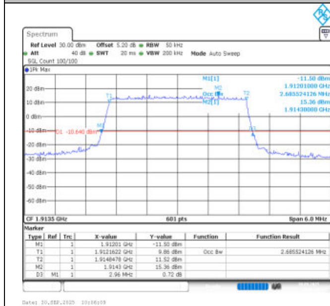
Band25-3MHz-QPSK-26675-15RB#0-PASS
