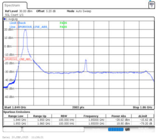
Band25-10MHz-16QAM-26090-1RB#0-PASS
