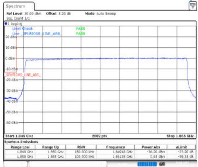
Band25-15MHz-16QAM-26115-75RB#0-PASS
