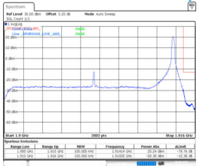
Band25-15MHz-QPSK-26615-1RB#74-PASS
