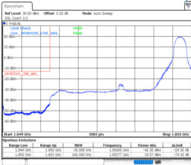
Band25-3MHz-16QAM-26055-1RB#14-PASS
