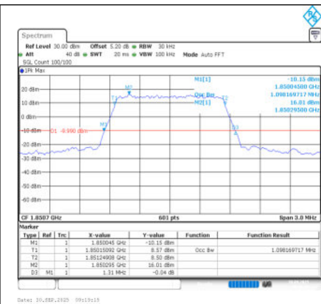
Band25-1.4MHz-16QAM-26047-6RB#0-PASS
