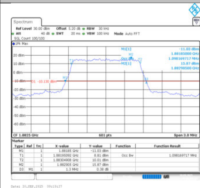
Band25-1.4MHz-16QAM-26365-6RB#0-PASS
