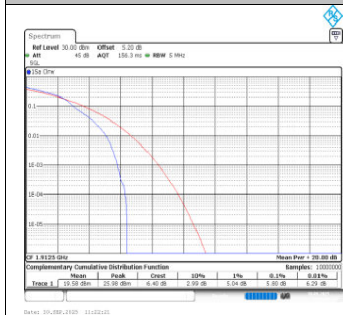
Band25-5MHz-16QAM-26665-1RB#0-PASS
