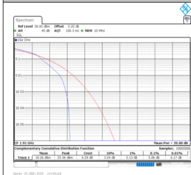
Band25-10MHz-16QAM-26640-1RB#0-PASS
