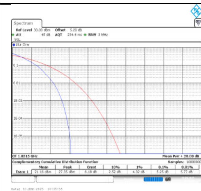
Band25-3MHz-QPSK-26055-15RB#0-PASS
