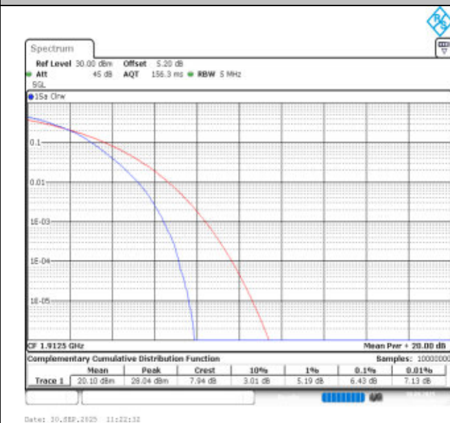
Band25-5MHz-16QAM-26665-25RB#0-PASS
