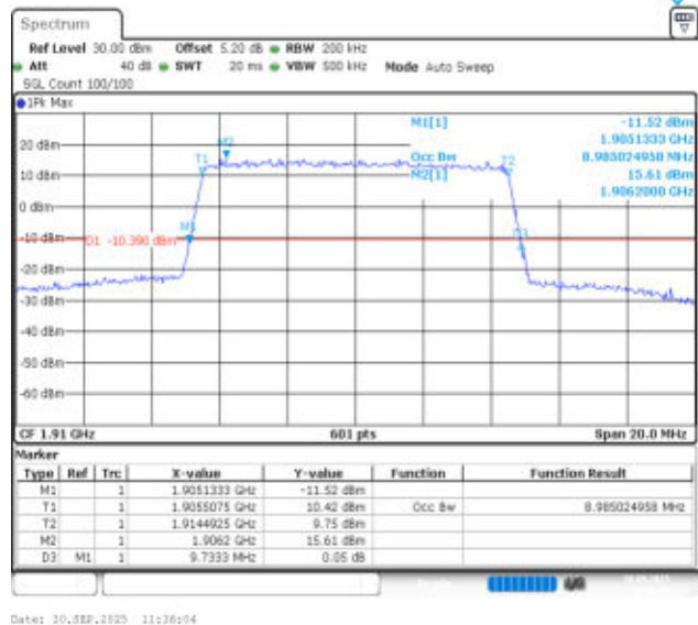
Band25-10MHz-16QAM-26640-50RB#0-PASS
