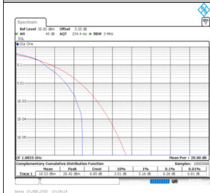
Band25-3MHz-16QAM-26365-1RB#0-PASS
