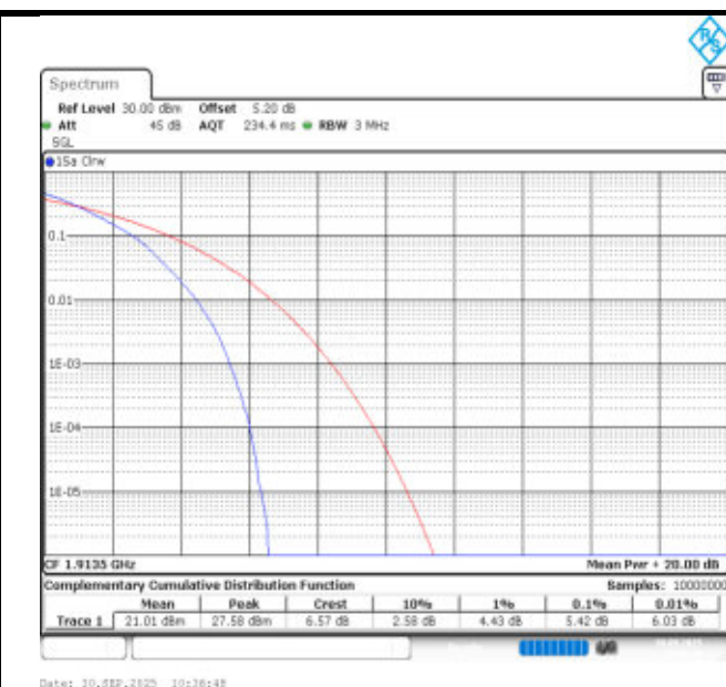
Band25-3MHz-QPSK-26675-15RB#0-PASS
