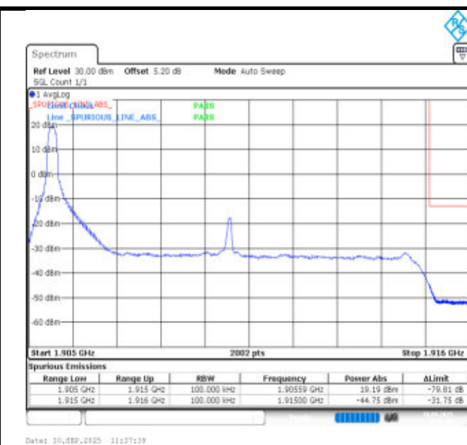
Band25-10MHz-16QAM-26640-1RB#0-PASS
