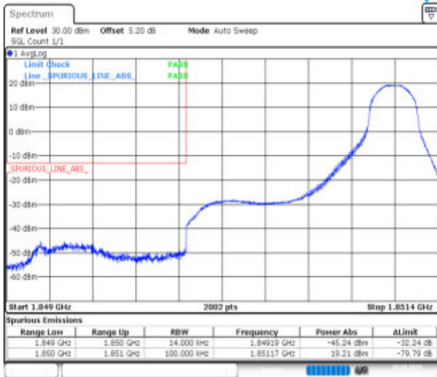
Band25-1.4MHz-16QAM-26047-1RB#5-PASS
