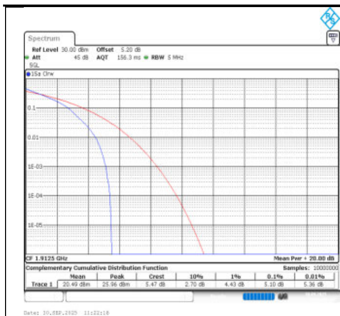
Band25-5MHz-QPSK-26665-1RB#0-PASS
