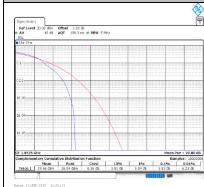
Band25-5MHz-16QAM-26065-1RB#0-PASS
