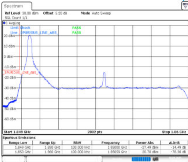
Band25-10MHz-QPSK-26090-1RB#0-PASS
