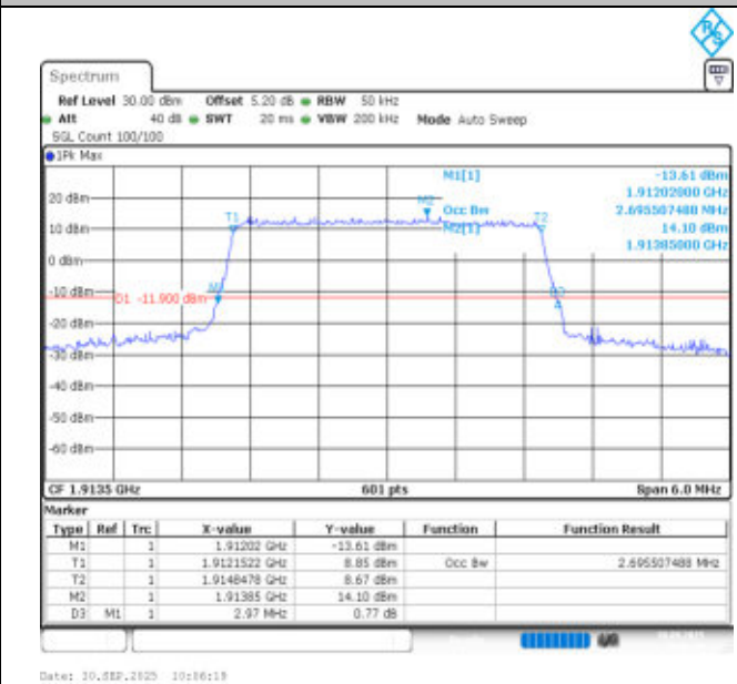
Band25-3MHz-16QAM-26675-15RB#0-PASS
