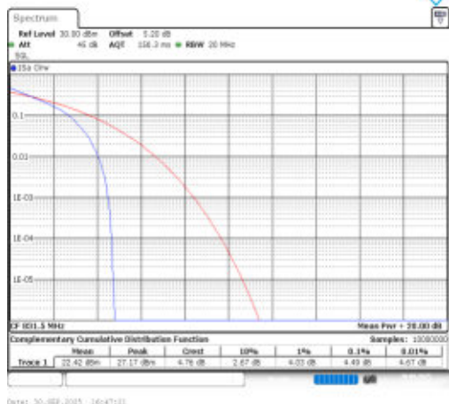
Band26(824-849)-15MHz-QPSK-26865-1RB#0-PASS
