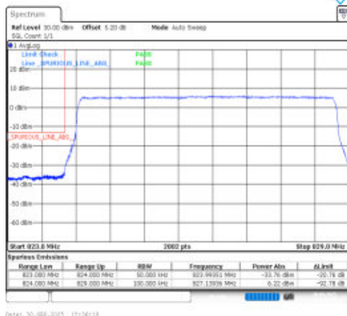
Band26(824-849)-5MHz-16QAM-26815-25RB#0-PASS
