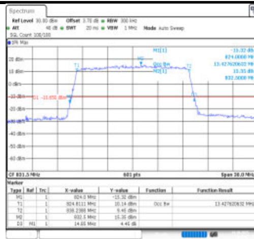
Band26(824-849)-15MHz-64QAM-26865-75RB#0-PASS
