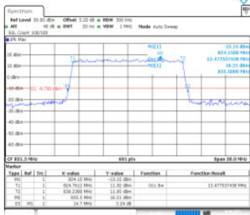
Band26(824-849)-15MHz-16QAM-26865-75RB#0-PASS
