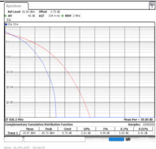
Band26(824-849)-1.4MHz-64QAM-26915-6RB#0-PASS
