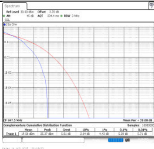
Band26(824-849)-3MHz-64QAM-27025-1RB#0-PASS
