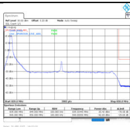
Band26(824-849)-10MHz-16QAM-26990-1RB#0-PASS
