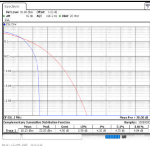
Band26(824-849)-15MHz-256QAM-26865-1RB#0-PASS
