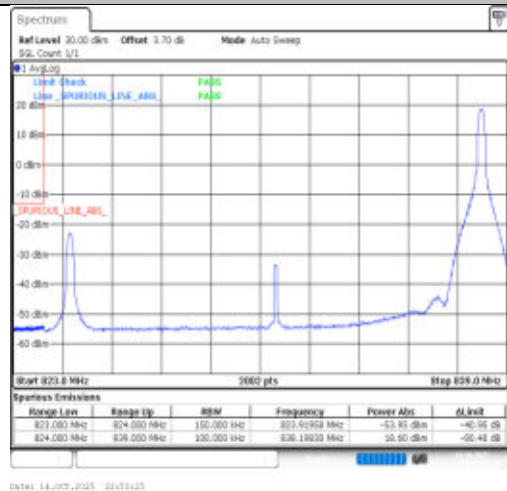
Band26(824-849)-15MHz-64QAM-26865-1RB#74-PASS
