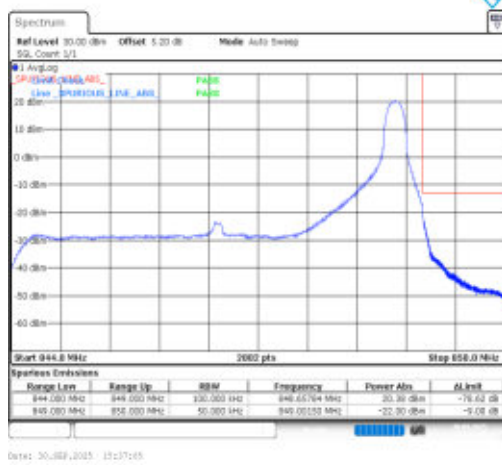
Band26(824-849)-5MHz-16QAM-27015-1RB#24-PASS
