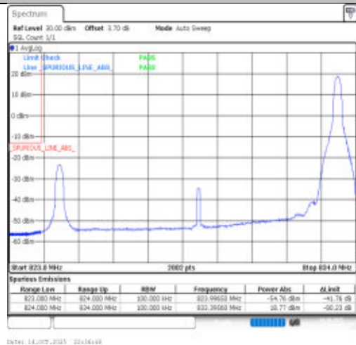
Band26(824-849)-10MHz-64QAM-26840-1RB#49-PASS
