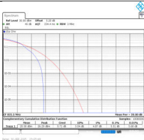
Band26(824-849)-3MHz-16QAM-26805-1RB#0-PASS
