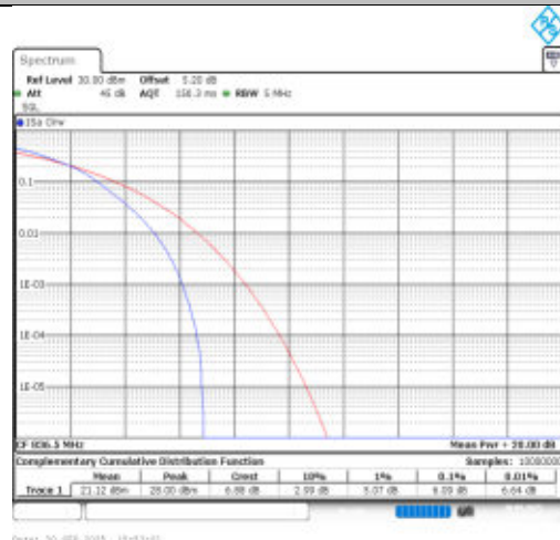
Band26(824-849)-5MHz-16QAM-26915-25RB#0-PASS
