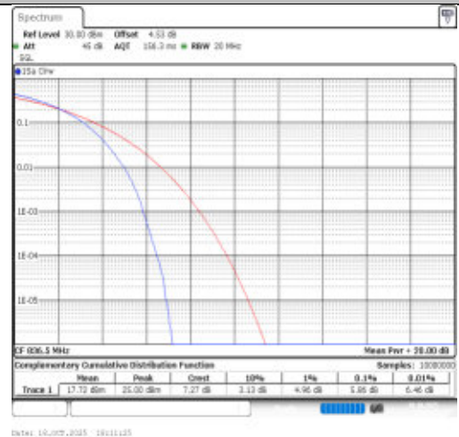
Band26(824-849)-15MHz-256QAM-26915-75RB#0-PASS
