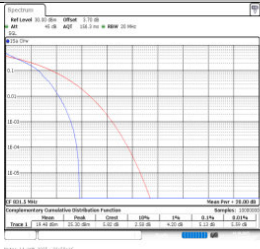
Band26(824-849)-15MHz-64QAM-26865-1RB#0-PASS
