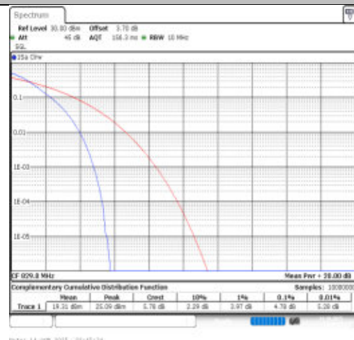
Band26(824-849)-10MHz-64QAM-26840-50RB#0-PASS
