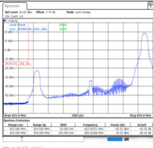
Band26(824-849)-5MHz-64QAM-26815-1RB#24-PASS
