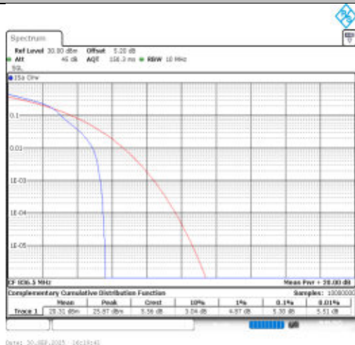
Band26(824-849)-10MHz-16QAM-26915-1RB#0-PASS
