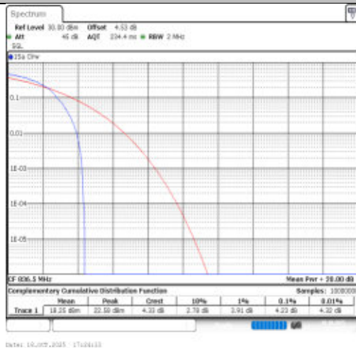
Band26(824-849)-1.4MHz-256QAM-26915-1RB#0-PASS
