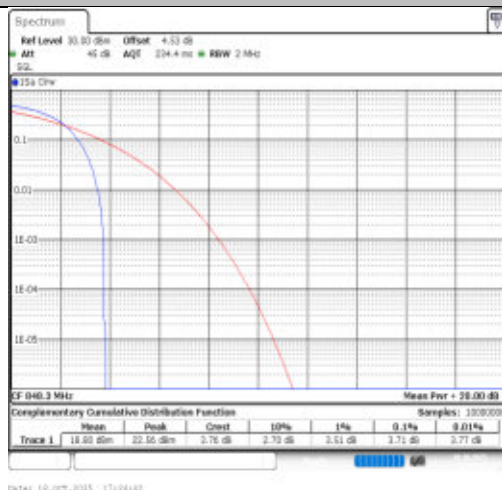
Band26(824-849)-1.4MHz-256QAM-27033-1RB#0-PASS
