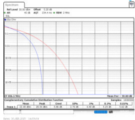
Band26(824-849)-1.4MHz-QPSK-26915-6RB#0-PASS
