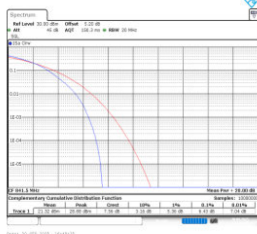
Band26(824-849)-15MHz-16QAM-26965-75RB#0-PASS
