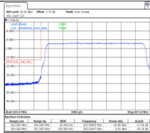
Band26(824-849)-3MHz-64QAM-26805-1RB#0-PASS
