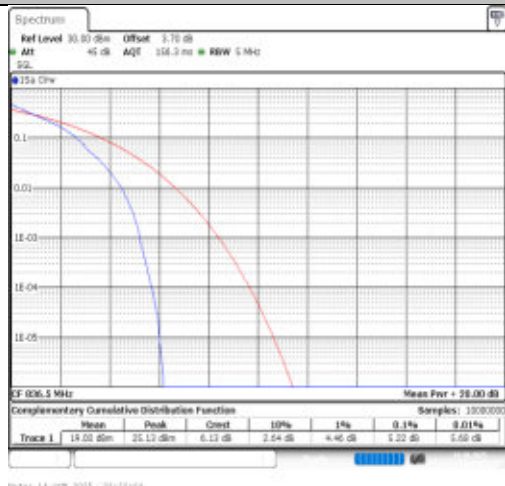
Band26(824-849)-5MHz-64QAM-26915-1RB#0-PASS
