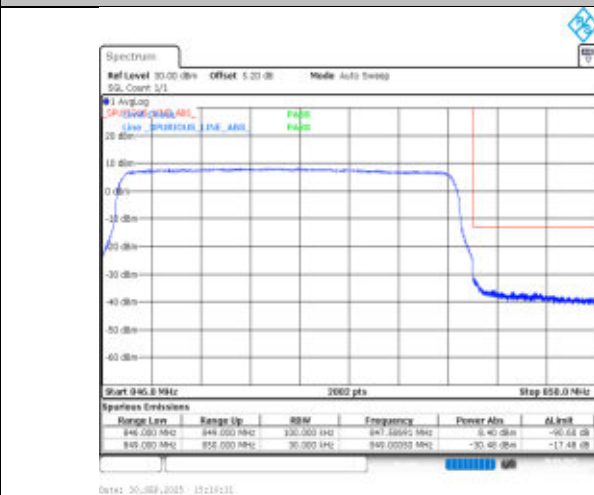
Band26(824-849)-3MHz-16QAM-27025-15RB#0-PASS
