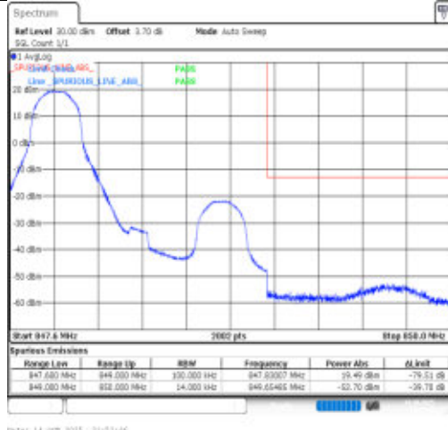
Band26(824-849)-1.4MHz-64QAM-27033-1RB#0-PASS
