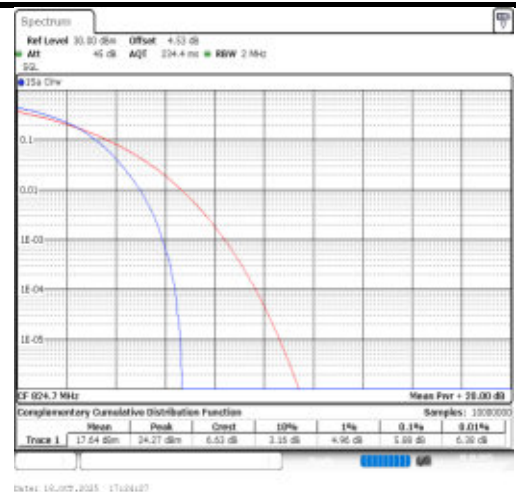
Band26(824-849)-1.4MHz-256QAM-26797-6RB#0-PASS
