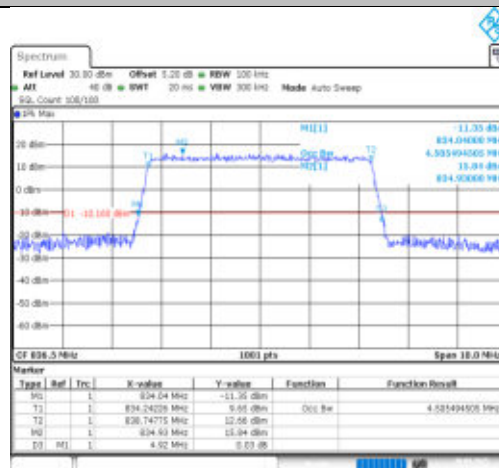
Band26(824-849)-5MHz-QPSK-26915-25RB#0-PASS
