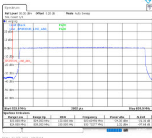
Band26(824-849)-15MHz-16QAM-26865-75RB#0-PASS
