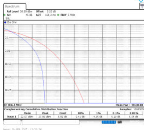
Band26(824-849)-5MHz-QPSK-26915-25RB#0-PASS
