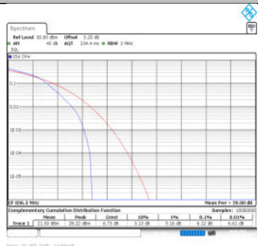
Band26(824-849)-1.4MHz-16QAM-26915-6RB#0-PASS
