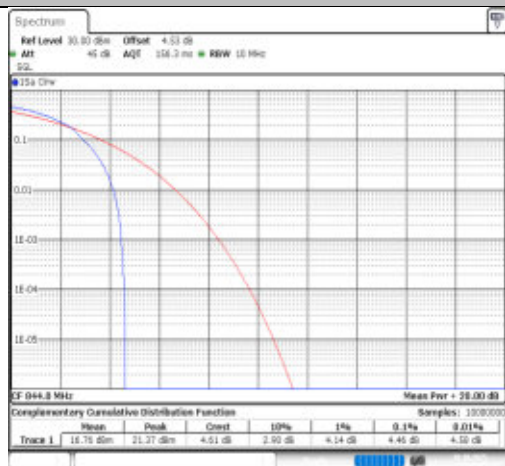
Band26(824-849)-10MHz-256QAM-26915-1RB#0-PASS
