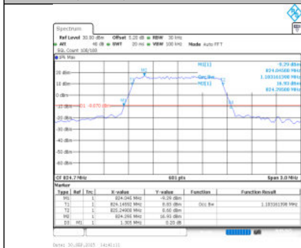
Band26(824-849)-1.4MHz-16QAM-26797-6RB#0-PASS
