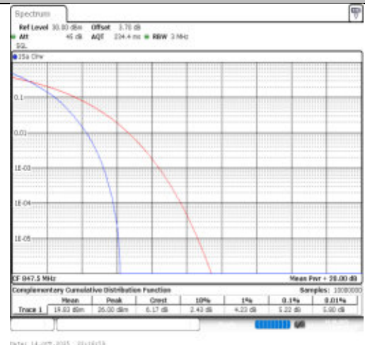
Band26(824-849)-3MHz-64QAM-27025-15RB#0-PASS
