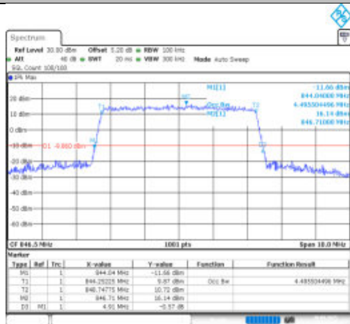
Band26(824-849)-5MHz-QPSK-27015-25RB#0-PASS
