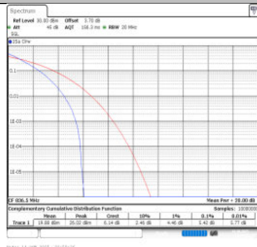
Band26(824-849)-15MHz-64QAM-26915-75RB#0-PASS
