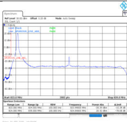
Band26(824-849)-15MHz-16QAM-26865-1RB#0-PASS
