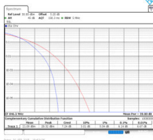
Band26(824-849)-5MHz-16QAM-27015-25RB#0-PASS
