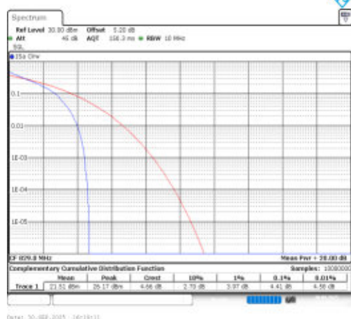
Band26(824-849)-10MHz-QPSK-26840-1RB#0-PASS
