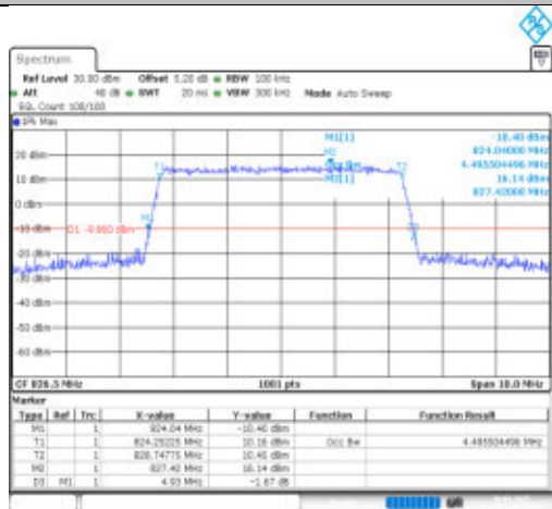
Band26(824-849)-5MHz-QPSK-26815-25RB#0-PASS
