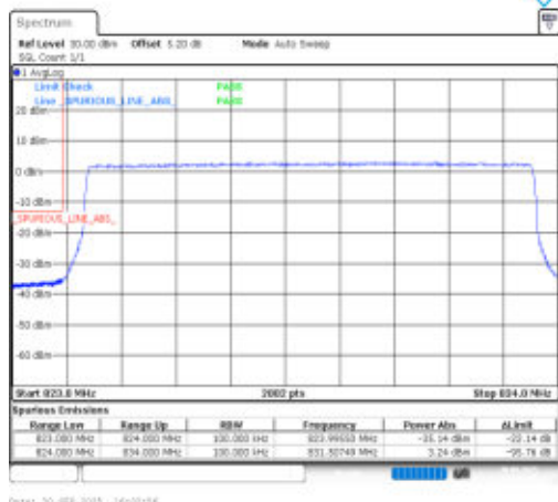
Band26(824-849)-10MHz-16QAM-26840-50RB#0-PASS
