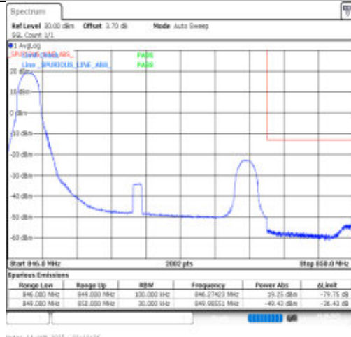
Band26(824-849)-3MHz-64QAM-27025-1RB#0-PASS
