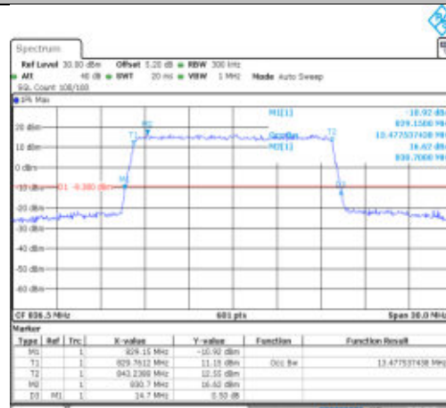
Band26(824-849)-15MHz-QPSK-26915-75RB#0-PASS
