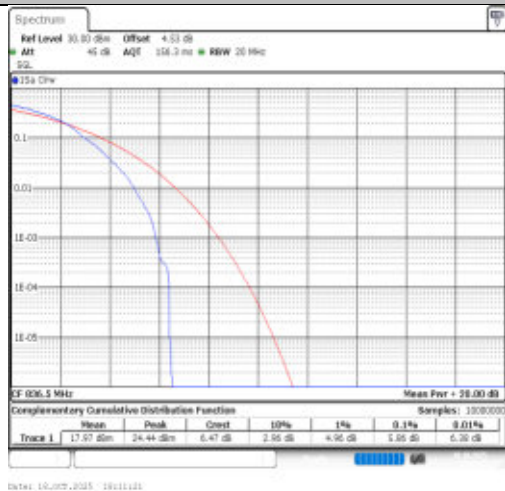
Band26(824-849)-15MHz-256QAM-26915-1RB#0-PASS
