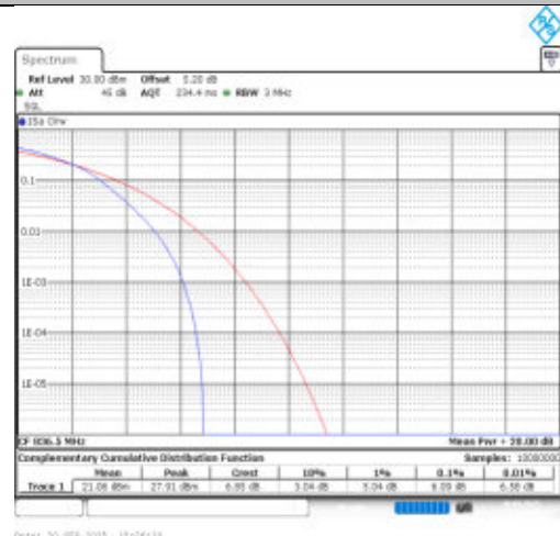
Band26(824-849)-3MHz-16QAM-26915-15RB#0-PASS
