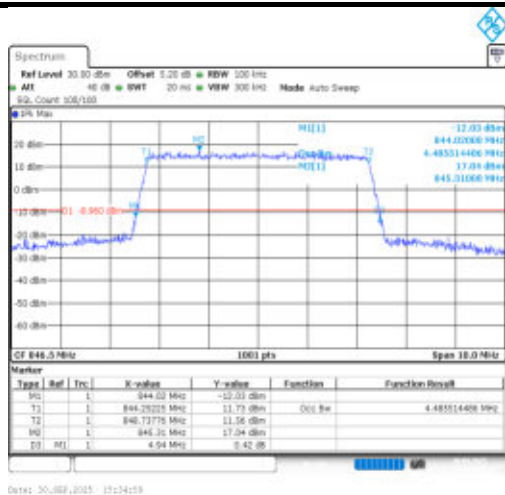
Band26(824-849)-5MHz-QPSK-27015-25RB#0-PASS
