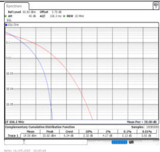
Band26(824-849)-10MHz-64QAM-26915-50RB#0-PASS
