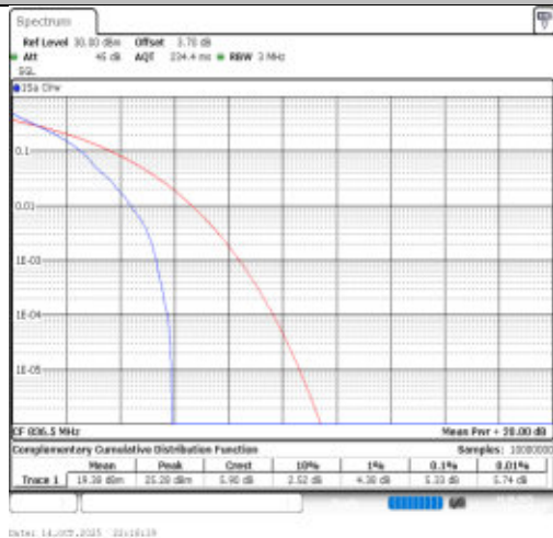
Band26(824-849)-3MHz-64QAM-26915-1RB#0-PASS
