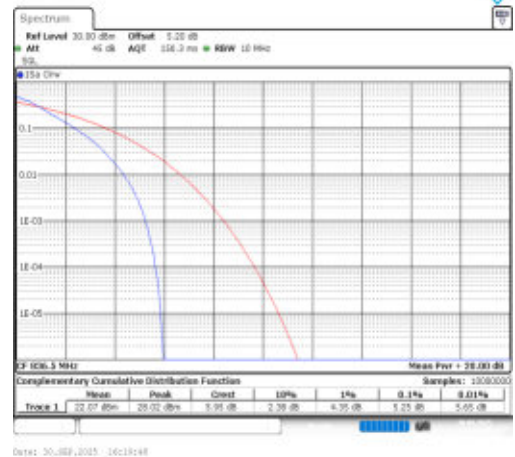
Band26(824-849)-10MHz-QPSK-26915-50RB#0-PASS
