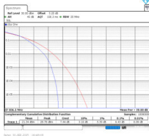
Band26(824-849)-15MHz-16QAM-26915-75RB#0-PASS
