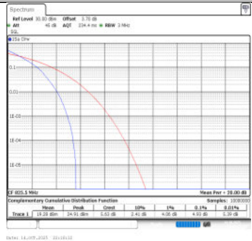
Band26(824-849)-3MHz-64QAM-26805-15RB#0-PASS
