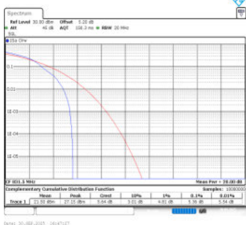
Band26(824-849)-15MHz-16QAM-26865-1RB#0-PASS
