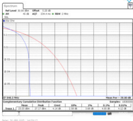
Band26(824-849)-1.4MHz-QPSK-27033-1RB#0-PASS
