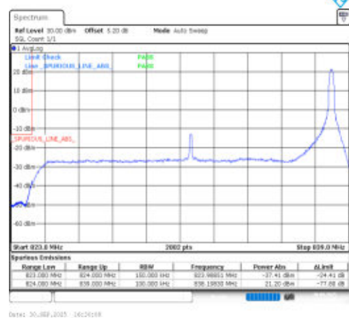
Band26(824-849)-15MHz-QPSK-26865-1RB#74-PASS
