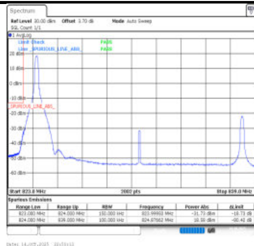
Band26(824-849)-15MHz-64QAM-26865-1RB#0-PASS
