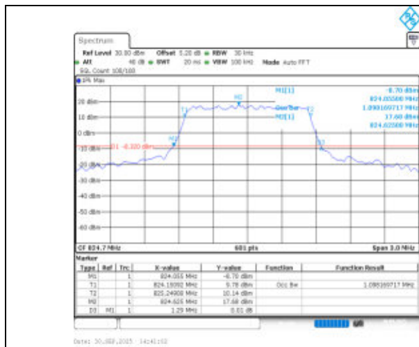
Band26(824-849)-1.4MHz-QPSK-26797-6RB#0-PASS
