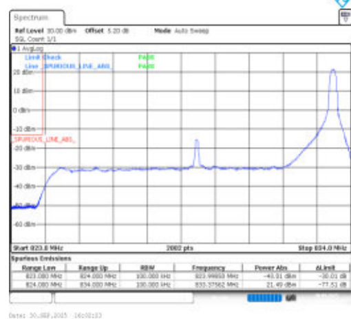
Band26(824-849)-10MHz-QPSK-26840-1RB#49-PASS
