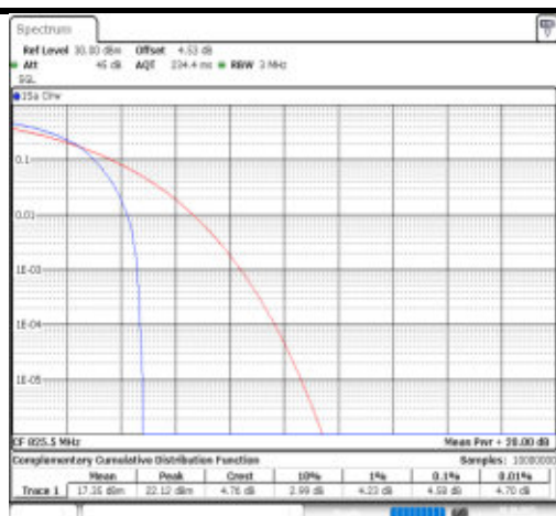
Band26(824-849)-3MHz-256QAM-26805-1RB#0-PASS
