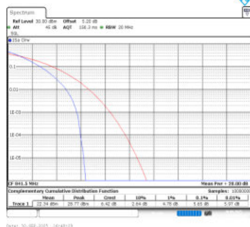
Band26(824-849)-15MHz-QPSK-26965-75RB#0-PASS
