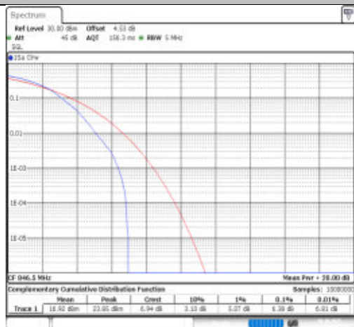
Band26(824-849)-5MHz-256QAM-26915-1RB#0-PASS
