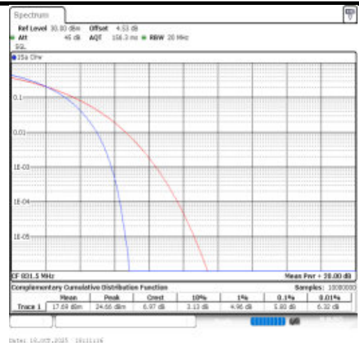
Band26(824-849)-15MHz-256QAM-26865-75RB#0-PASS
