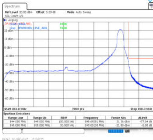
Band26(824-849)-5MHz-QPSK-27015-1RB#24-PASS
