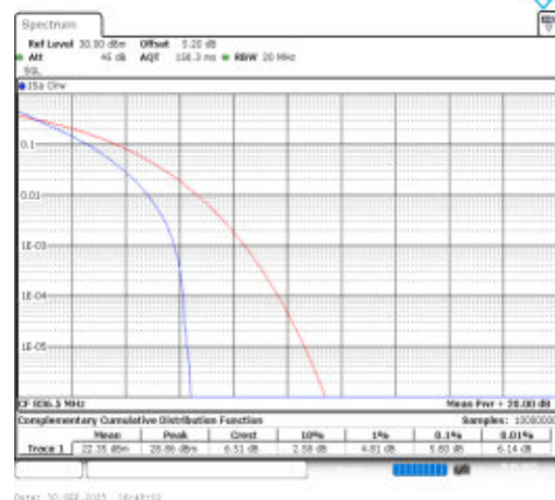
Band26(824-849)-15MHz-QPSK-26915-75RB#0-PASS
