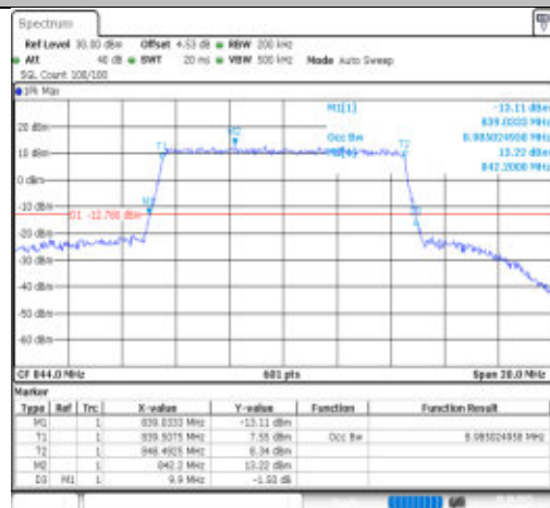
Band26(824-849)-10MHz-256QAM-26840-50RB#0-PASS
