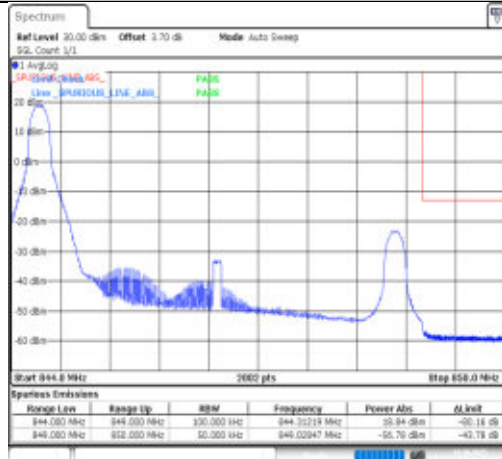
Band26(824-849)-5MHz-QPSK-27015-1RB#24-PASS
