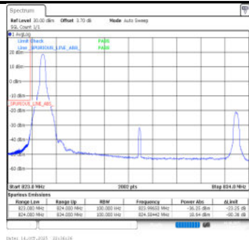
Band26(824-849)-10MHz-64QAM-26840-1RB#0-PASS
