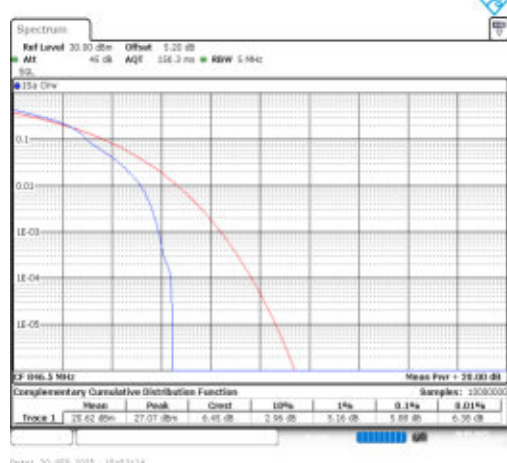
Band26(824-849)-5MHz-16QAM-27015-1RB#0-PASS
