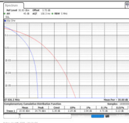
Band26(824-849)-5MHz-64QAM-26815-25RB#0-PASS
