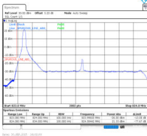
Band26(824-849)-10MHz-QPSK-26840-1RB#0-PASS
