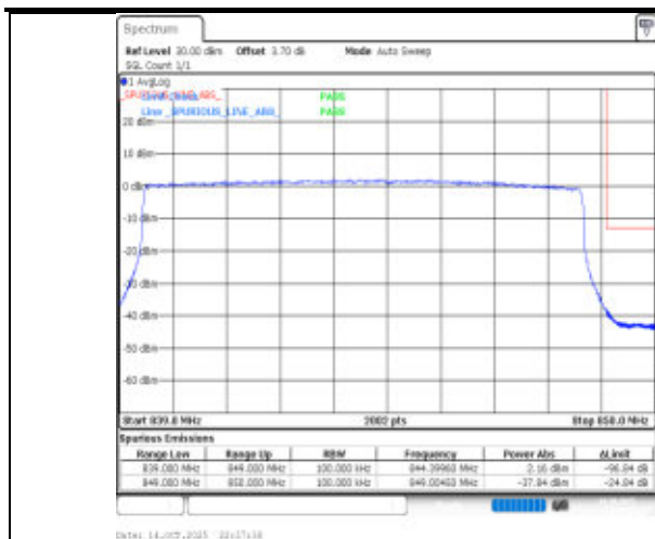
Band26(824-849)-10MHz-64QAM-26990-50RB#0-PASS
