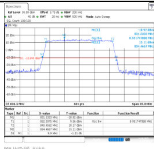
Band26(824-849)-10MHz-64QAM-26915-50RB#0-PASS
