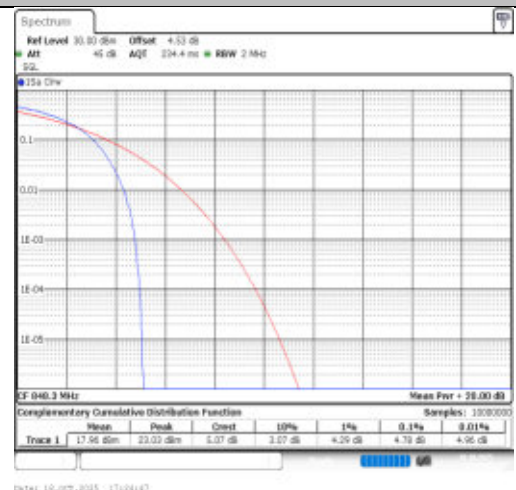
Band26(824-849)-1.4MHz-256QAM-27033-6RB#0-PASS
