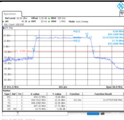
Band26(824-849)-15MHz-QPSK-26965-75RB#0-PASS
