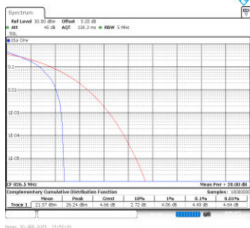
Band26(824-849)-5MHz-QPSK-26815-1RB#0-PASS
