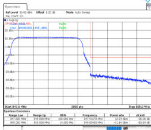
Band26(824-849)-1.4MHz-16QAM-27033-6RB#0-PASS
