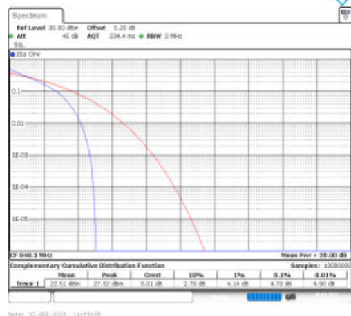
Band26(824-849)-1.4MHz-QPSK-27033-6RB#0-PASS
