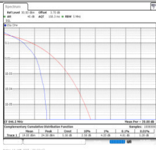
Band26(824-849)-5MHz-64QAM-27015-1RB#0-PASS
