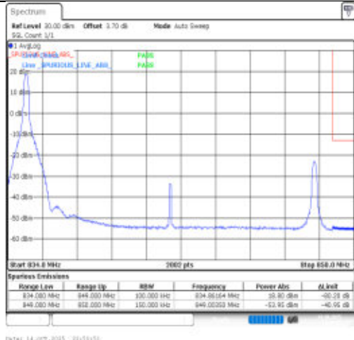
Band26(824-849)-15MHz-64QAM-26965-1RB#0-PASS
