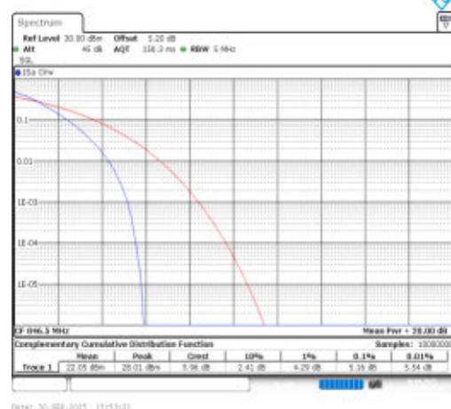
Band26(824-849)-5MHz-QPSK-27015-25RB#0-PASS
