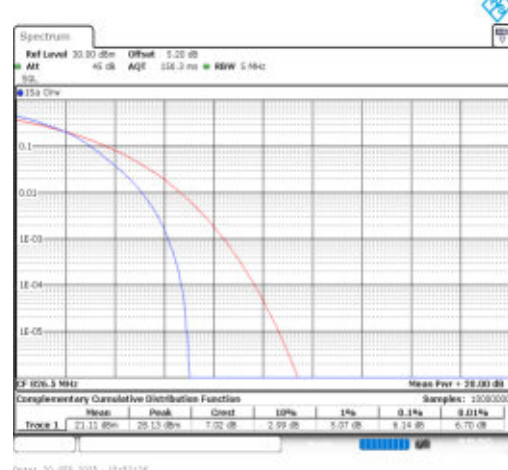
Band26(824-849)-5MHz-16QAM-26815-25RB#0-PASS
