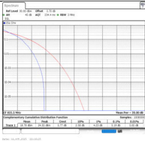
Band26(824-849)-3MHz-64QAM-26805-1RB#0-PASS
