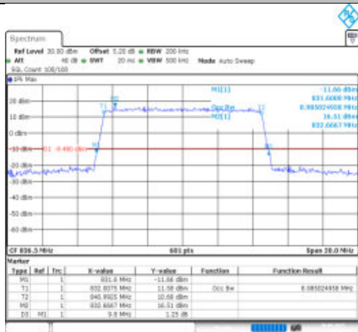
Band26(824-849)-10MHz-QPSK-26915-50RB#0-PASS
