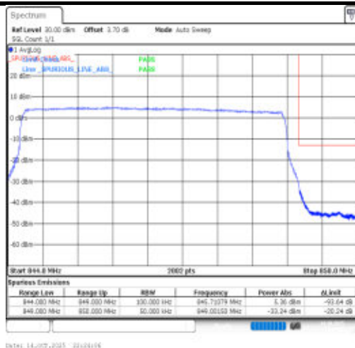
Band26(824-849)-5MHz-64QAM-27015-25RB#0-PASS
