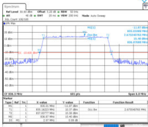
Band26(824-849)-3MHz-16QAM-26915-15RB#0-PASS
