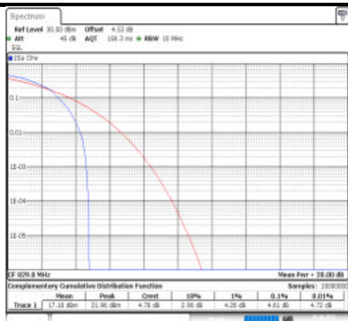
Band26(824-849)-10MHz-256QAM-26840-1RB#0-PASS
