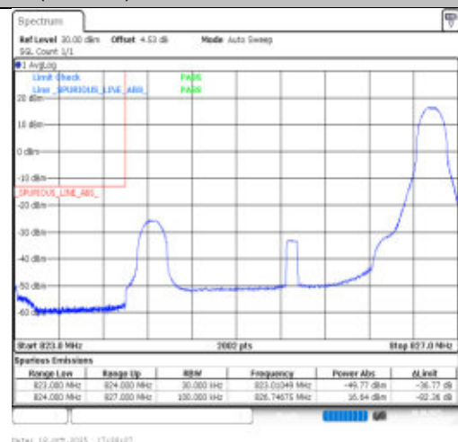
Band26(824-849)-3MHz-256QAM-26805-1RB#14-PASS
