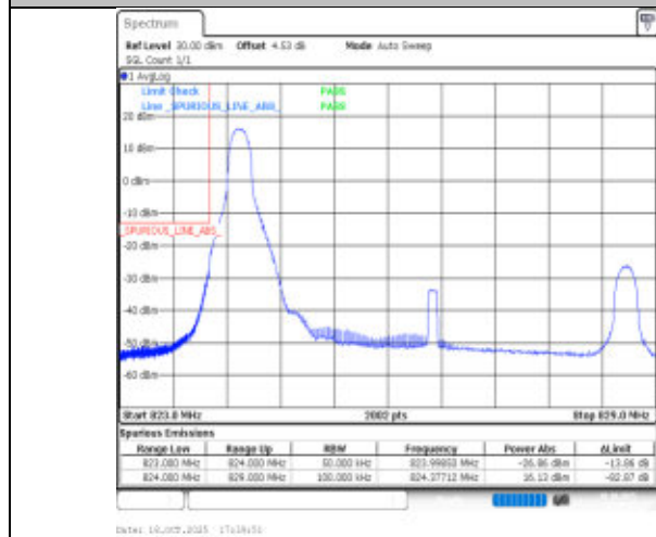
Band26(824-849)-5MHz-256QAM-26815-1RB#0-PASS
