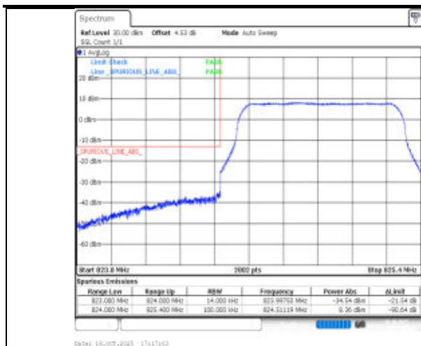
Band26(824-849)-1.4MHz-256QAM-26797-6RB#0-PASS
