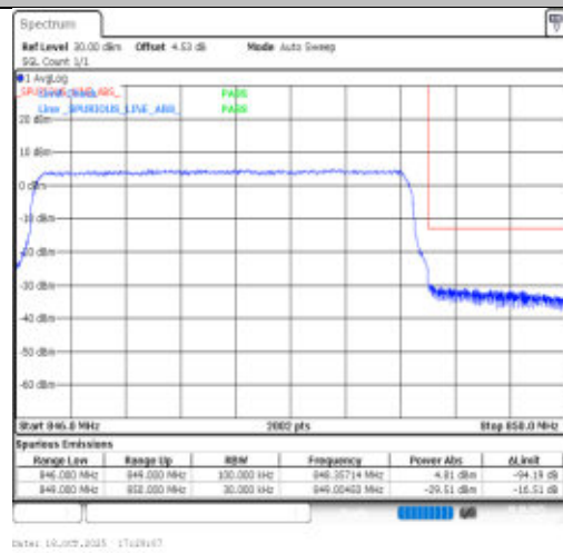
Band26(824-849)-3MHz-256QAM-27025-15RB#0-PASS
