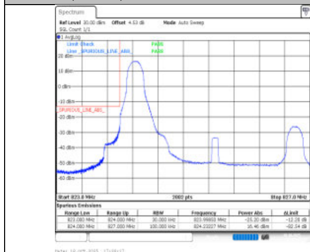
Band26(824-849)-3MHz-256QAM-26805-1RB#0-PASS
