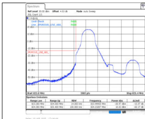
Band26(824-849)-1.4MHz-256QAM-26797-1RB#0-PASS
