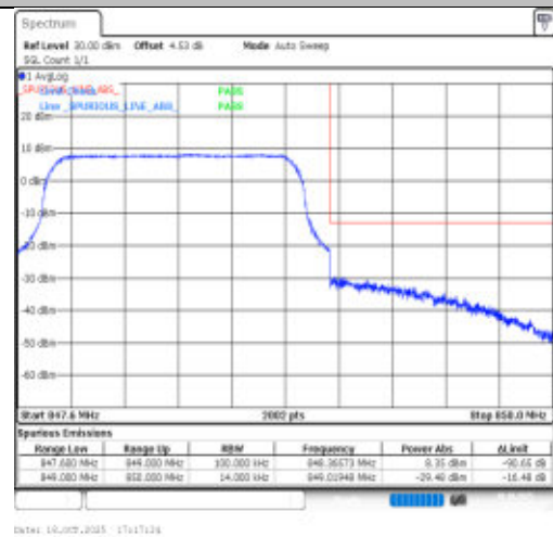
Band26(824-849)-1.4MHz-256QAM-27033-6RB#0-PASS
