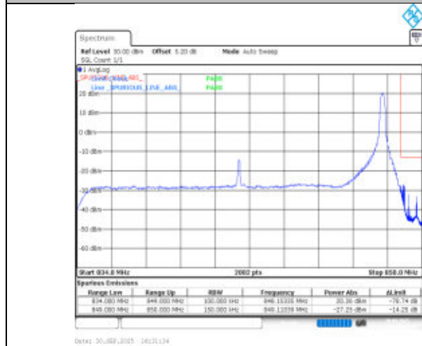
Band26(824-849)-15MHz-16QAM-26965-1RB#74-PASS
