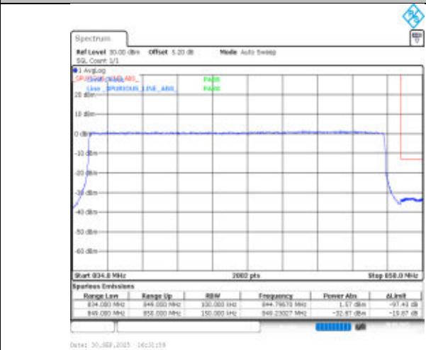
Band26(824-849)-15MHz-16QAM-26965-75RB#0-PASS
