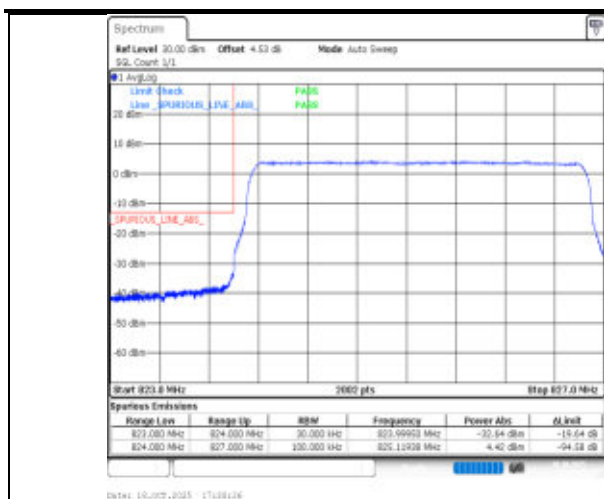
Band26(824-849)-3MHz-256QAM-26805-15RB#0-PASS
