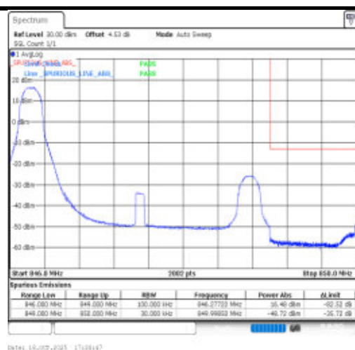
Band26(824-849)-3MHz-256QAM-27025-1RB#0-PASS
