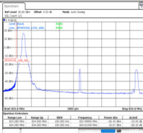
Band26(824-849)-5MHz-256QAM-27015-1RB#24-PASS
