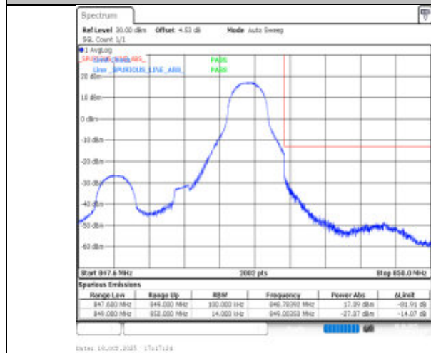
Band26(824-849)-1.4MHz-256QAM-27033-1RB#5-PASS
