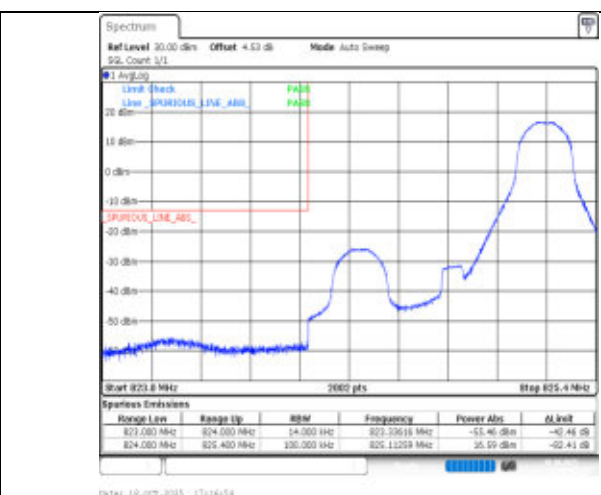
Band26(824-849)-1.4MHz-256QAM-26797-1RB#5-PASS
