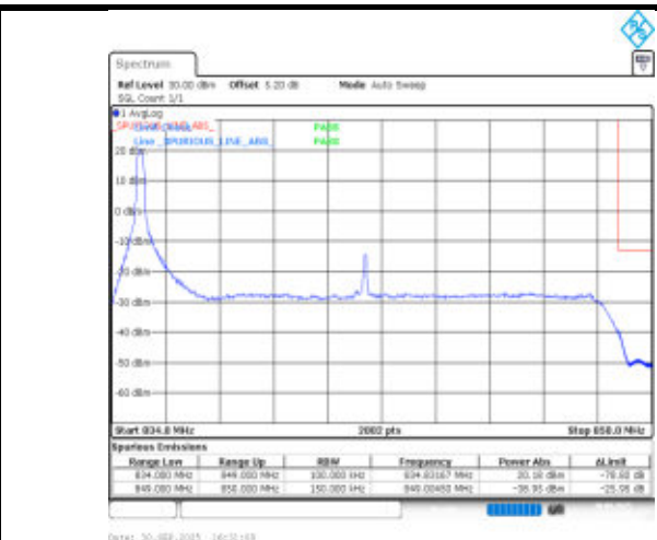
Band26(824-849)-15MHz-16QAM-26965-1RB#0-PASS
