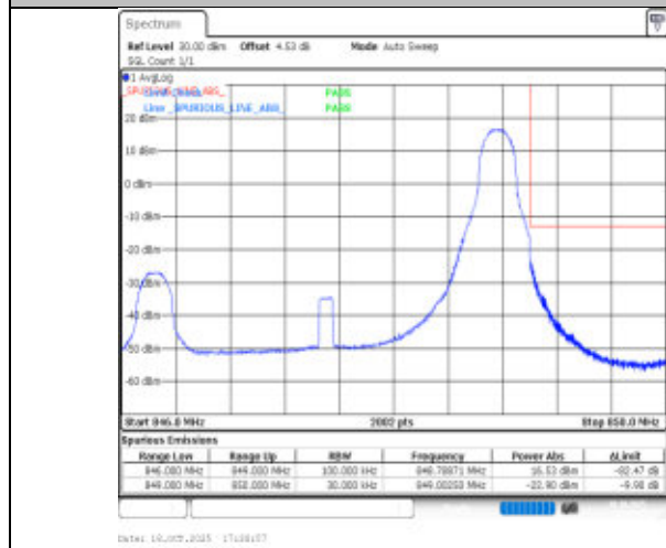
Band26(824-849)-3MHz-256QAM-27025-1RB#14-PASS
