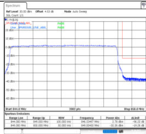
Band26(824-849)-5MHz-256QAM-27015-1RB#0-PASS
