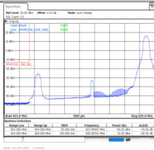
Band26(824-849)-5MHz-256QAM-26815-1RB#24-PASS
