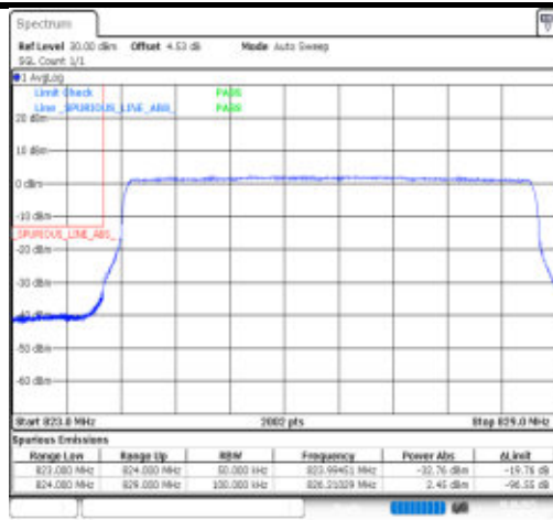
Band26(824-849)-5MHz-256QAM-26815-25RB#0-PASS
