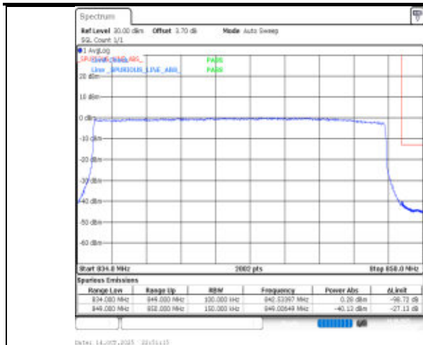
Band26(824-849)-15MHz-64QAM-26965-75RB#0-PASS
