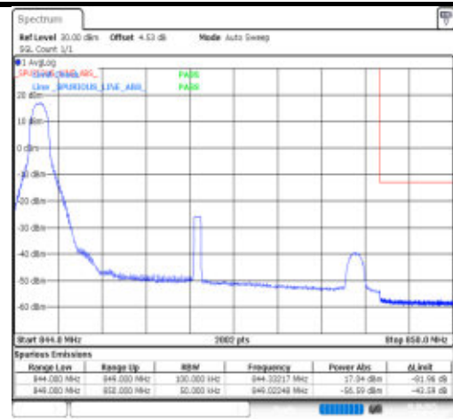
Band26(824-849)-5MHz-256QAM-27015-1RB#0-PASS
