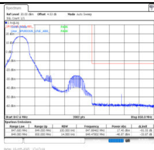
Band26(824-849)-1.4MHz-256QAM-27033-1RB#0-PASS
