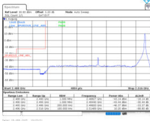
Band41-20MHz-16QAM-39750-1RB#99-PASS
