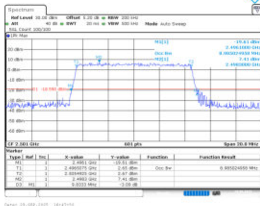
Band41-10MHz-16QAM-39700-50RB#0-PASS
