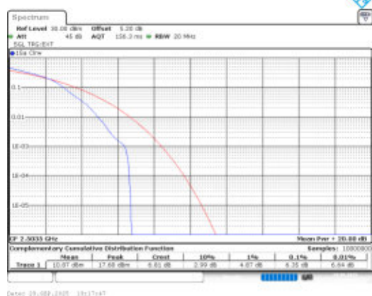
Band41-15MHz-16QAM-39725-1RB#0-PASS
