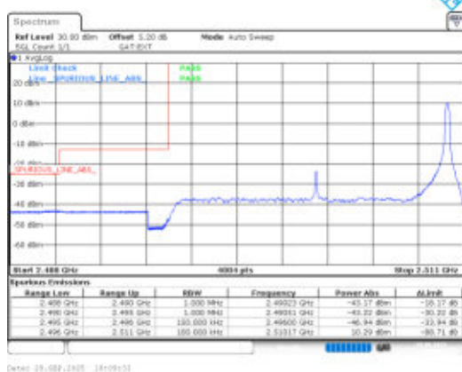
Band41-15MHz-16QAM-39725-1RB#74-PASS
