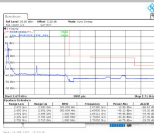
Band41-15MHz-16QAM-41515-1RB#0-PASS
