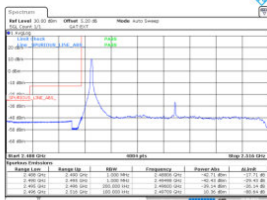
Band41-20MHz-16QAM-39750-1RB#0-PASS
