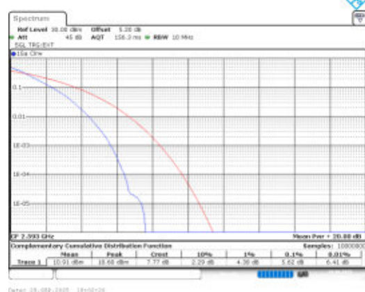
Band41-10MHz-QPSK-40620-50RB#0-PASS
