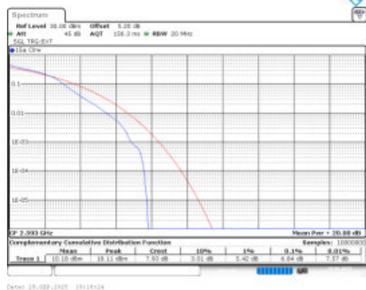
Band41-15MHz-16QAM-40620-1RB#0-PASS
