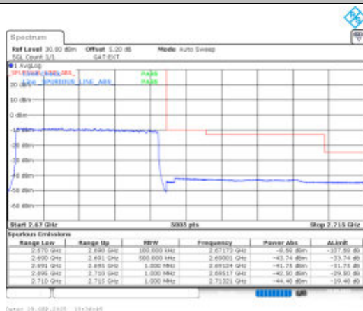
Band41-20MHz-QPSK-41490-100RB#0-PASS
