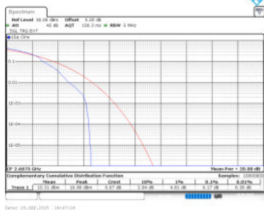
Band41-5MHz-16QAM-41565-1RB#0-PASS
