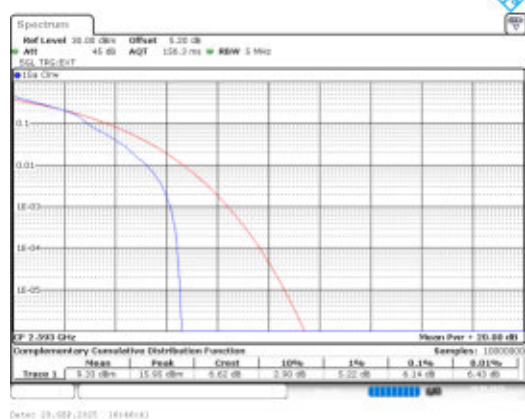
Band41-5MHz-16QAM-40620-1RB#0-PASS
