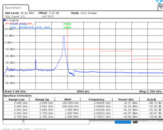
Band41-10MHz-16QAM-41540-1RB#49-PASS
