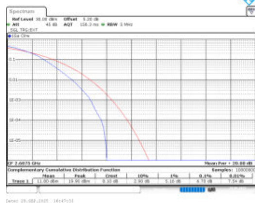
Band41-5MHz-16QAM-41565-25RB#0-PASS
