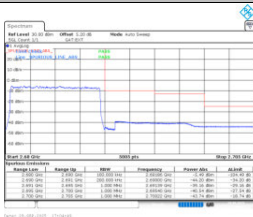
Band41-10MHz-QPSK-41540-50RB#0-PASS
