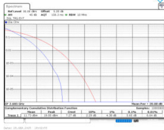
Band41-10MHz-QPSK-41540-50RB#0-PASS
