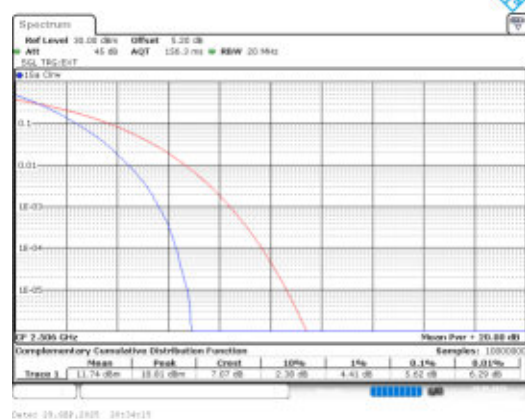
Band41-20MHz-QPSK-39750-100RB#0-PASS
