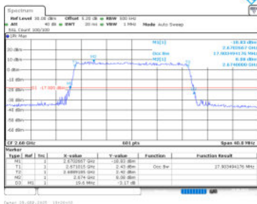
Band41-20MHz-QPSK-41490-100RB#0-PASS
