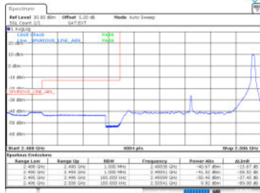
Band41-10MHz-QPSK-39700-1RB#49-PASS
