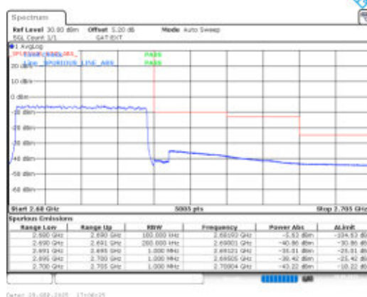
Band41-10MHz-16QAM-41540-50RB#0-PASS
