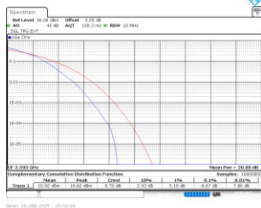
Band41-10MHz-16QAM-40620-50RB#0-PASS
