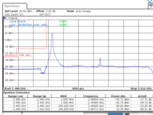
Band41-20MHz-QPSK-39750-1RB#0-PASS
