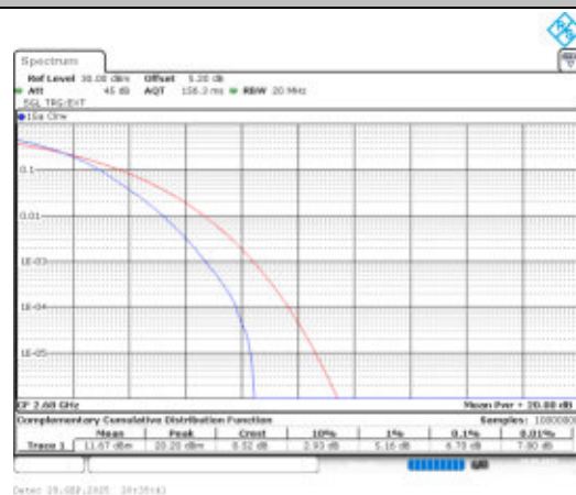
Band41-20MHz-16QAM-41490-100RB#0-PASS
