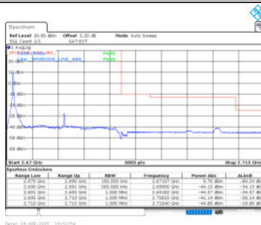
Band41-20MHz-16QAM-41490-1RB#0-PASS
