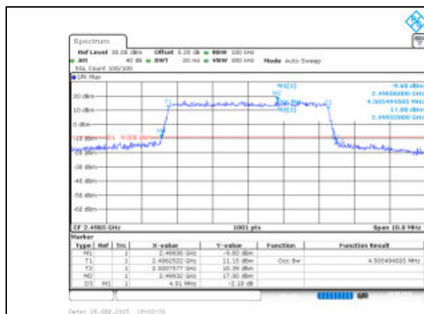
Band41-5MHz-QPSK-39675-25RB#0-PASS
