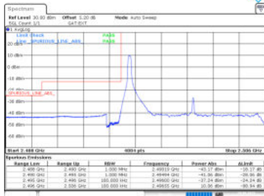
Band41-10MHz-QPSK-39700-1RB#0-PASS
