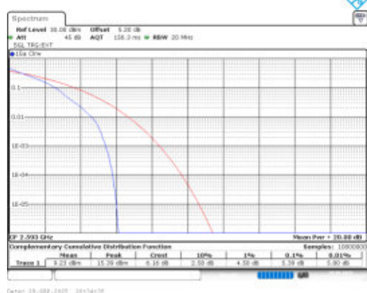
Band41-20MHz-QPSK-40620-1RB#0-PASS
