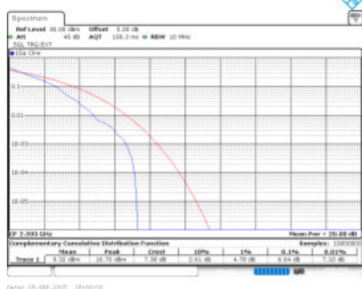
Band41-10MHz-QPSK-40620-1RB#0-PASS
