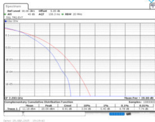
Band41-15MHz-16QAM-40620-75RB#0-PASS
