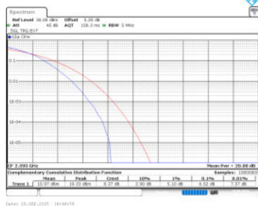
Band41-5MHz-16QAM-40620-25RB#0-PASS
