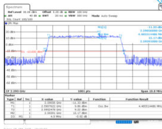
Band41-5MHz-16QAM-40620-25RB#0-PASS
