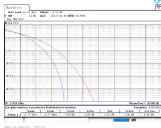
Band41-10MHz-16QAM-39700-50RB#0-PASS
