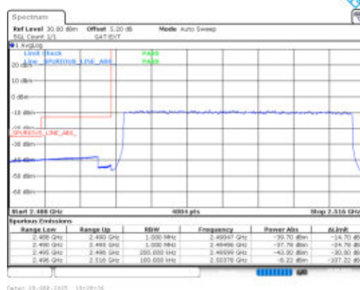
Band41-20MHz-16QAM-39750-100RB#0-PASS
