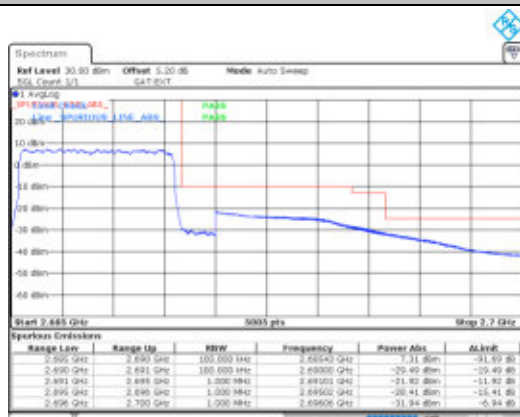
Band41-5MHz-QPSK-41565-1RB#0-PASS
