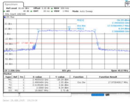
Band41-20MHz-16QAM-39750-100RB#0-PASS
