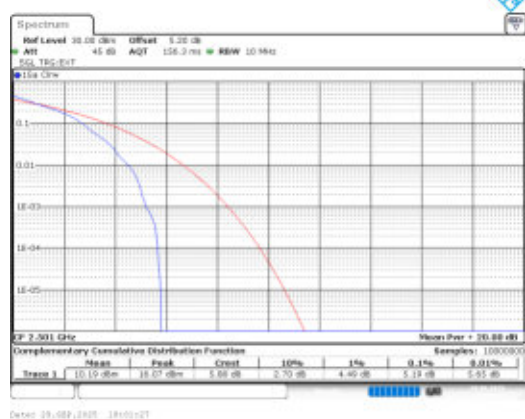
Band41-10MHz-QPSK-39700-1RB#0-PASS
