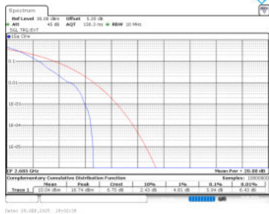
Band41-10MHz-QPSK-41540-1RB#0-PASS
