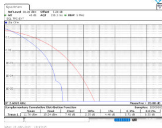
Band41-5MHz-QPSK-41565-25RB#0-PASS
