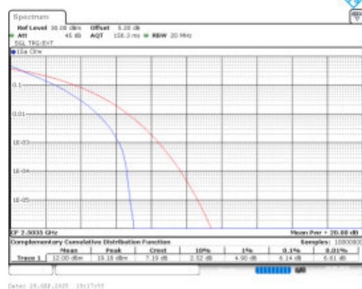
Band41-15MHz-QPSK-39725-75RB#0-PASS
