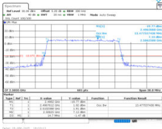
Band41-15MHz-QPSK-39725-75RB#0-PASS
