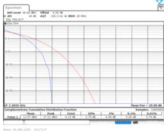
Band41-15MHz-QPSK-39725-1RB#0-PASS
