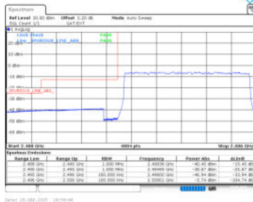
Band41-10MHz-16QAM-39700-50RB#0-PASS
