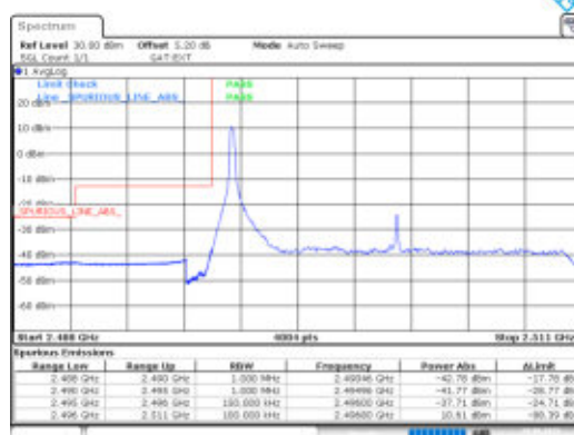
Band41-15MHz-16QAM-39725-1RB#0-PASS
