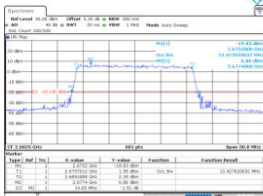
Band41-15MHz-QPSK-41515-75RB#0-PASS
