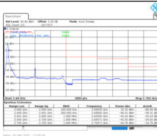
Band41-10MHz-16QAM-41540-1RB#0-PASS
