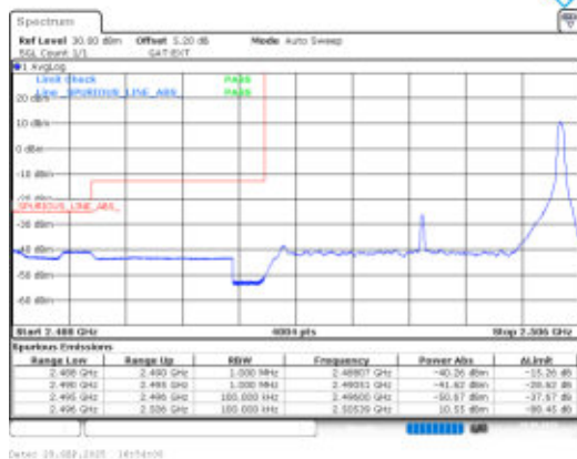
Band41-10MHz-16QAM-39700-1RB#49-PASS
