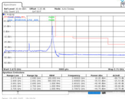
Band41-15MHz-16QAM-41515-1RB#74-PASS
