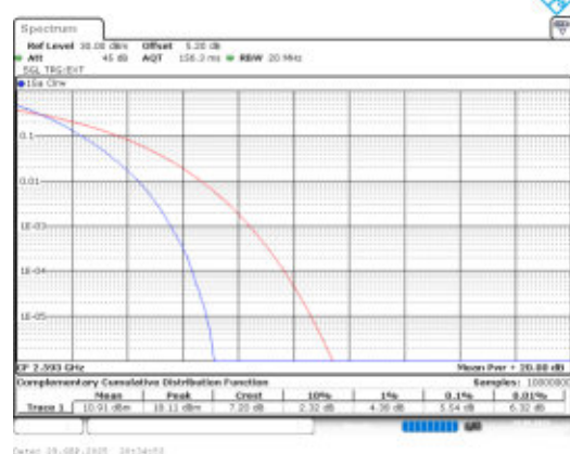
Band41-20MHz-QPSK-40620-100RB#0-PASS
