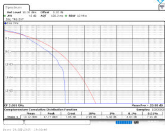
Band41-10MHz-16QAM-41540-1RB#0-PASS
