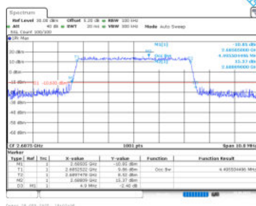
Band41-5MHz-16QAM-41565-25RB#0-PASS
