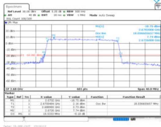
Band41-20MHz-16QAM-41490-100RB#0-PASS
