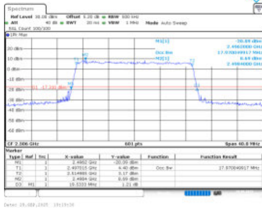
Band41-20MHz-QPSK-39750-100RB#0-PASS
