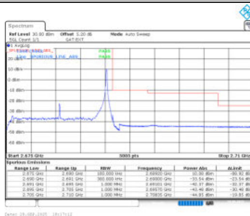
Band41-15MHz-QPSK-41515-1RB#74-PASS
