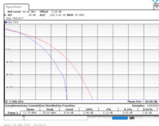
Band41-20MHz-16QAM-39750-100RB#0-PASS
