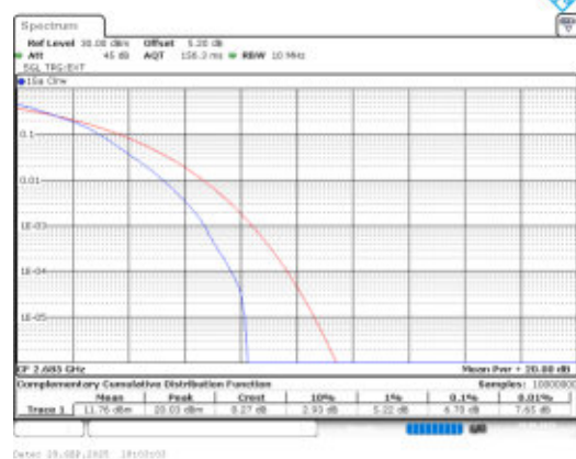
Band41-10MHz-16QAM-41540-50RB#0-PASS
