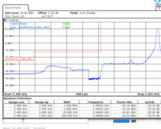
Band41-5MHz-16QAM-39675-1RB#24-PASS
