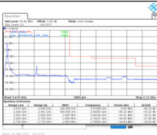
Band41-15MHz-QPSK-41515-1RB#0-PASS
