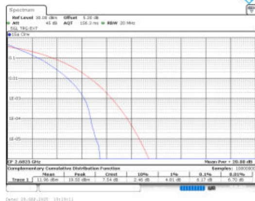
Band41-15MHz-QPSK-41515-75RB#0-PASS
