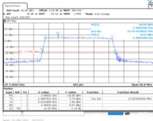
Band41-15MHz-16QAM-39725-75RB#0-PASS
