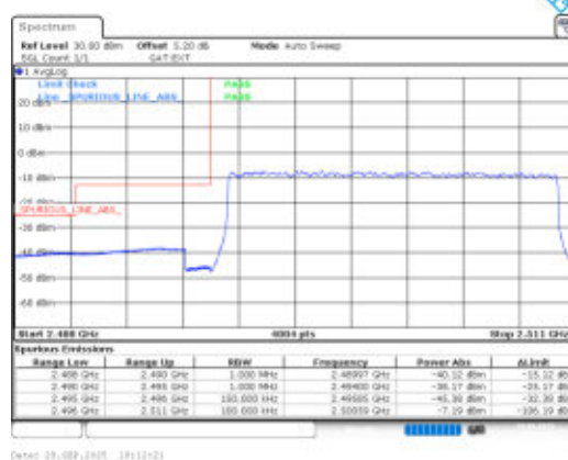
Band41-15MHz-16QAM-39725-75RB#0-PASS
