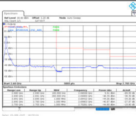
Band41-10MHz-QPSK-41540-1RB#0-PASS
