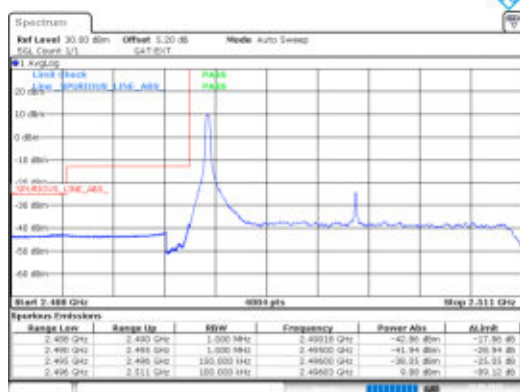
Band41-15MHz-QPSK-39725-1RB#0-PASS
