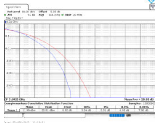
Band41-15MHz-16QAM-41515-75RB#0-PASS
