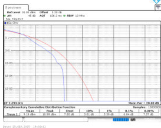
Band41-10MHz-16QAM-40620-1RB#0-PASS
