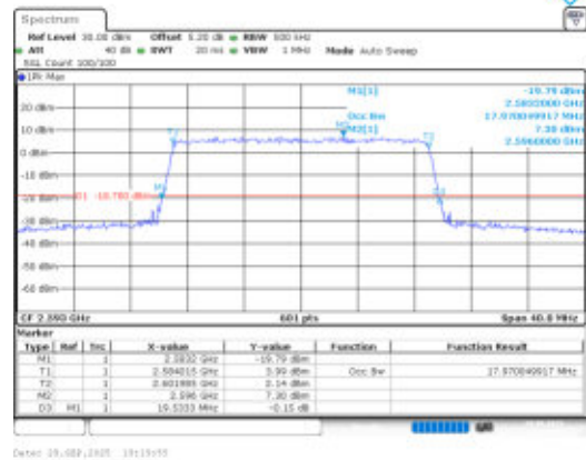
Band41-20MHz-16QAM-40620-100RB#0-PASS
