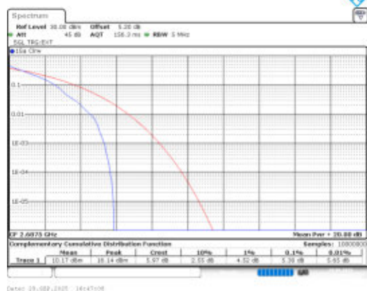
Band41-5MHz-QPSK-41565-1RB#0-PASS
