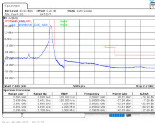
Band41-5MHz-16QAM-41565-1RB#24-PASS
