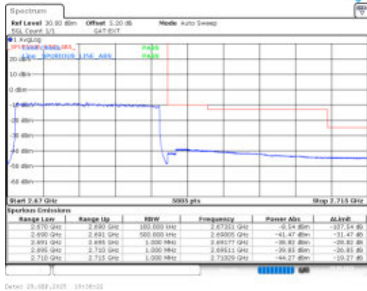
Band41-20MHz-16QAM-41490-100RB#0-PASS
