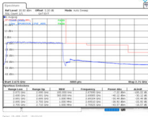
Band41-15MHz-16QAM-41515-75RB#0-PASS
