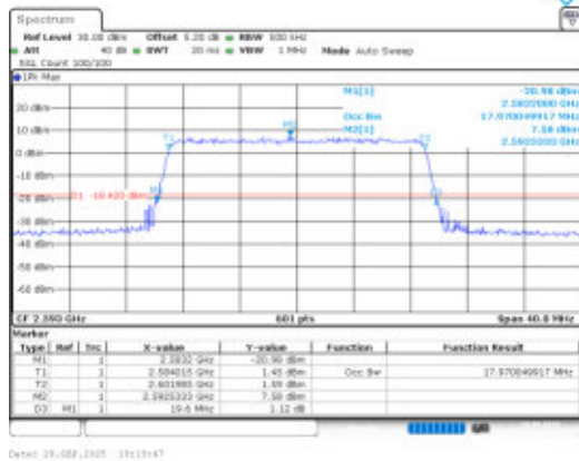
Band41-20MHz-QPSK-40620-100RB#0-PASS
