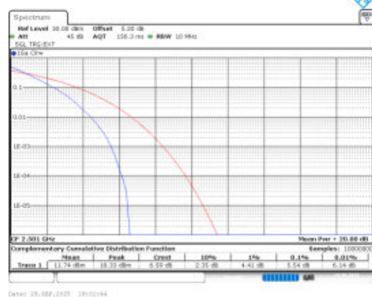
Band41-10MHz-QPSK-39700-50RB#0-PASS
