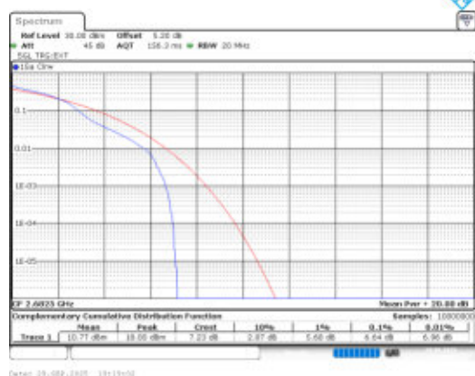
Band41-15MHz-16QAM-41515-1RB#0-PASS
