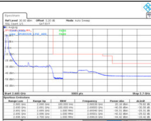
Band41-5MHz-QPSK-41565-1RB#24-PASS
