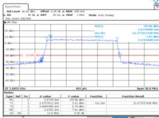
Band41-15MHz-16QAM-41515-75RB#0-PASS
