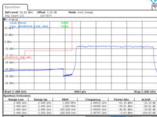
Band41-10MHz-QPSK-39700-50RB#0-PASS
