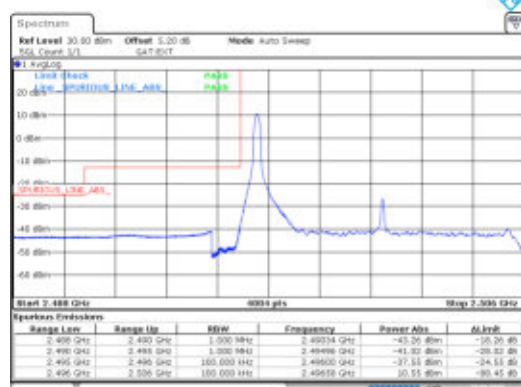
Band41-10MHz-16QAM-39700-1RB#0-PASS
