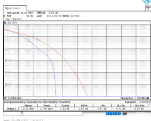
Band41-15MHz-QPSK-40620-1RB#0-PASS
