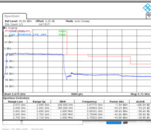
Band41-15MHz-QPSK-41515-75RB#0-PASS
