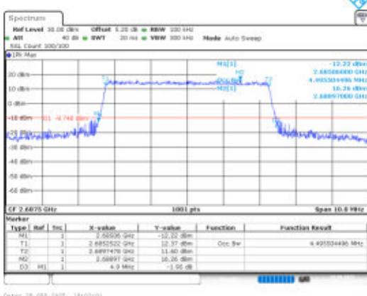
Band41-5MHz-QPSK-41565-25RB#0-PASS
