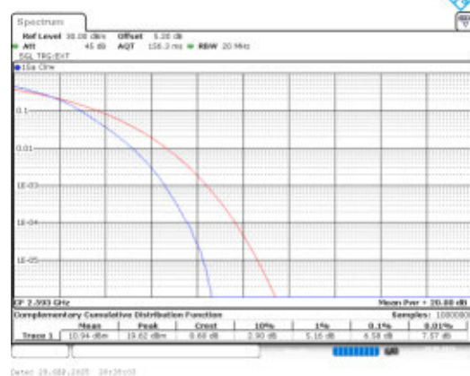
Band41-20MHz-16QAM-40620-100RB#0-PASS
