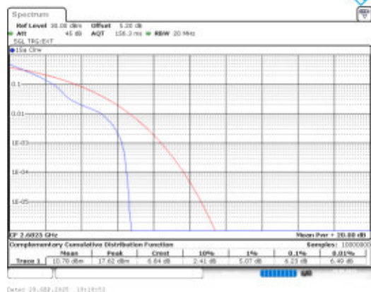
Band41-15MHz-QPSK-41515-1RB#0-PASS
