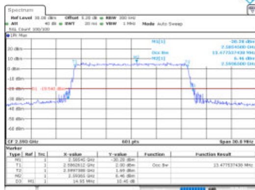
Band41-15MHz-16QAM-40620-75RB#0-PASS
