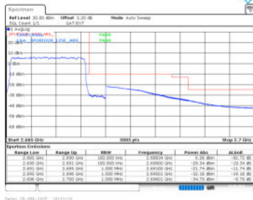
Band41-5MHz-16QAM-41565-25RB#0-PASS
