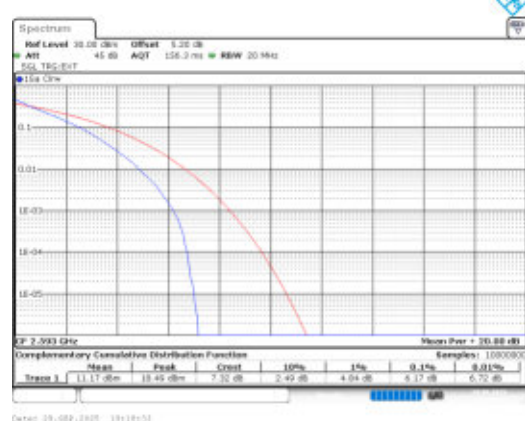
Band41-15MHz-QPSK-40620-75RB#0-PASS
