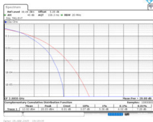
Band41-15MHz-16QAM-39725-75RB#0-PASS
