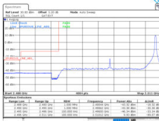
Band41-15MHz-QPSK-39725-1RB#74-PASS
