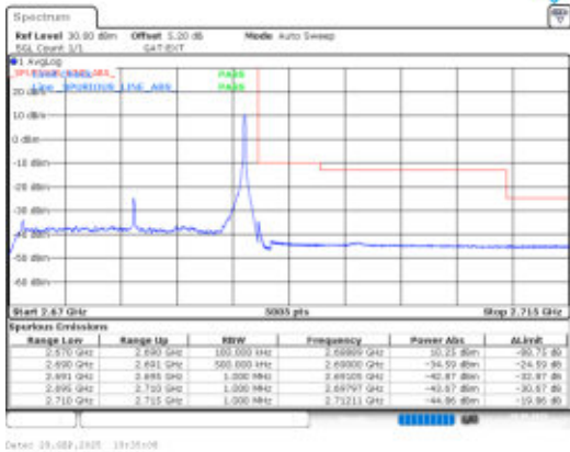
Band41-20MHz-16QAM-41490-1RB#99-PASS
