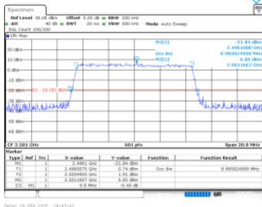
Band41-10MHz-QPSK-39700-50RB#0-PASS
