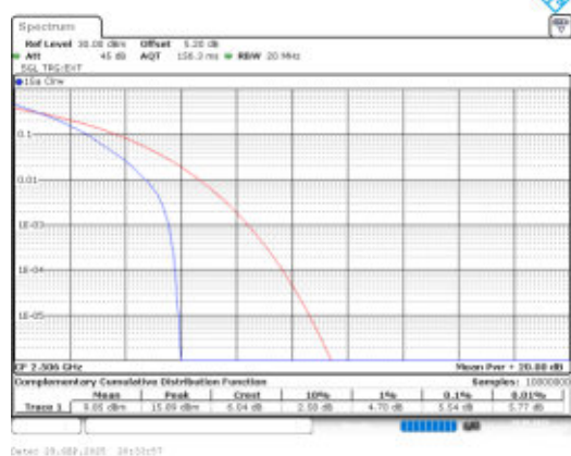
Band41-20MHz-QPSK-39750-1RB#0-PASS
