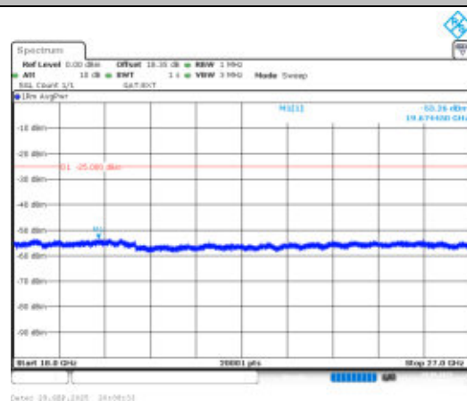
Band41-20MHz-16QAM-41490-1RB#0- 18000~27000-PASS
