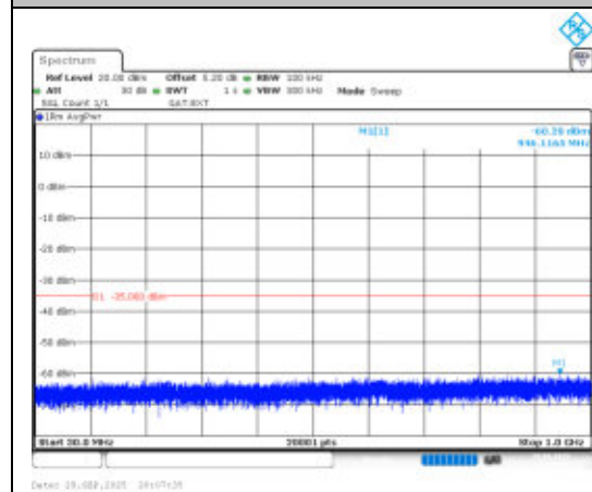
Band41-20MHz-16QAM-41490-1RB#0-30~1000- PASS
