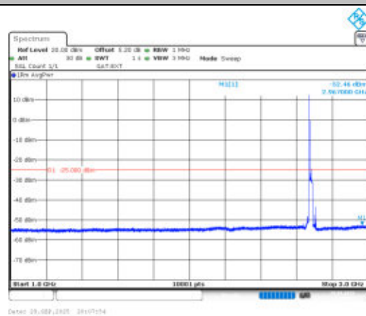
Band41-20MHz-16QAM-41490-1RB#0- 1000~3000-PASS
