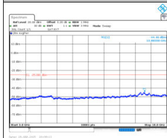
Band41-20MHz-16QAM-41490-1RB#0- 3000~18000-PASS
