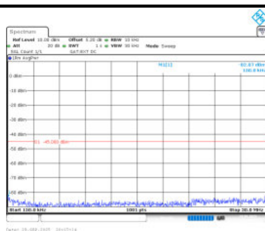
Band41-20MHz-16QAM-41490-1RB#0-0.15~30- PASS
