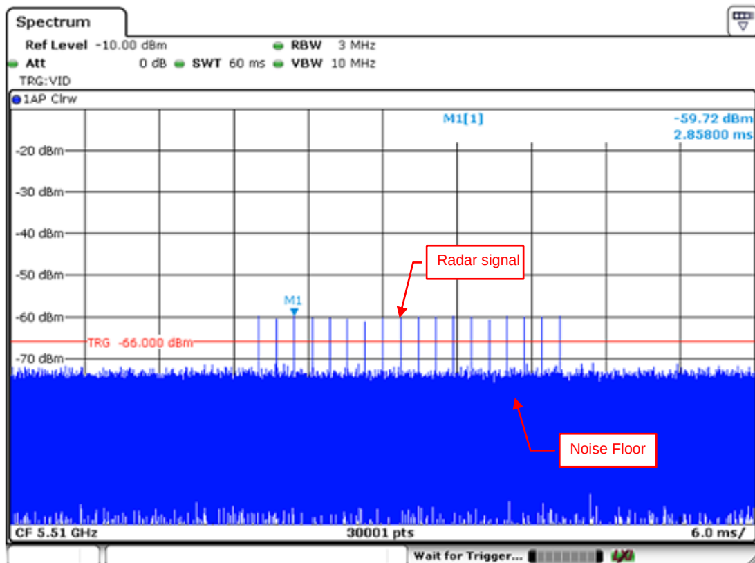
Radar Signal 0
