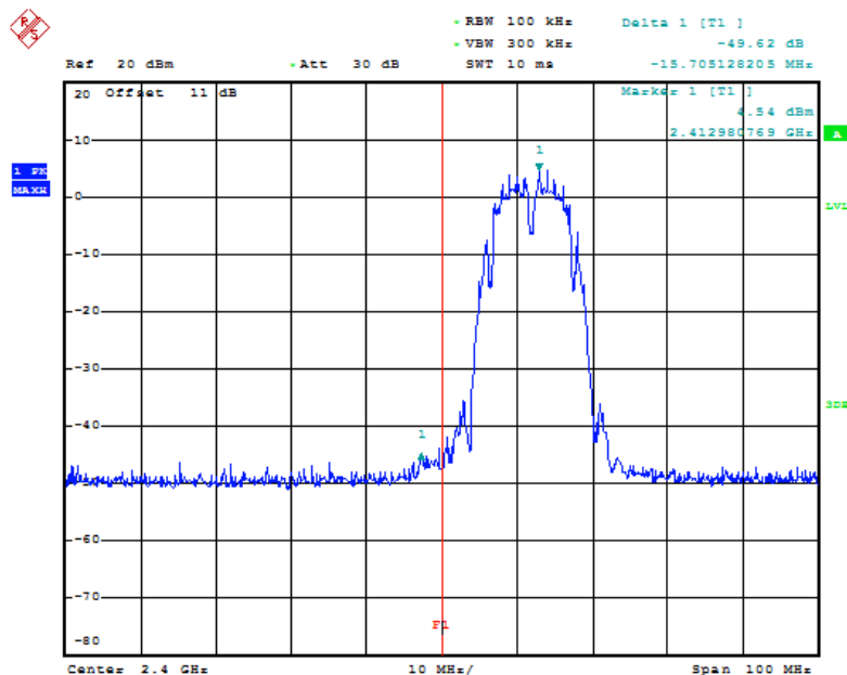
Band Edge, Left Side (B mode / CH Low)
