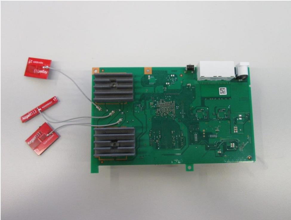
Photo A3-3: Main PCB, Bottom View with antennas
