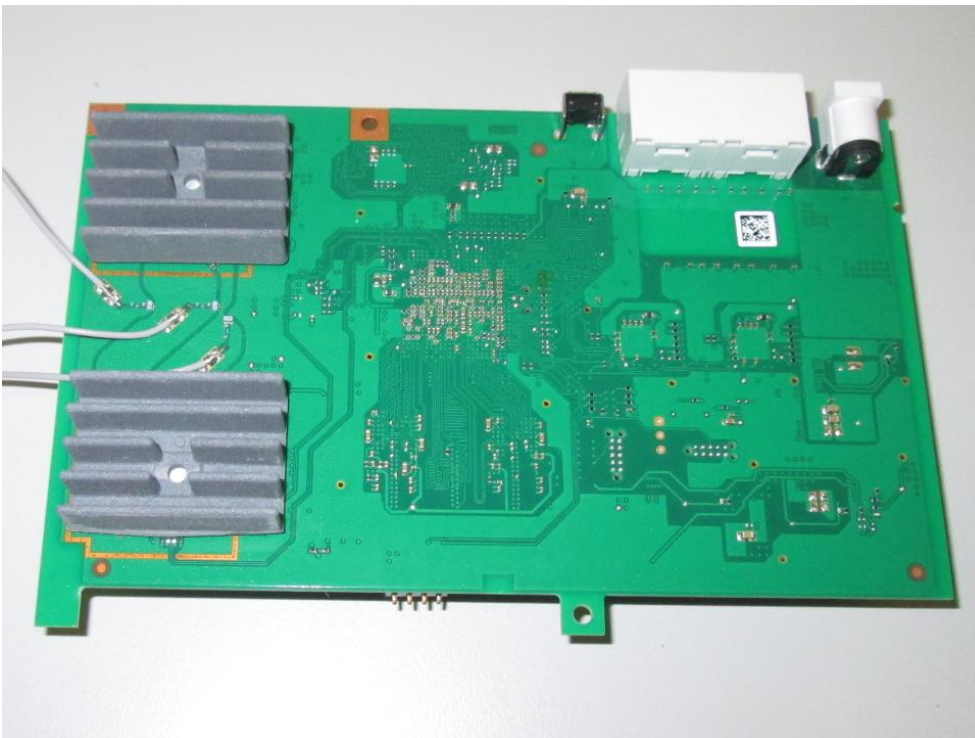
Photo A3-2: Main PCB, Bottom View
