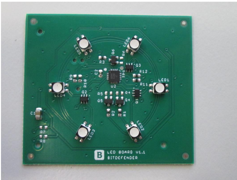
Photo A3-5: LED PCB, Top View
