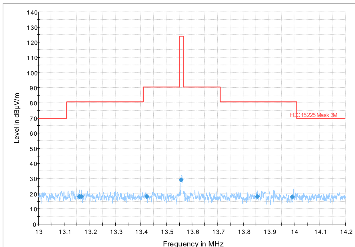
Figure 8.4-1: Radiated emissions spectral plot (13 MHz - 14.2 MHz), 0 degrees
