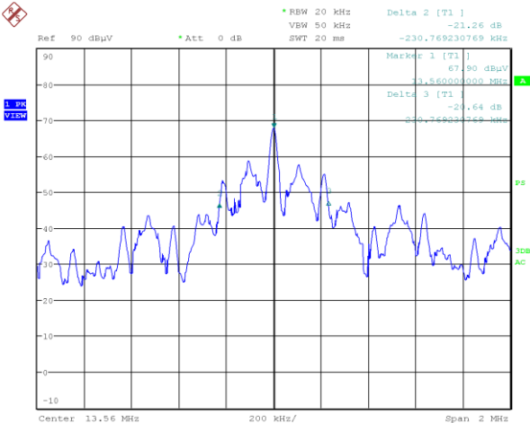
Figure 8.2-1: 20 dB occupied bandwidth, 13.56 MHz
