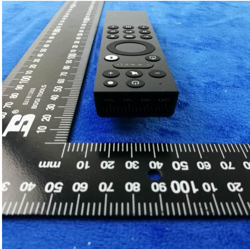
EUT - Top View
