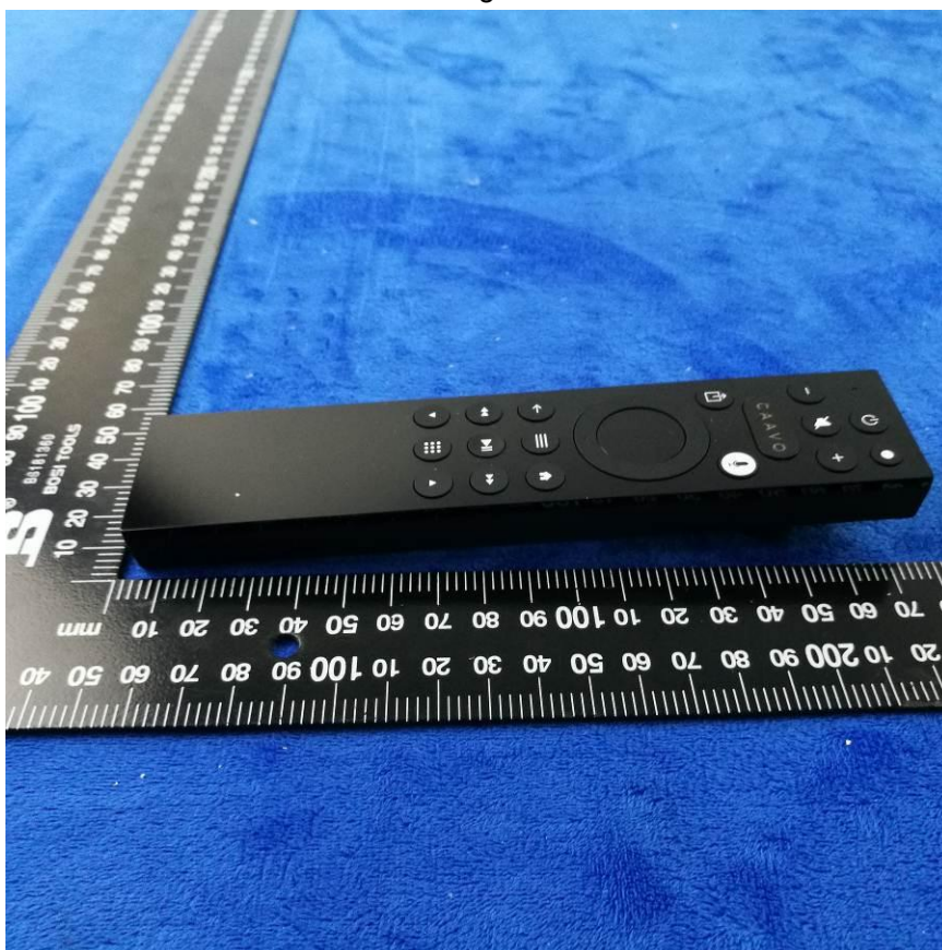
EUT - Right View
