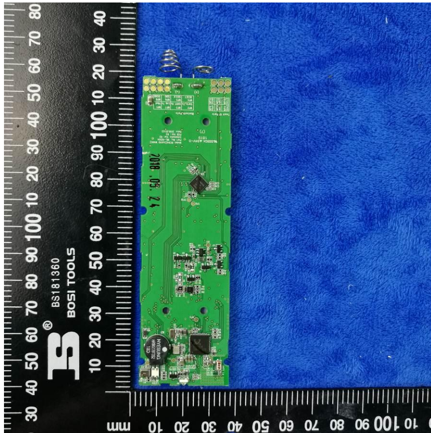
Mainboard - Front View
