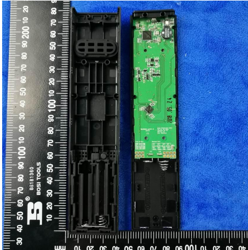
Cover Off - Top View 1
