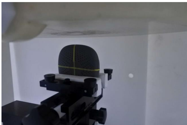
Left side, Test Separation 16 mm
