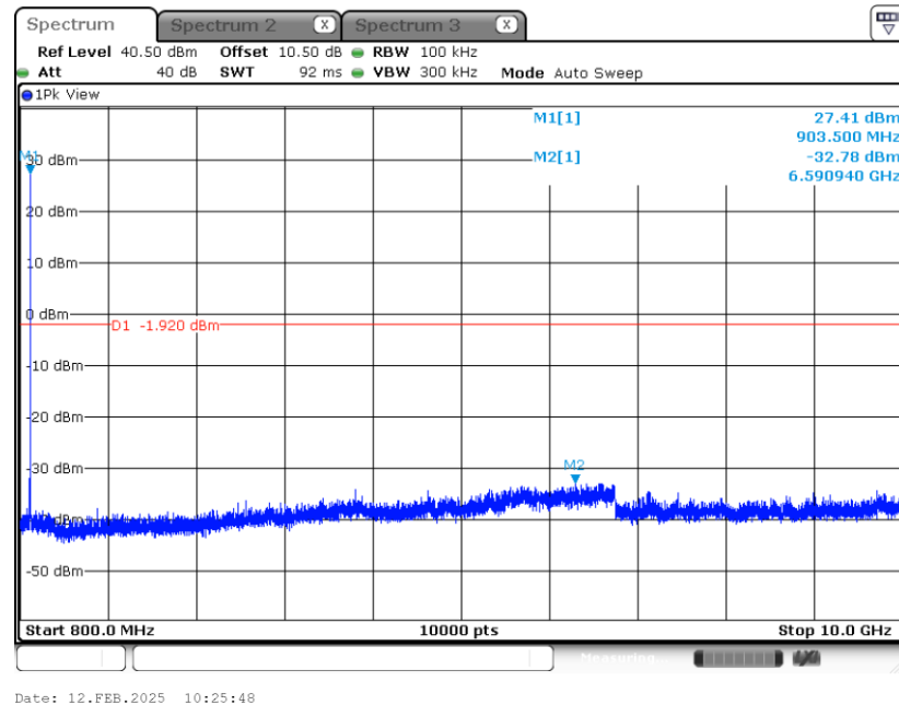
Conducted Spurious Emission Plot on 904 MHz
