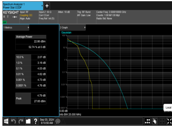
N77(20M)_DFT-s-OFDM_PI_2- BPSK_Edge_1RB_Left_Mid_CH
