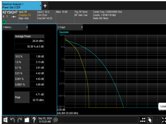
N77(20M)_DFT-s-OFDM_PI_2- BPSK_Outer_Full_Mid_CH
