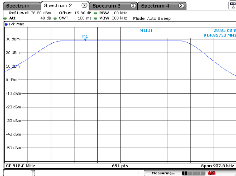
PSD 100kHz Plot on 915 MHz
