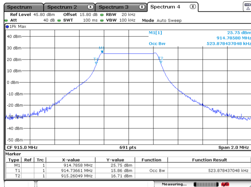
99% Occupied Bandwidth Plot on 915 MHz
