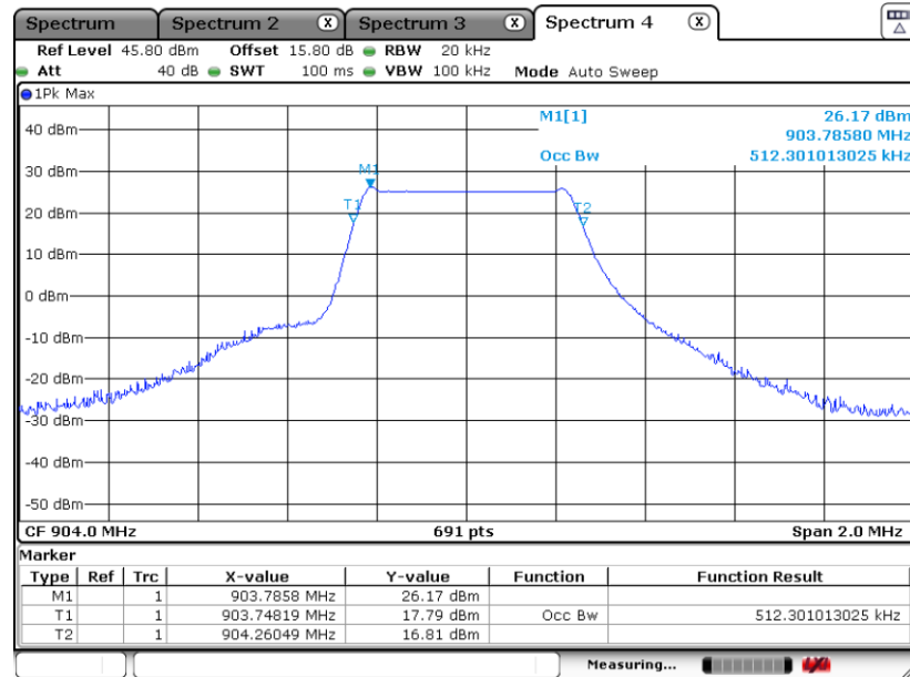
99% Occupied Bandwidth Plot on 904 MHz
