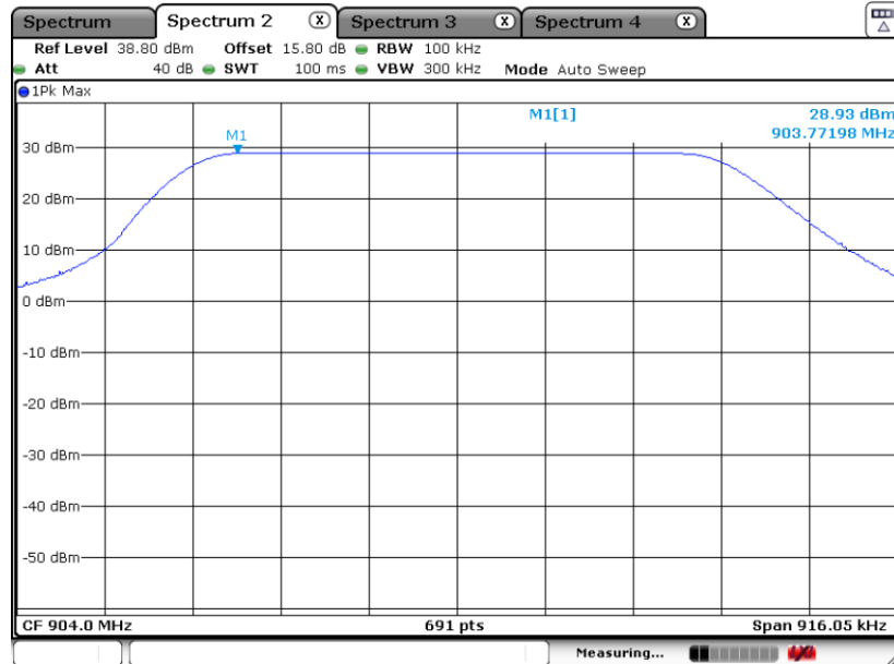
PSD 100kHz Plot on 904 MHz
