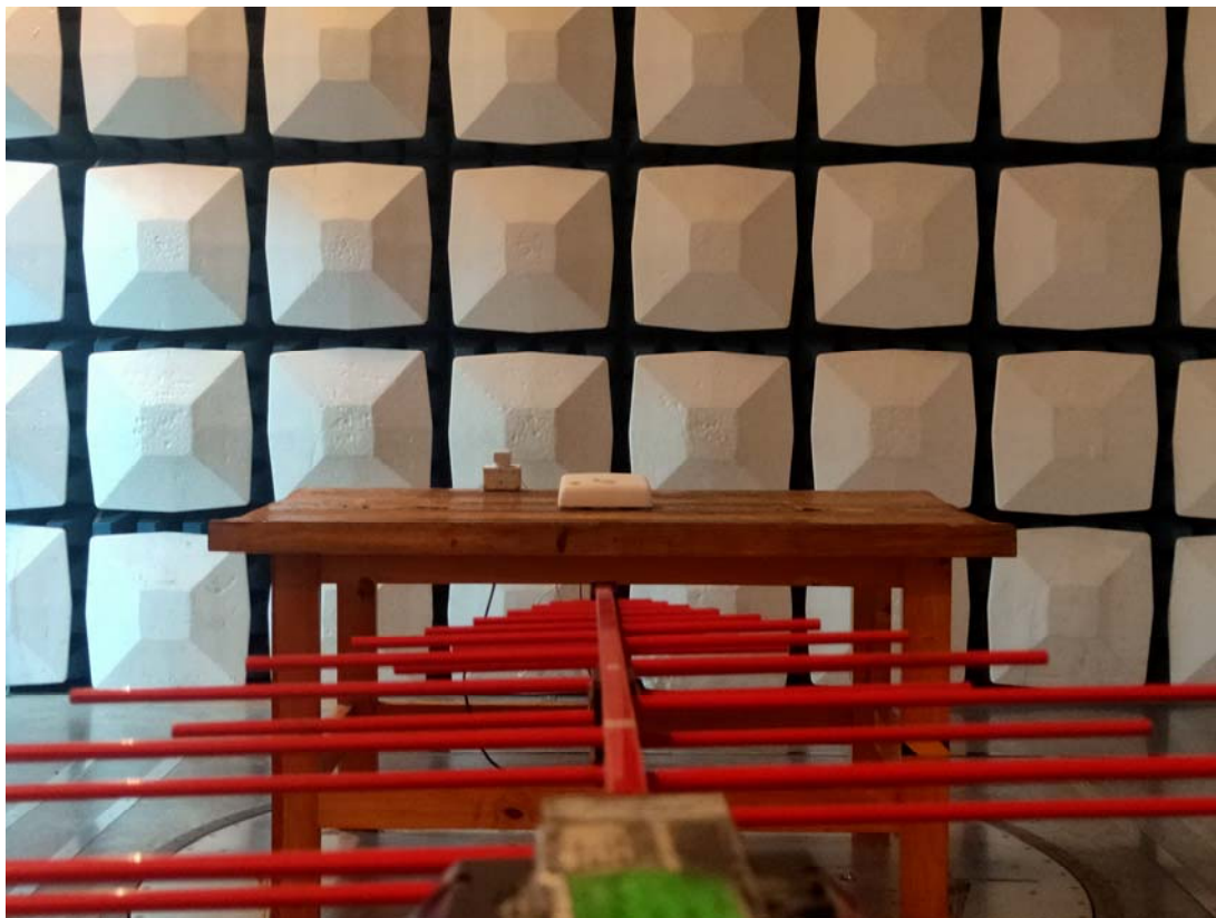
Radiated Emission Below 1GHz View-USB Adapter Mode
