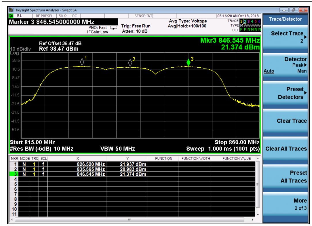
(Plot I, HSUPA 850 MHz, Channel = 4132, 4182, 4233)
