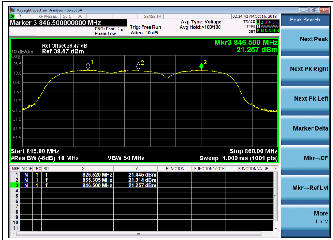
(Plot G, WCDMA 850 MHz, Channel = 4132, 4182, 4233)
