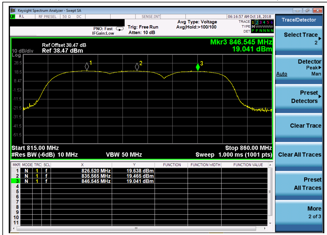
(Plot H, HSDPA 850 MHz, Channel = 4132, 4182, 4233)
