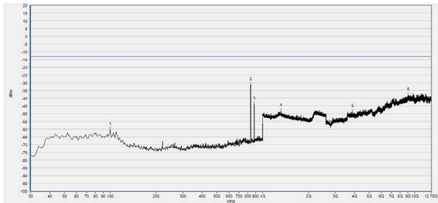
(Plot E3, WCDMA 850MHz, Channel = 4182, Horizontal)
