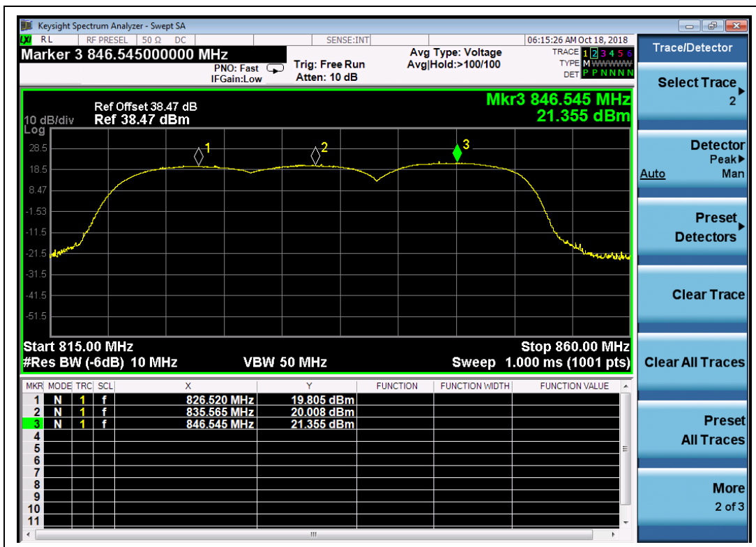
(Plot J, HSPA+ 850 MHz, Channel = 4132, 4182, 4233)
