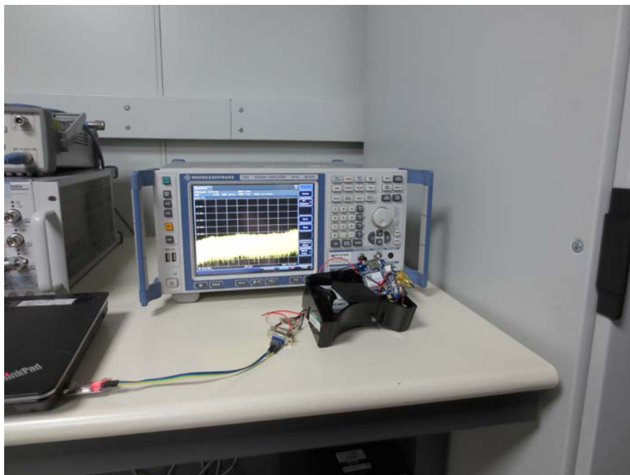
RF Conducted Emissions Test setup
