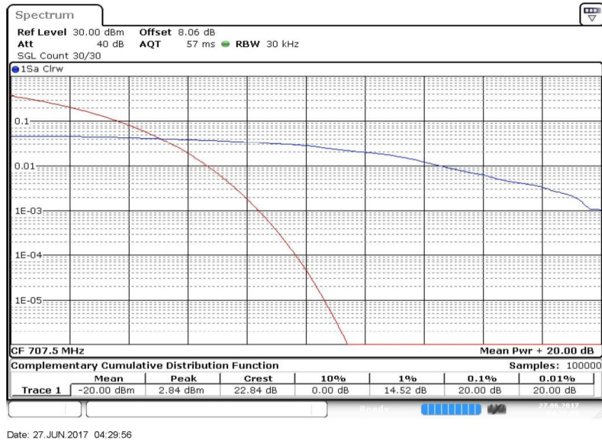
Peak-Average Ratio Plot(1.4MHz BW,QPSK,Band 12-mid Channel)
