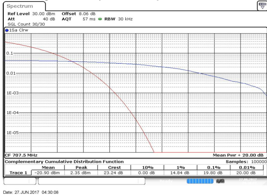
Peak-Average Ratio Plot(1.4MHz BW,16QAM,Band 12-mid Channel)
