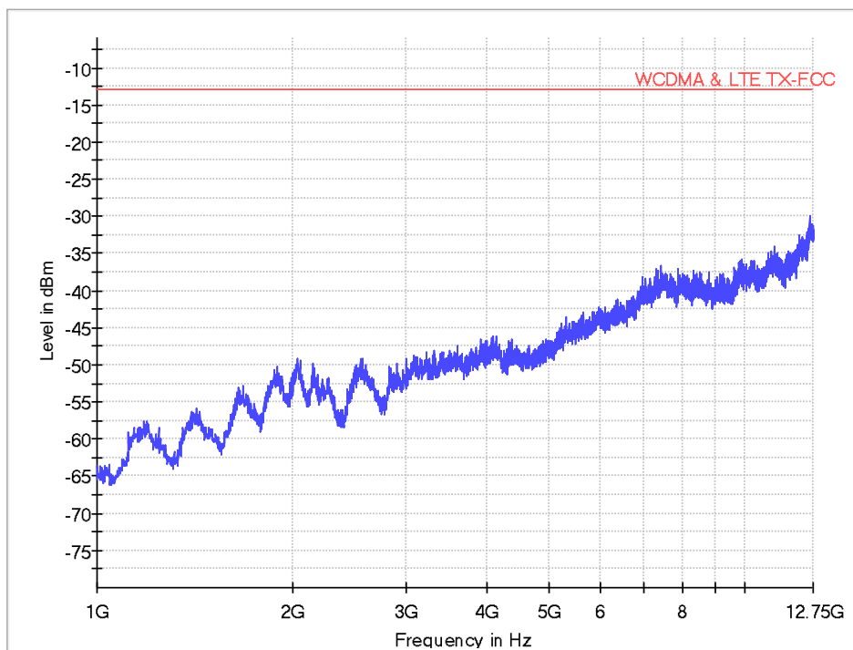
FCC 234G TX 1-12.75G dBm
