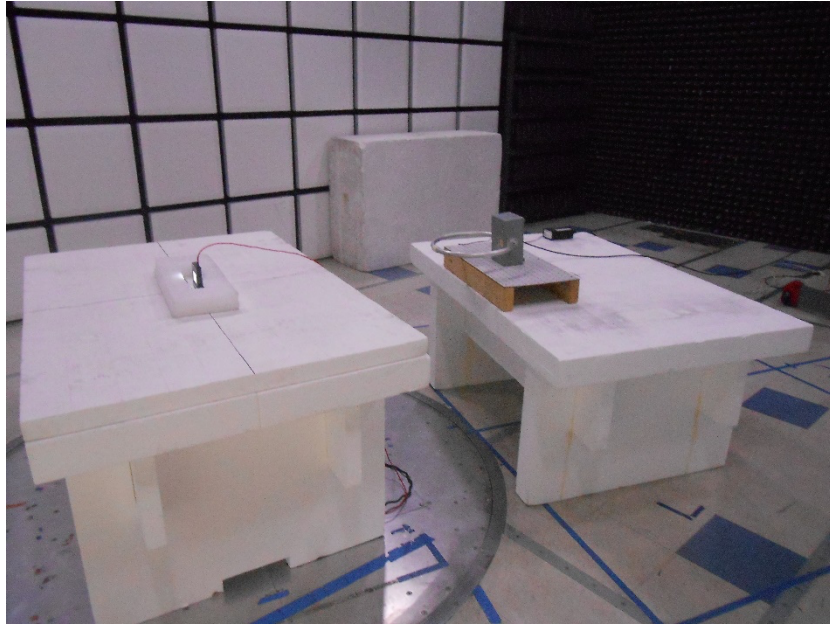
Radiated Emissions below 30 MHz
