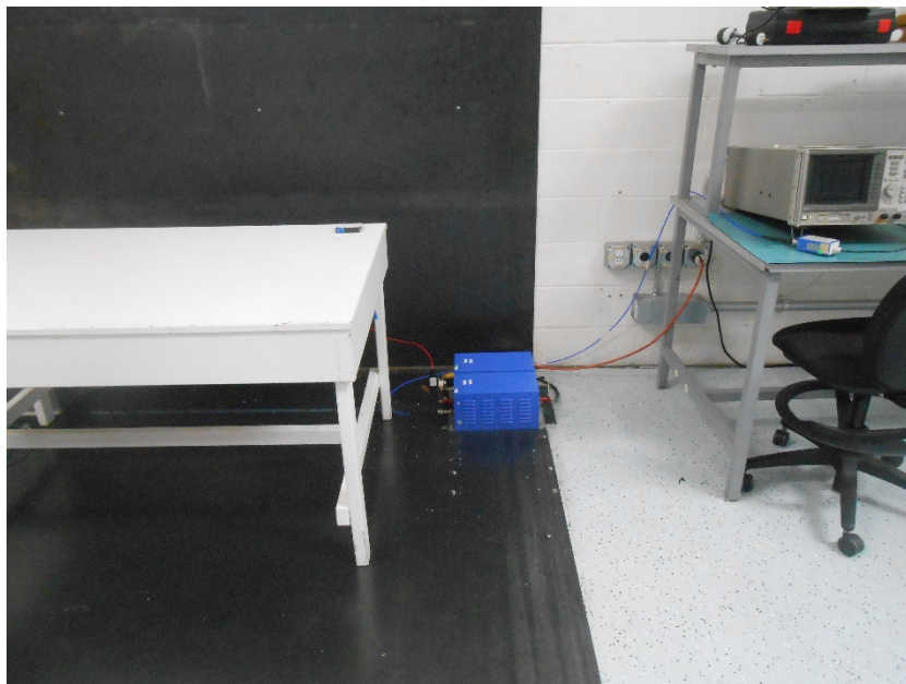
AC Conducted Emissions
