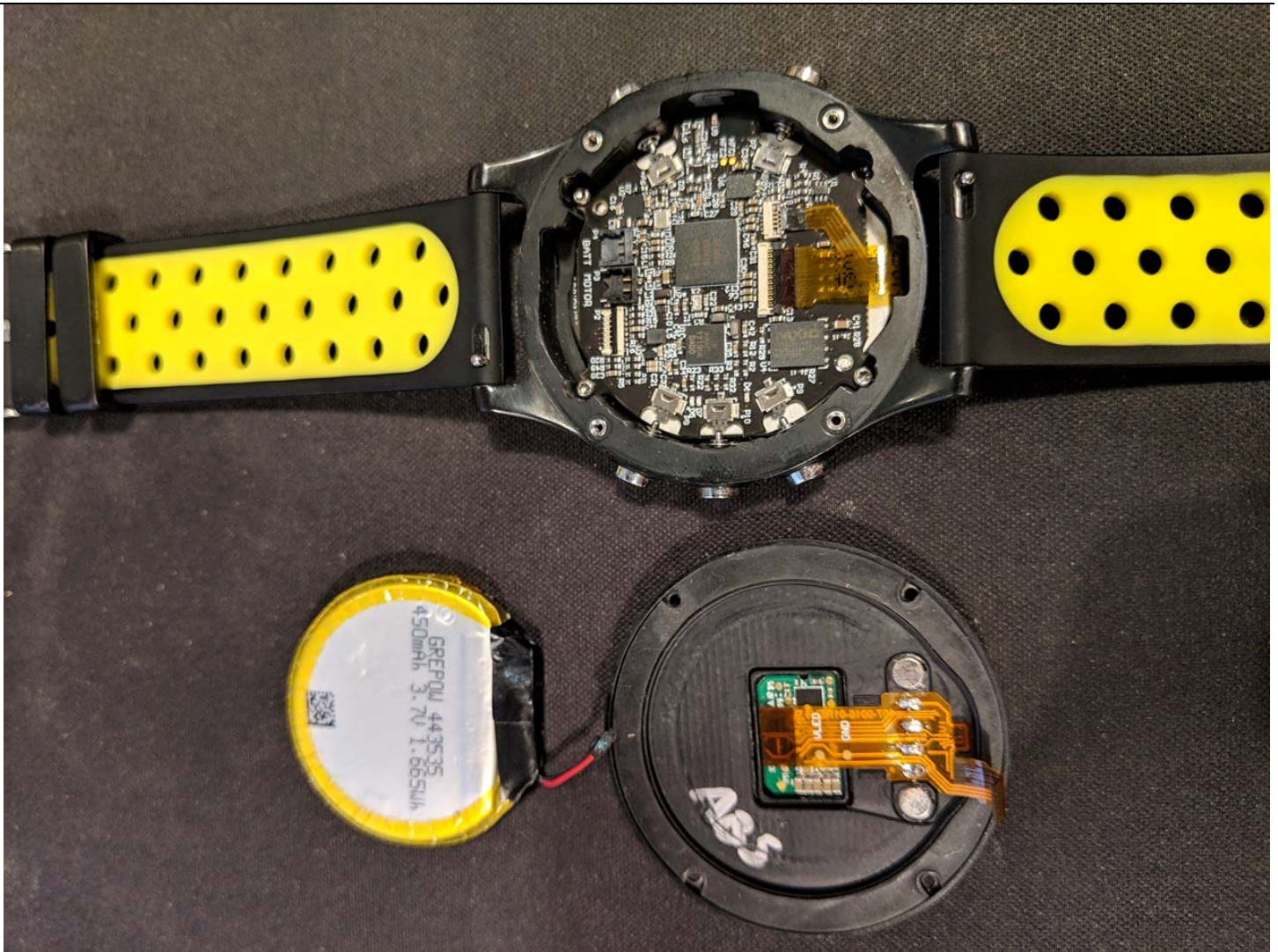
Disassembly Overview
