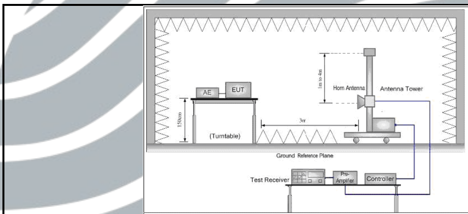
Figure 3. Above 1GHz
