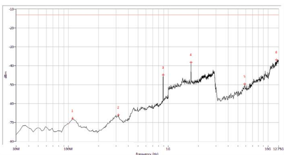
(Plot C.4: WCDMA 850MHz Channel = 4175, Test Antenna Vertical)
