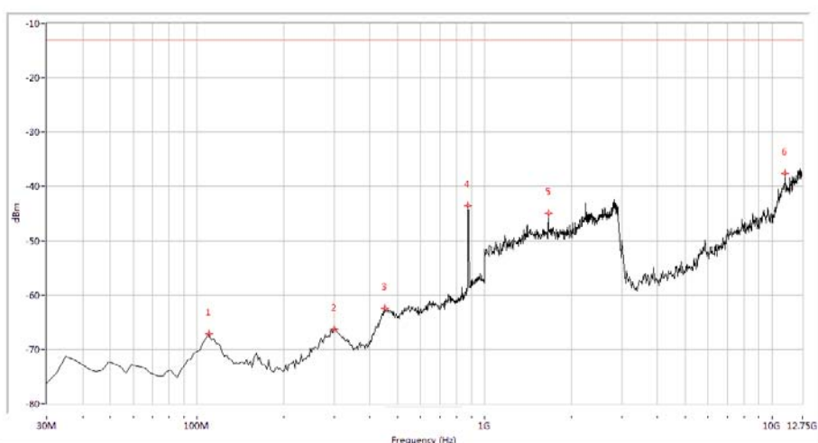
(Plot C.2: WCDMA 850MHz Channel = 4132, Test Antenna Vertical)
