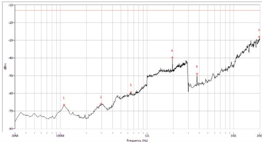
(Plot D.2: WCDMA 1900MHz Channel = 9262, Test Antenna Vertical)
