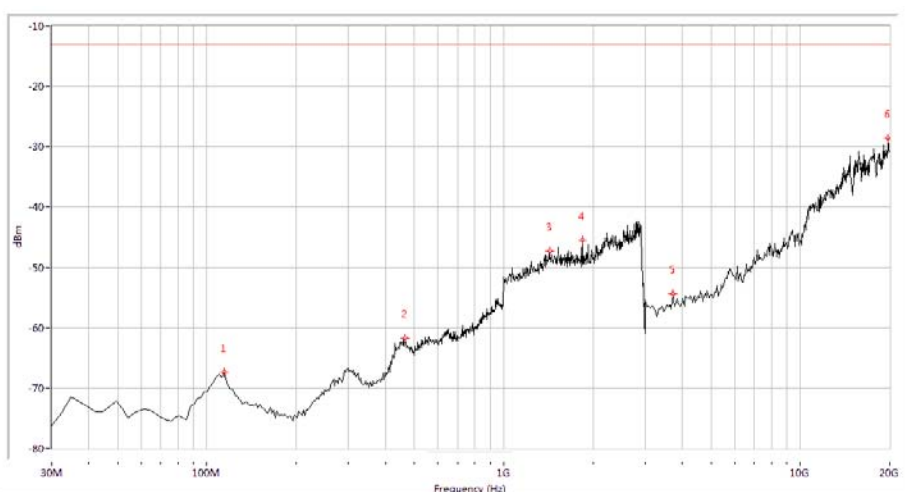
(Plot C.6: WCDMA 850MHz Channel = 4233, Test Antenna Vertical)
