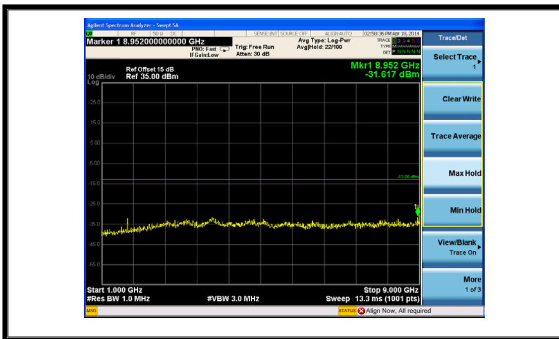
(Plot C 2.1: WCDMA850MHz Channel = 4175, 1GHz to 9GHz)
