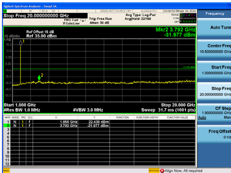
(Plot D1.1: WCDMA1900MHz Channel = 9262, 1GHz to 20GHz)
