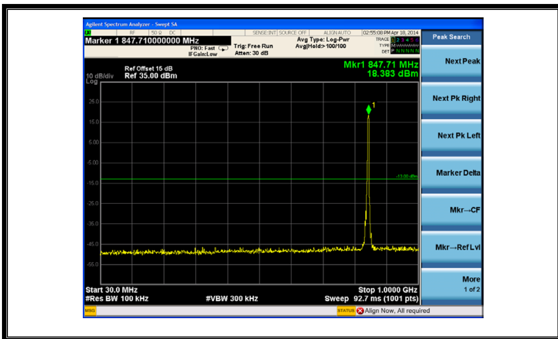
(Plot C3: WCDMA850MHz Channel = 4233, 30MHz to 1GHz)
