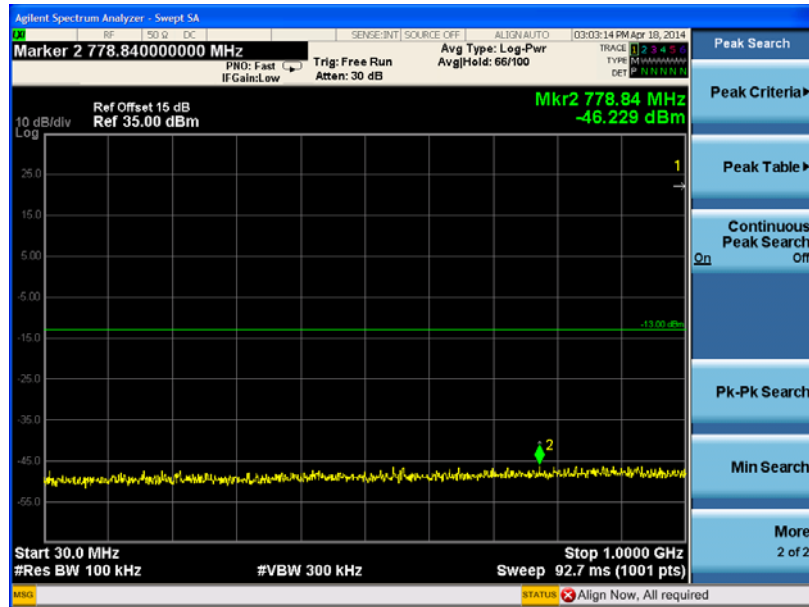
(Plot D3: WCDMA1900MHz Channel = 9538, 30MHz to 1GHz)
