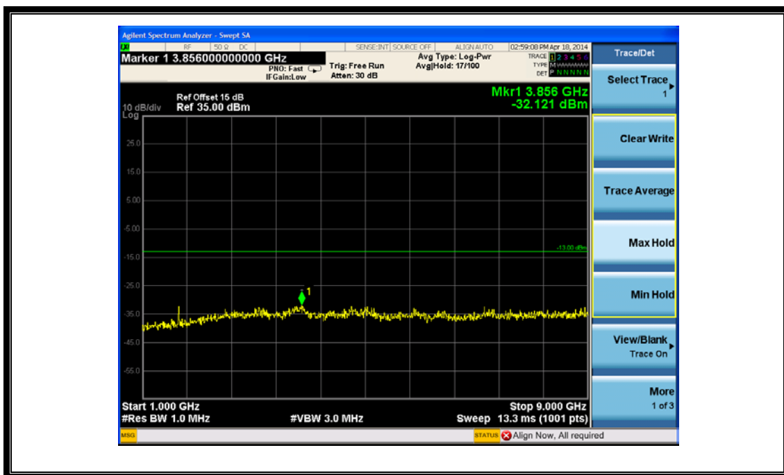
(Plot C1.1: WCDMA850MHz Channel = 4132, 1GHz to 9GHz)
