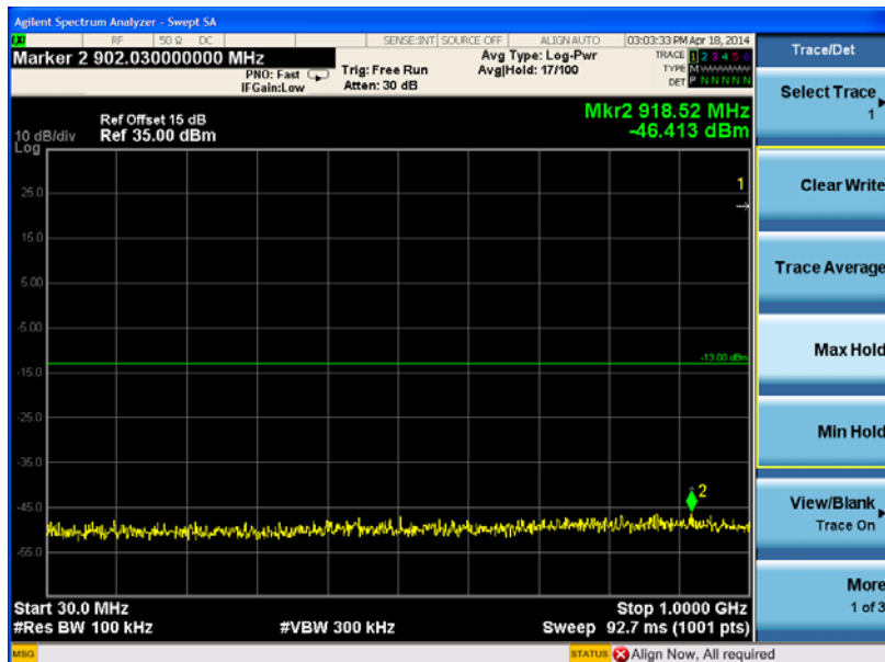
(Plot D2: WCDMA1900MHz Channel = 9400, 30MHz to 1GHz)
