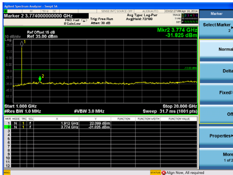
(Plot D3.1: WCDMA1900MHz Channel = 9538 1GHz to 20GHz)
