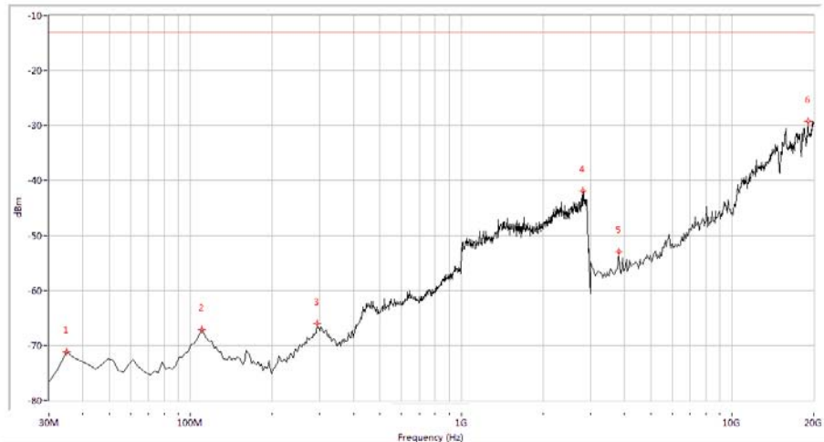
(Plot D.4: WCDMA 1900MHz Channel = 9400, Test Antenna Vertical)
