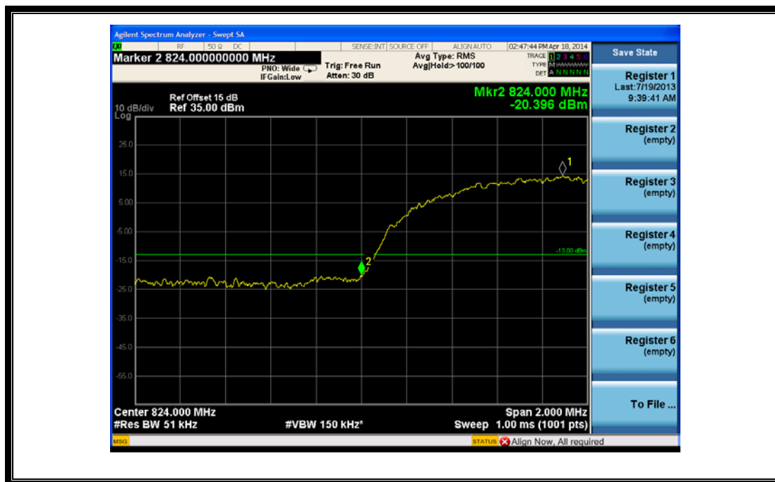
(Plot E: WCDMA 850 Channel = 4132)
