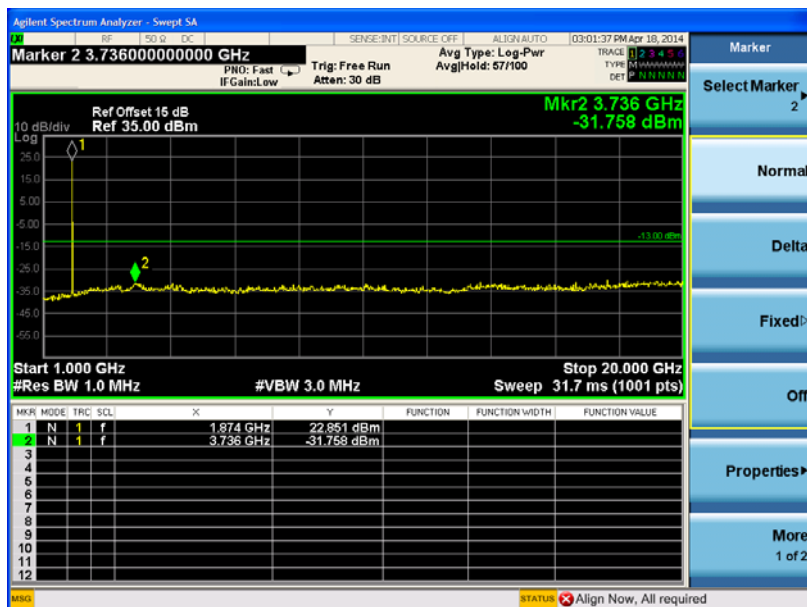
(Plot D2.1: WCDMA1900MHz Channel = 9400, 1GHz to 20GHz)
