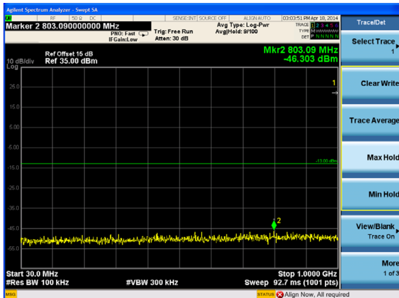
(Plot D1: WCDMA1900MHz Channel = 9262, 30MHz to 1GHz)
