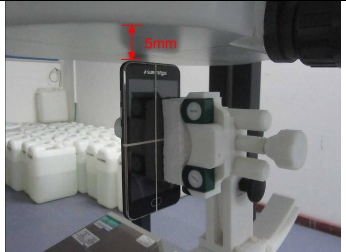
Top Side (Separation distance of 5mm)
