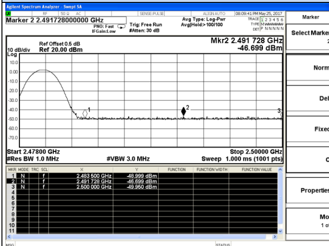
Channel 78 / 2480 MHz – Peak
