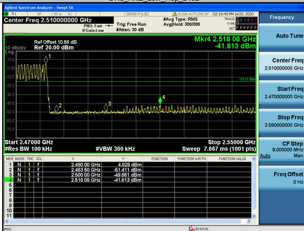
DH5_Ant1_High_Hop_2480
