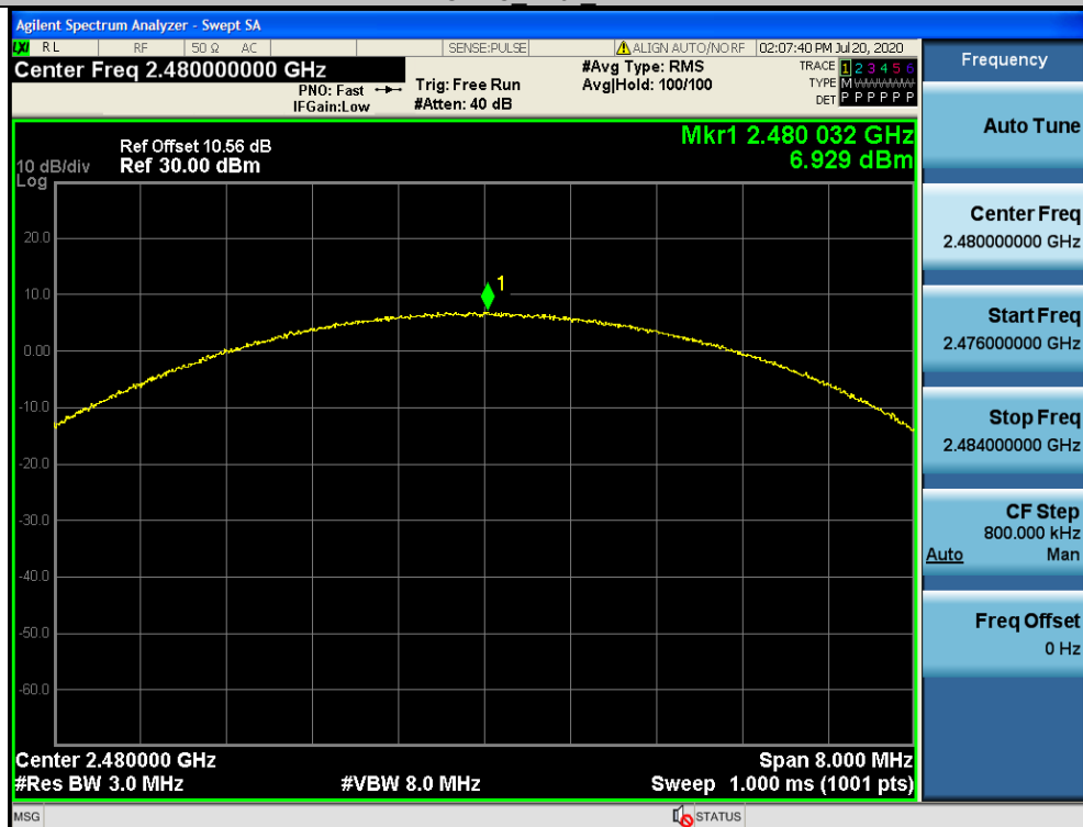
3DH5_Ant1_2480
