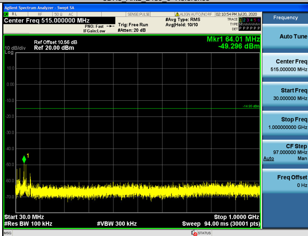
3DH5_Ant1_2480_30~1000
