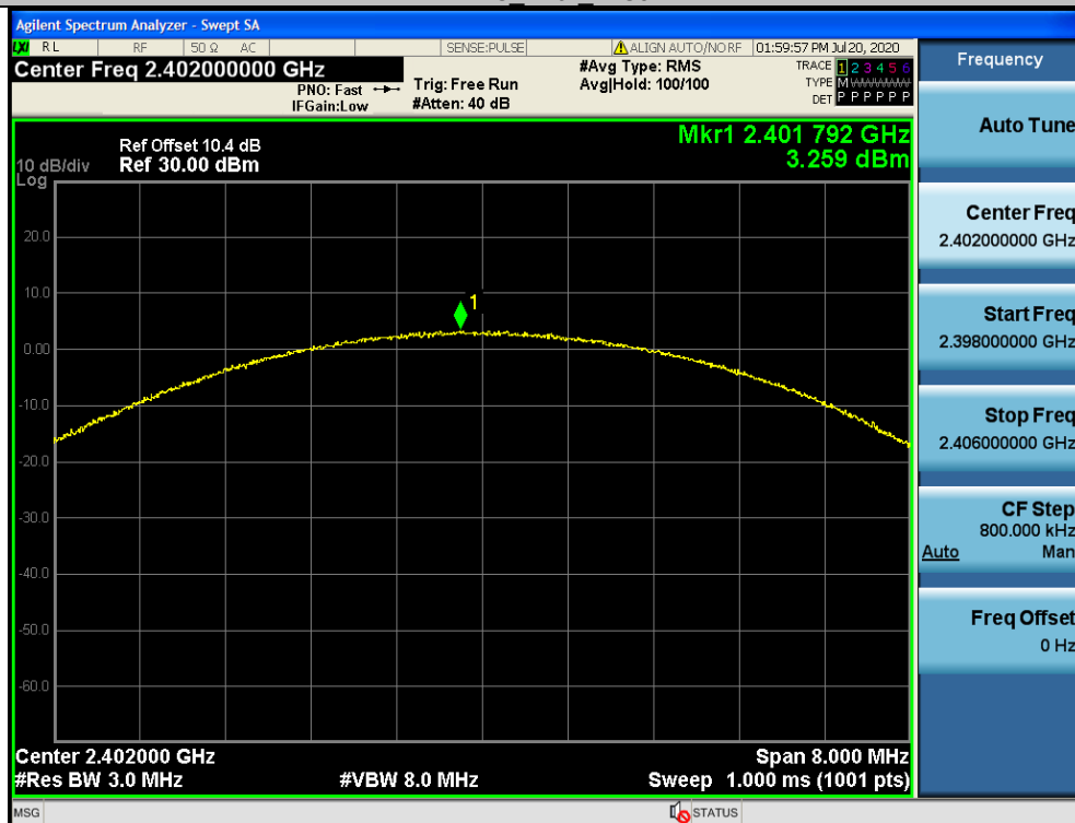
3DH5_Ant1_2402
