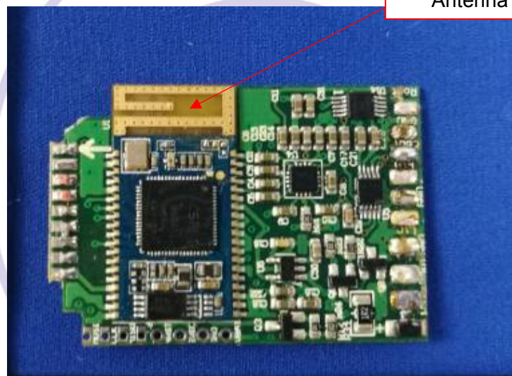
BT Antenna
