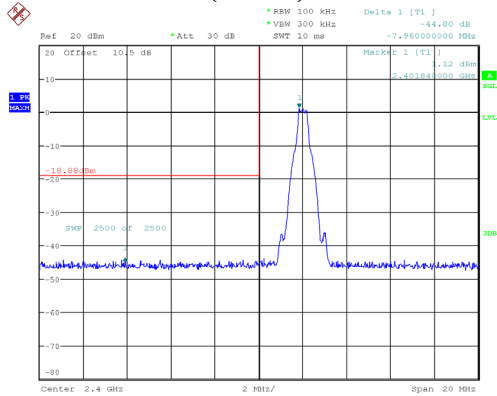
BDR (GFSK): Left Side
