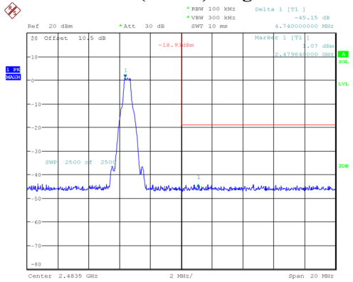
BDR (GFSK): Right Side
