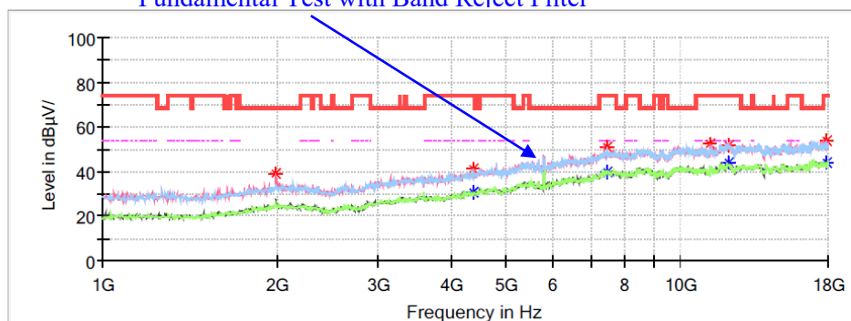
Full Spectrum Fundamental Test with Band Reject Filter
