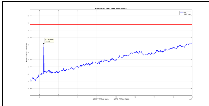
Plot 13. Peak Radiated Spurious Emissions, 1 – 18 GHz, BW 20M, Ch. 2412 M, G mode
