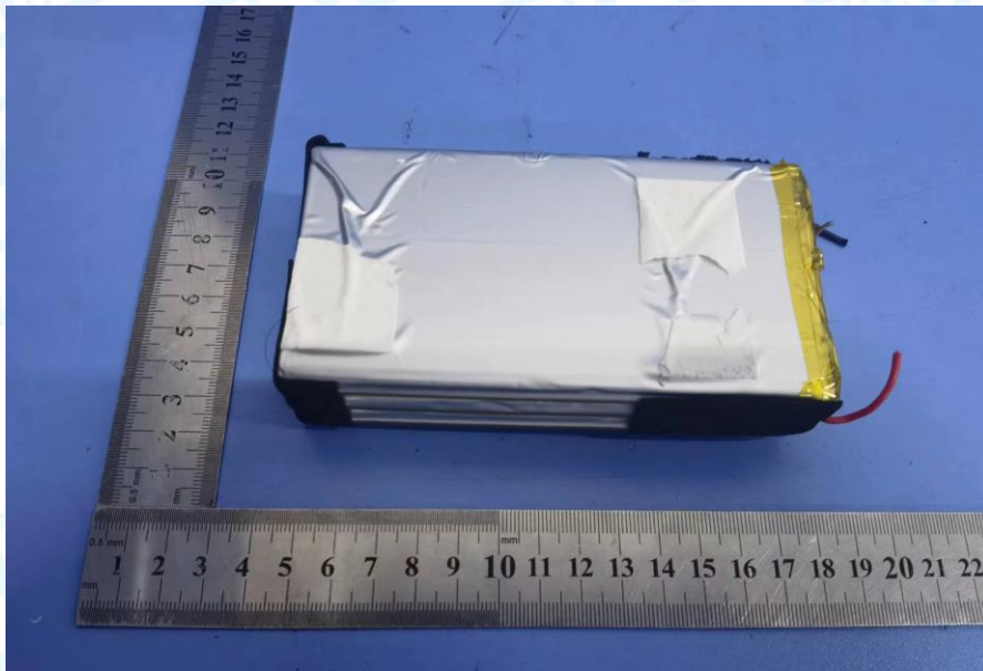
Photo 12 Appearance of Battery
