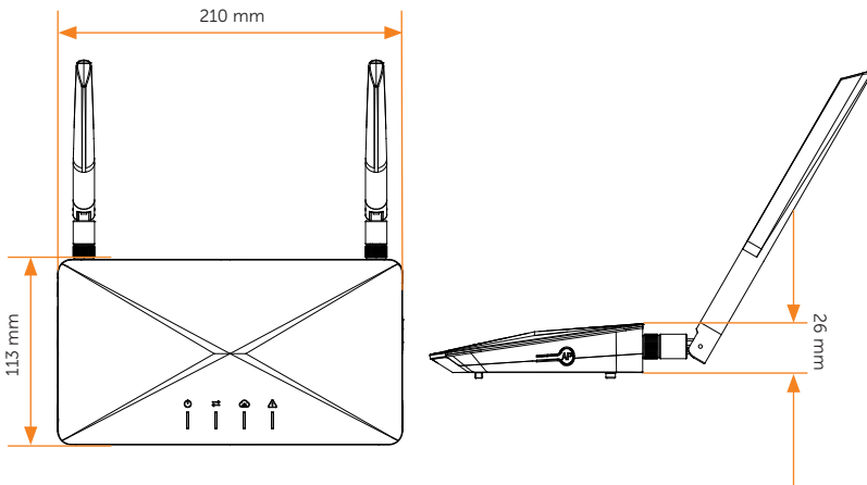
Figure 2-3 Dimensions
