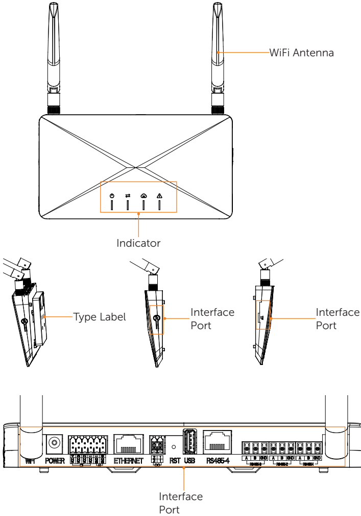
Figure 2-2 Appearance
