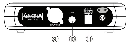
REAR PANEL
