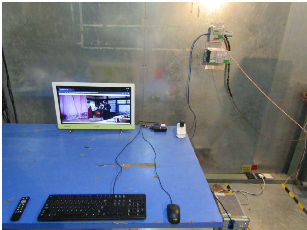
Conducted Measurement Photos(RJ45 Port)
