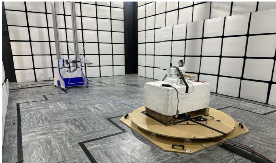
Figure 41 - Radiated Spurious Emissions Setup: 30 MHz to 1 GHz
