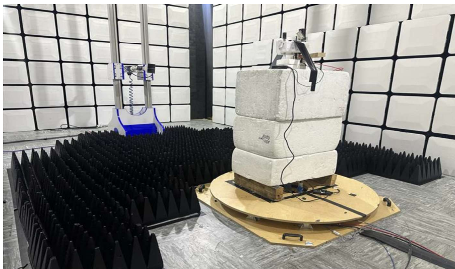
Figure 42 - Radiated Spurious Emissions Setup: 1 GHz to 18 GHz
