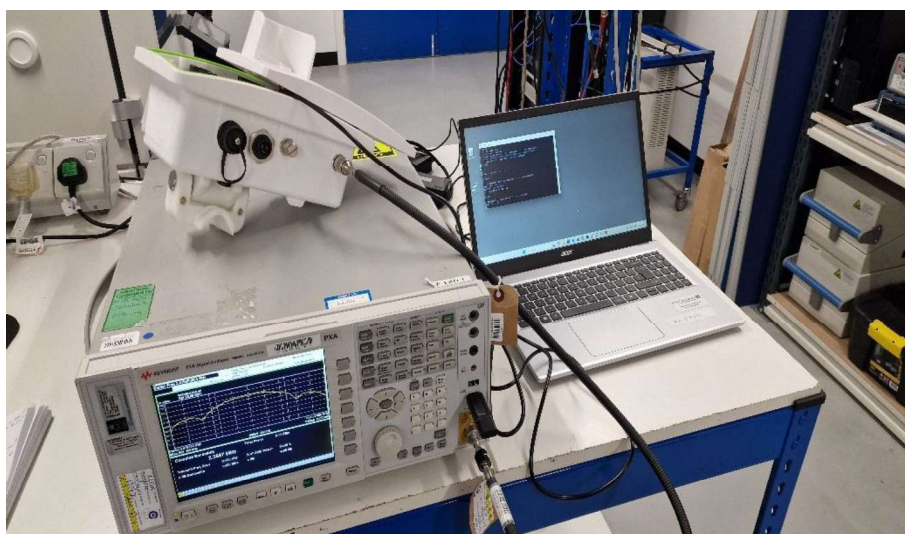
Figure 44 - Conducted Test Setup
