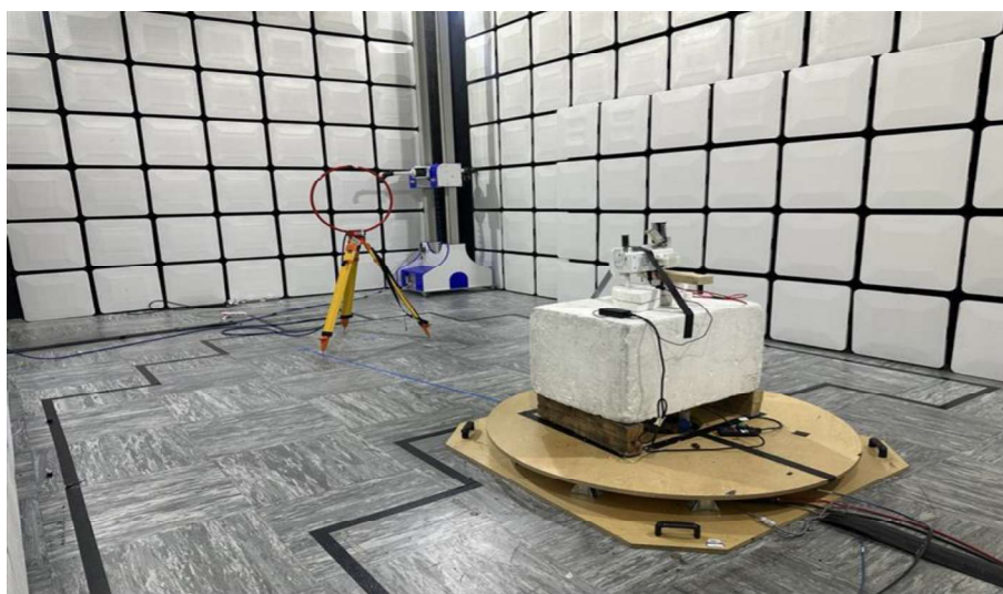
Figure 40 - Radiated Spurious Emissions Setup: 9 kHz to 30 MHz
