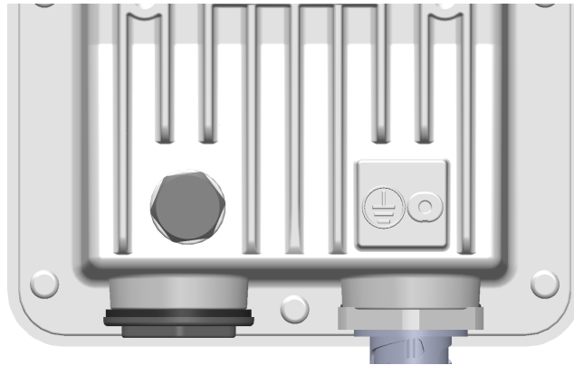
Figure 2.4: Earthing point
